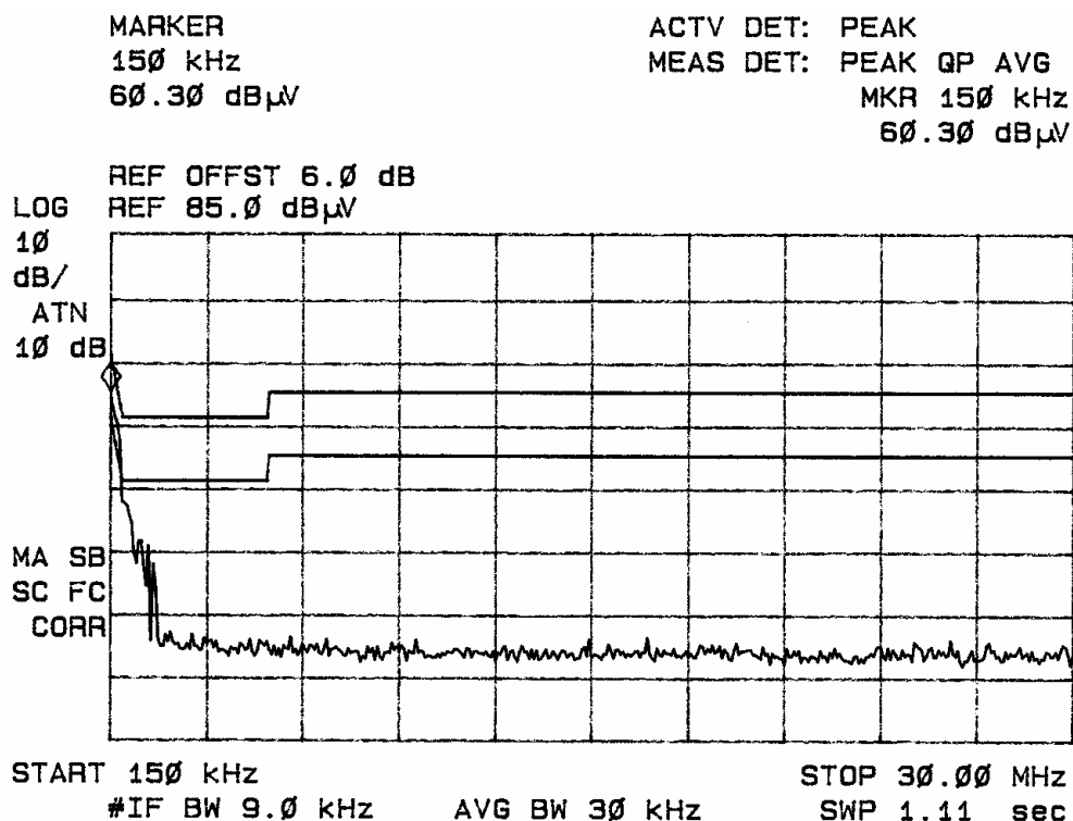
Figure two, AC power line conducted emissions Line L2.
