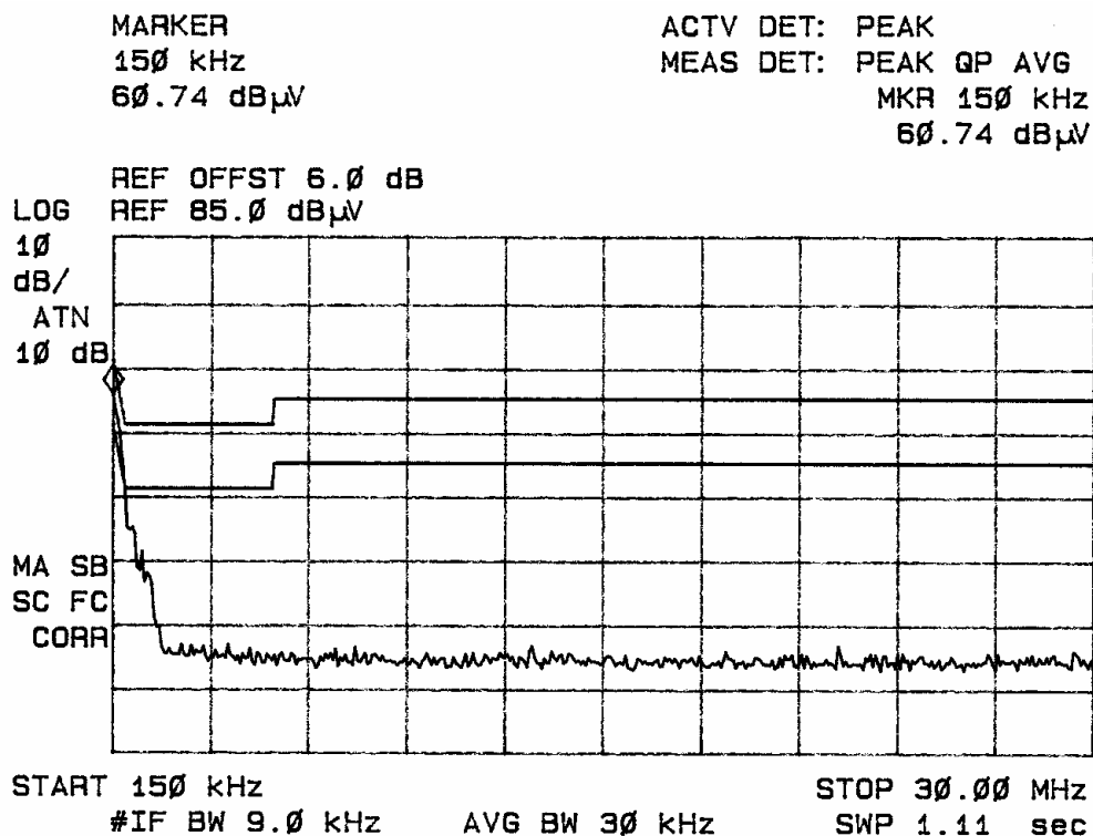
Figure one, AC power line conducted emissions Line L1.
