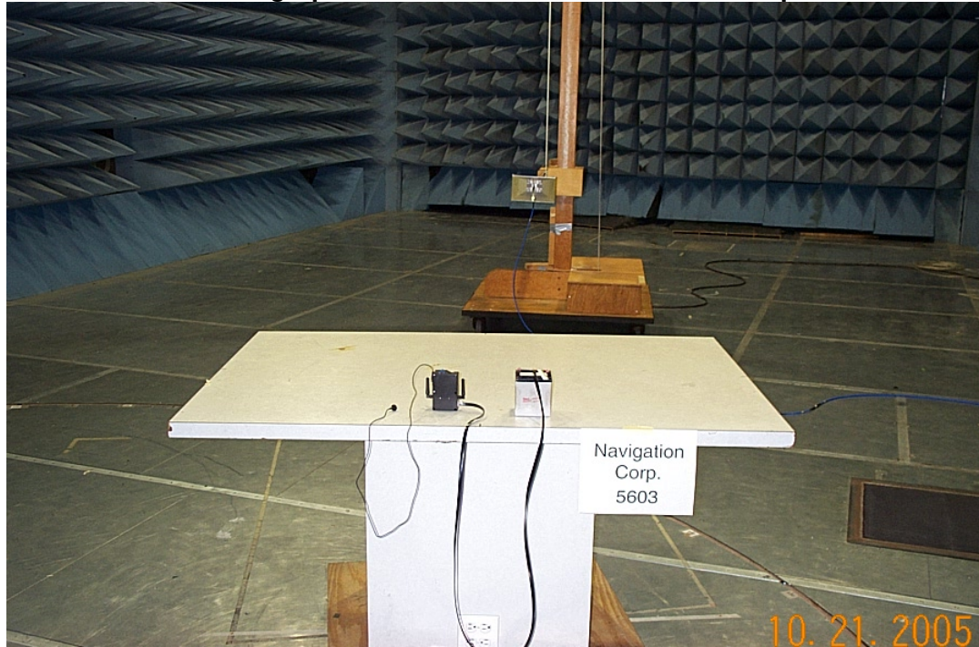
Photographs of Radiated Emissions Test Setup
