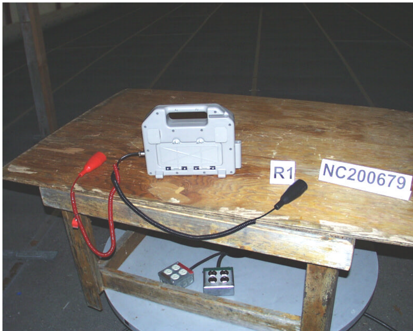
Radiated Emissions (Electric Field) Test Setup
