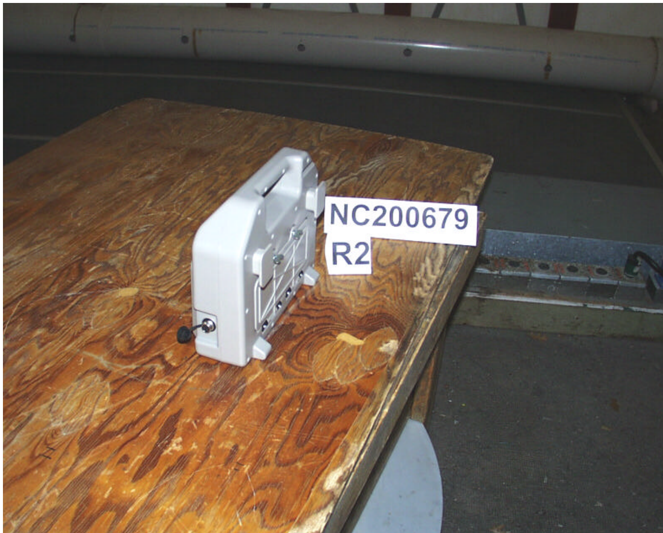
Radiated Emissions (Magnetic Field) Test Setup
