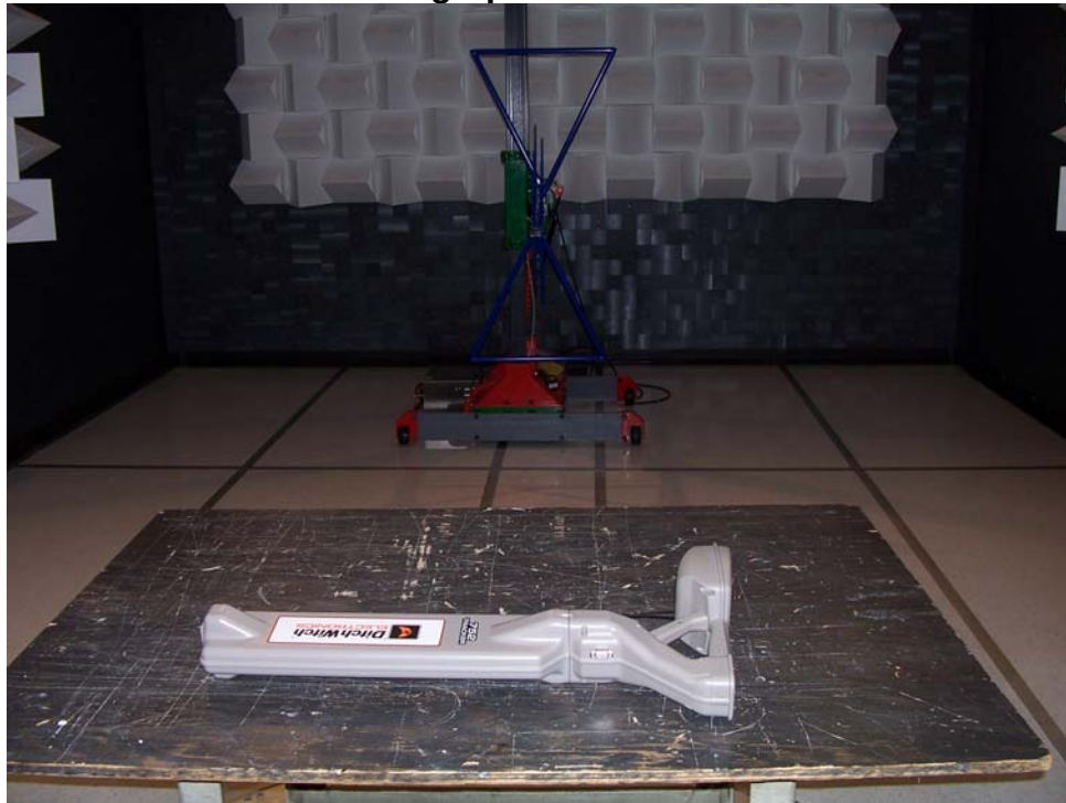
Test Photographs - Test #REHE-01
