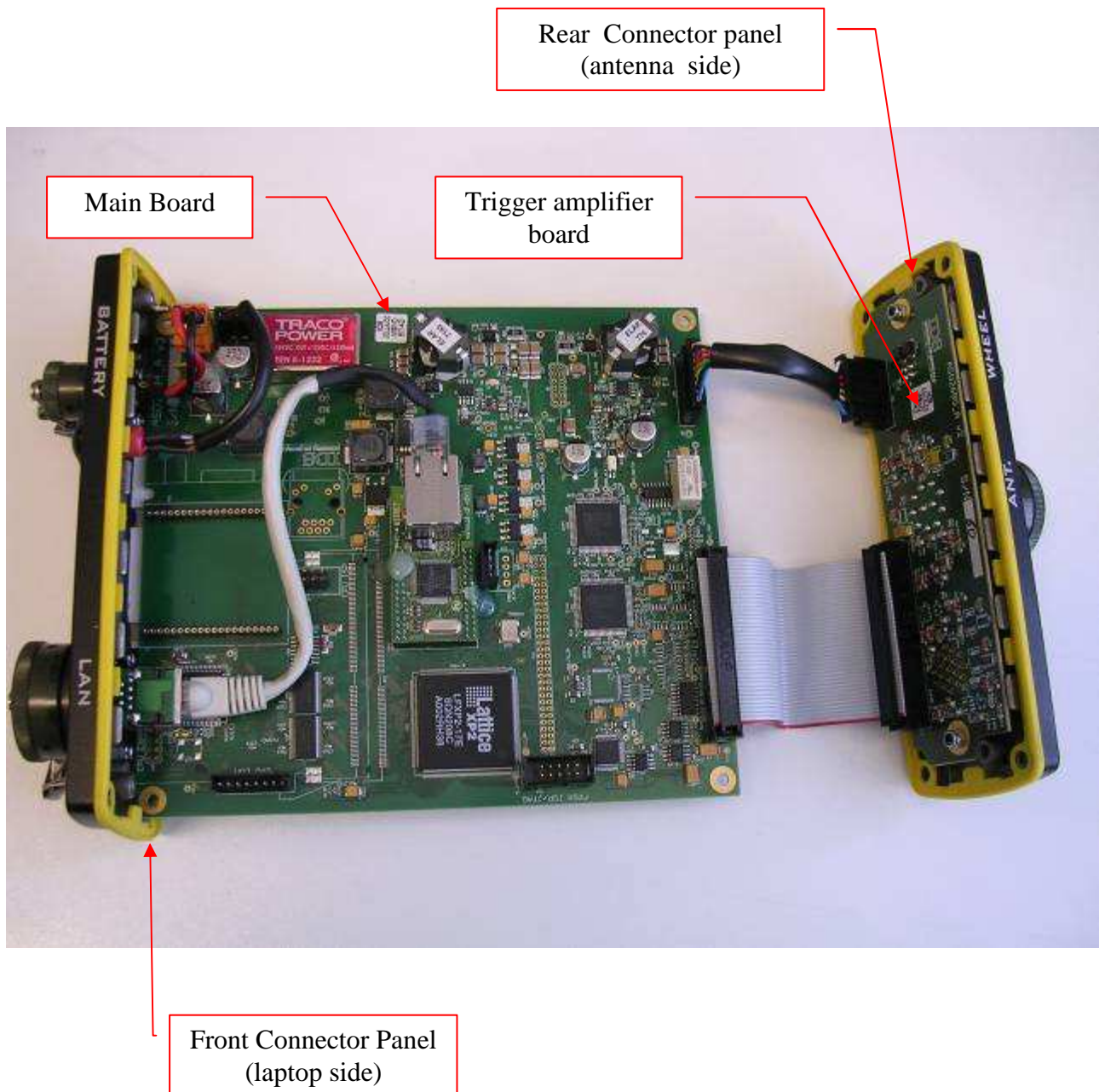
Fig. 1: DAD internal pictures showing the main board and connector panels
