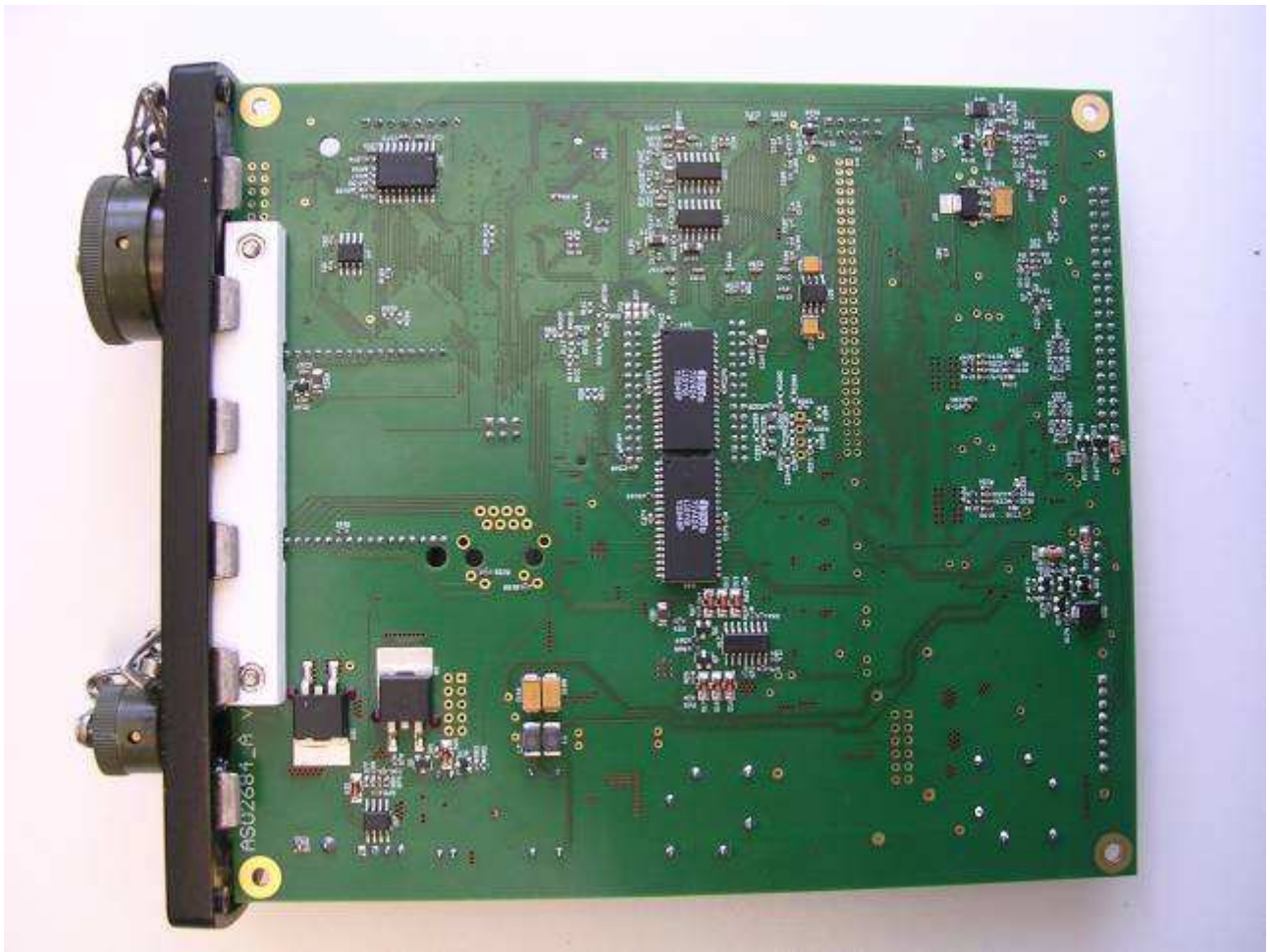
Fig. 5: D.A.D. main board (bottom side)
