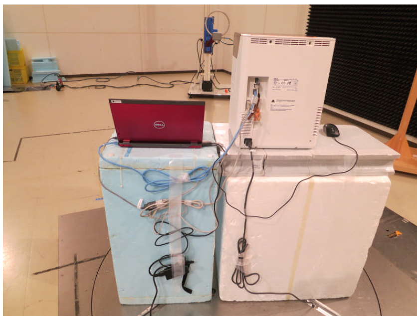
Photo2 Test setup for below 30 MHz ( Back )
