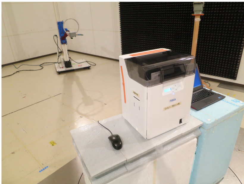
Photo1 Test setup for below 30 MHz ( Front )
