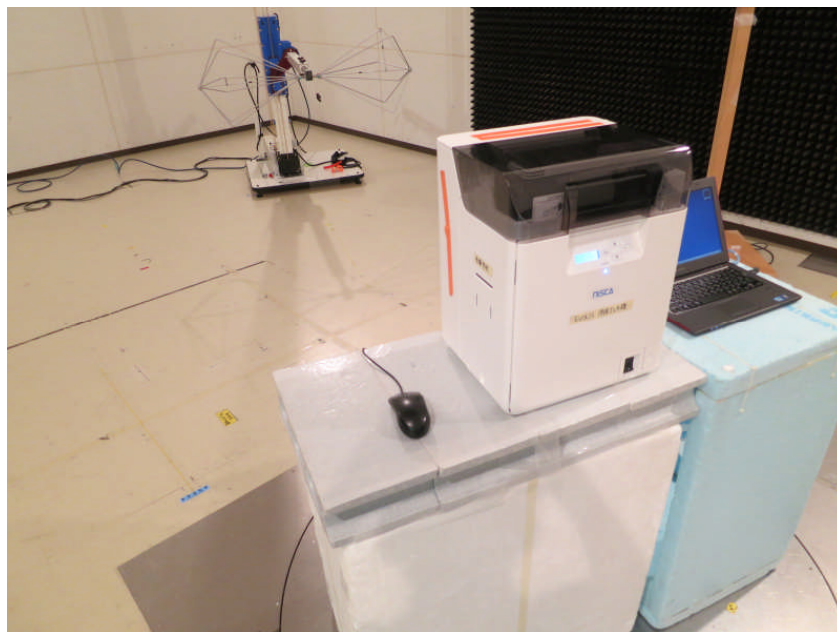
Photo3 Test setup for above 30 MHz ( Front )
