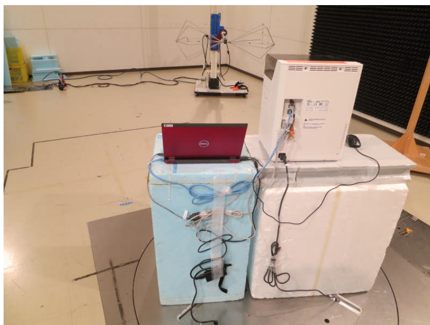
Photo4 Test setup for above 30 MHz ( Back )
