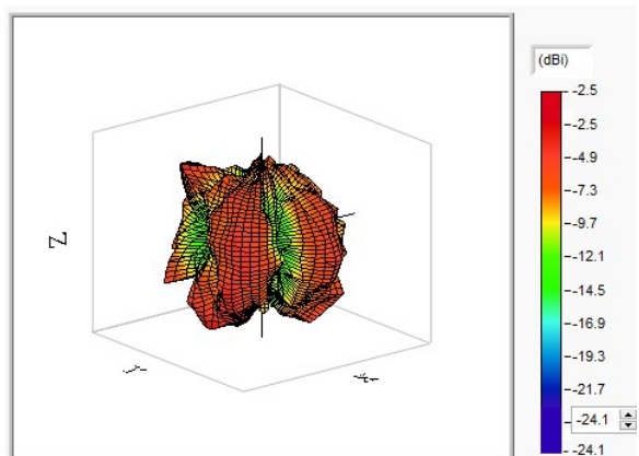
WIFI 5250MHz
