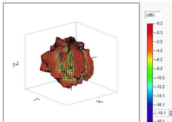
WIFI 2450MHz
