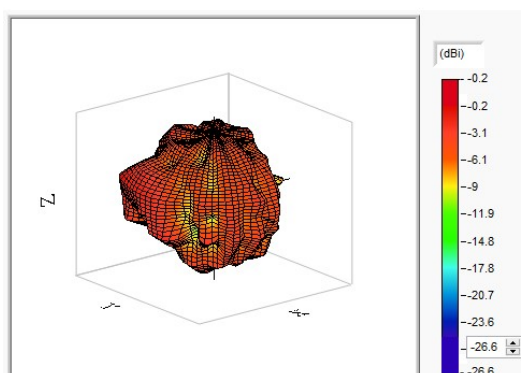
WIFI 2500MHz
