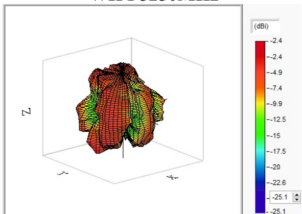
WIFI 5470MHz
