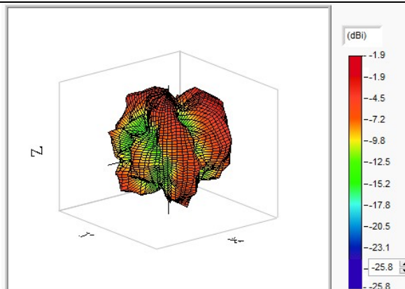
WIFI 5850MHz
