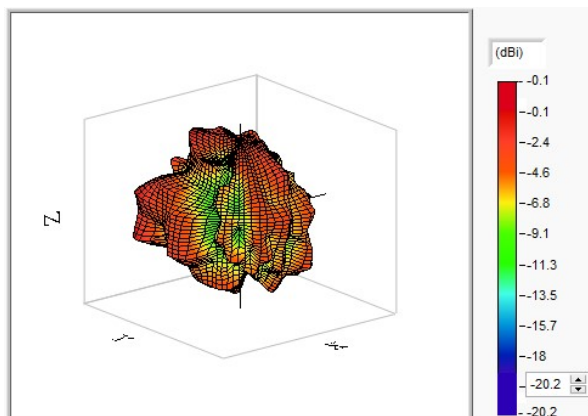
WIFI 2400MHz
