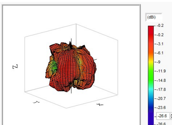
WIFI 5150MHz
