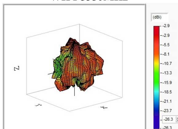
WIFI 5600MHz
