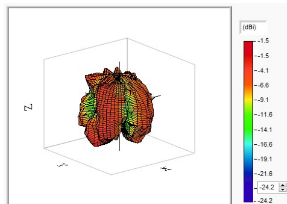
WIFI 5350MHz
