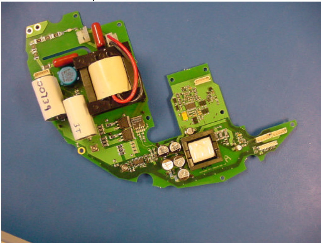
Transmitter component side
