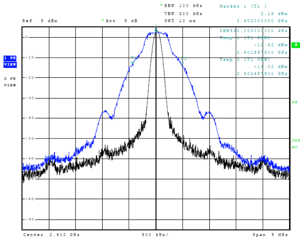
Figure 8 Plot of Transmitter Emissions (99% Occupied Bandwidth)
