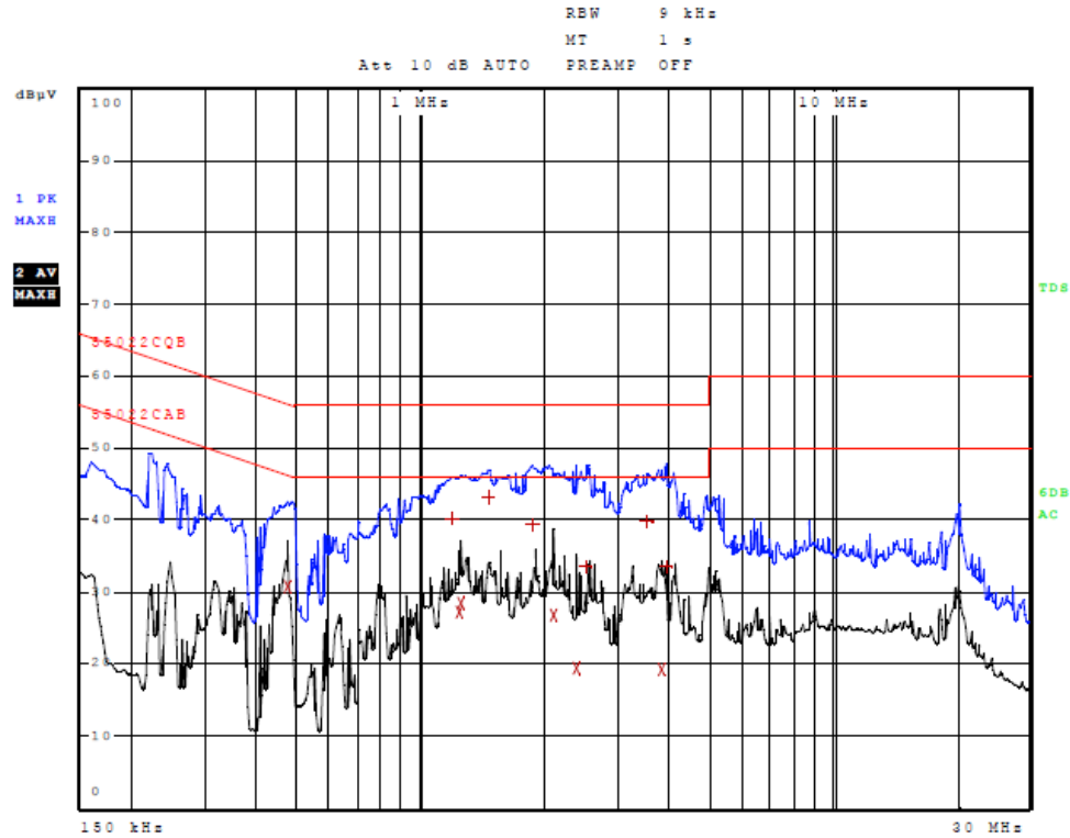
Figure 5 AC Line Conducted emissions of EUT line 1 (EUT-USB-CPU)
