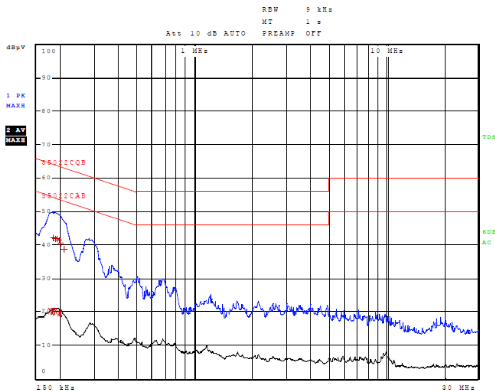
Figure 4 AC Line Conducted emissions of EUT line 2 (EUT AC Adapter #2)
