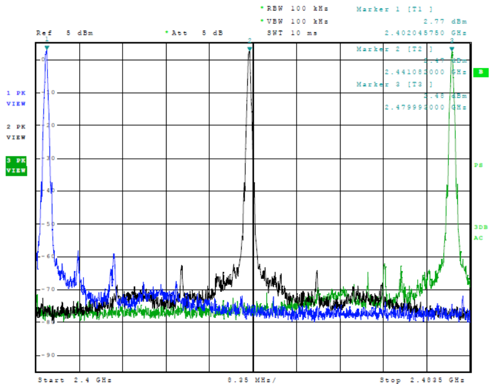
Figure 7 Plot of Transmitter Emissions (In 2402-2480 MHz Band)
