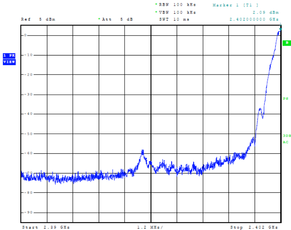
Figure 9 Plot of Transmitter Emissions (Low Band Edge)
