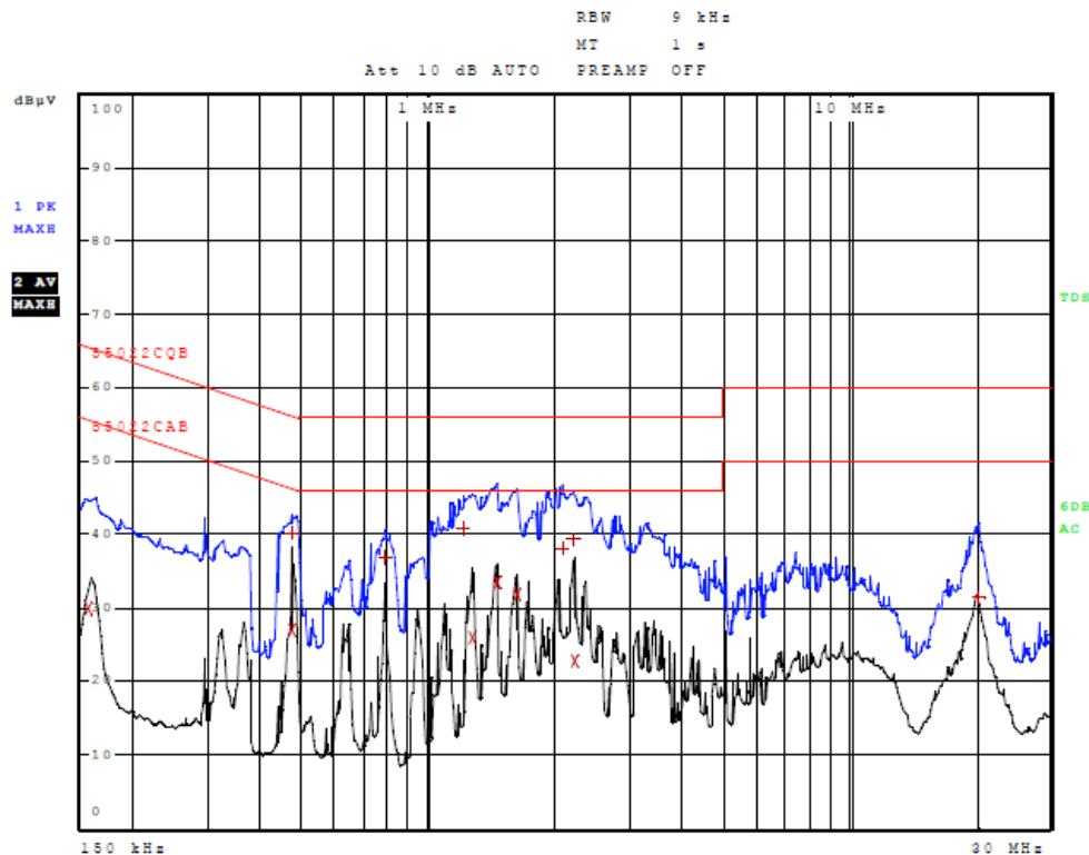
Figure 6 AC Line Conducted emissions of EUT line 2 (EUT-USB-CPU)
