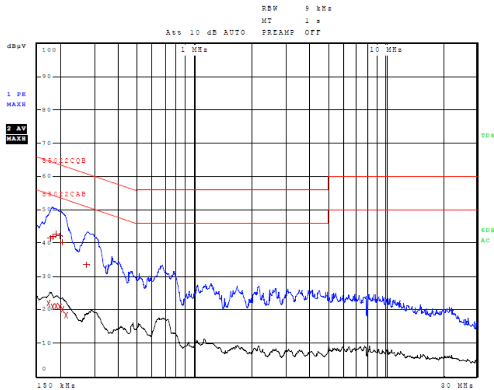
Figure 3 AC Line Conducted emissions of EUT line 1 (EUT AC Adapter #2)
