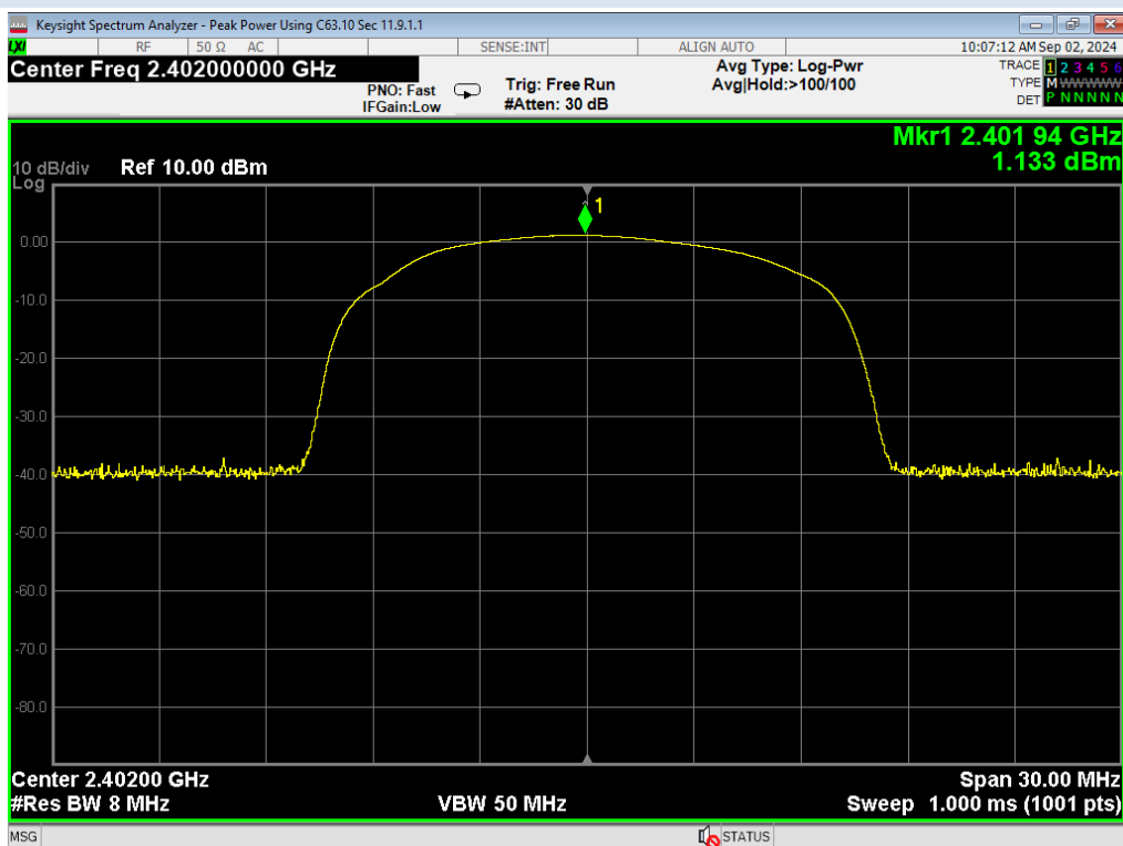
01, Peak Power, ANT GFSK, Low
