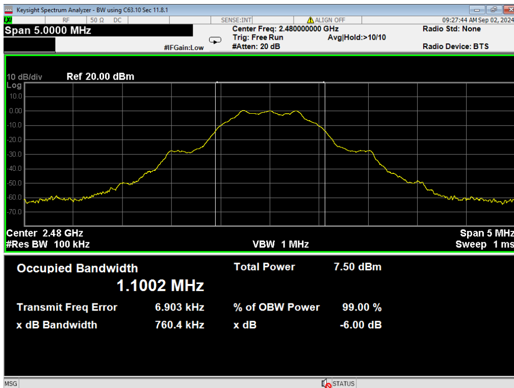
25, 6dB Bandwidth, BLE 1MB, High
