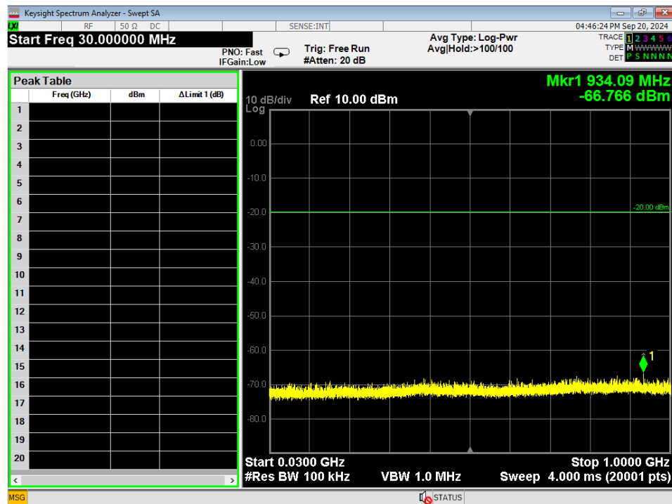
Figure 14 - Radiated Emissions Plot, GMSK 1MB, 30MHz – 1GHz, Mid
