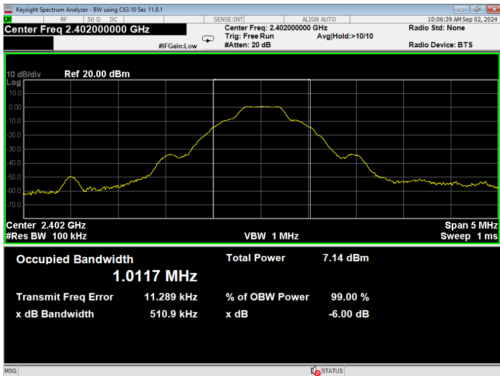
07, 6dB Bandwidth, ANT GFSK, Low
