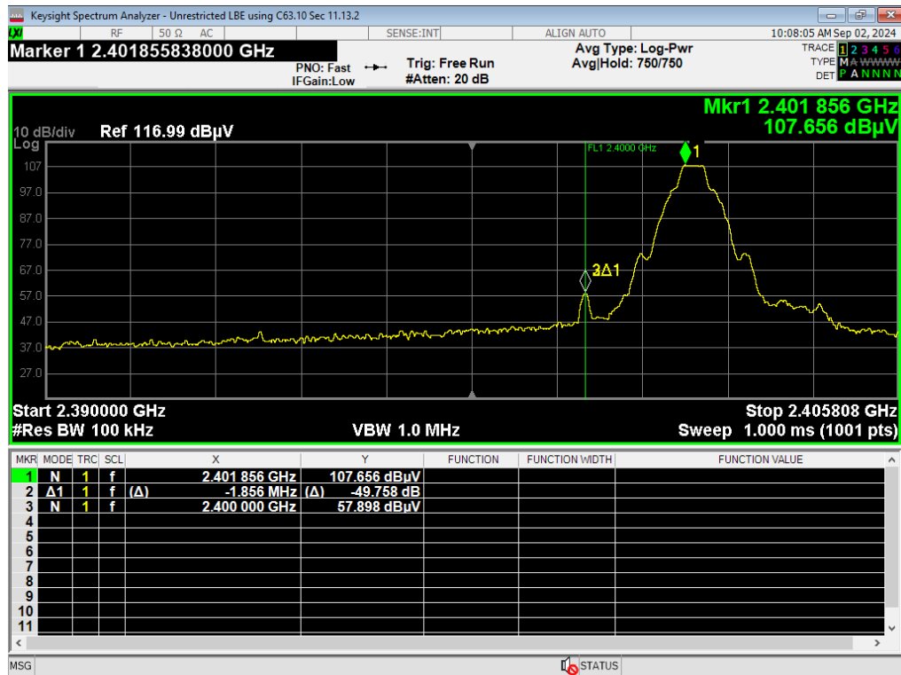
13, LBE Unrestricted, ANT GFSK
