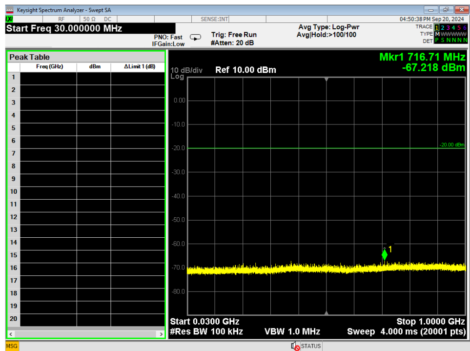
Figure 11 - Radiated Emissions Plot, GFSK, 30MHz – 1GHz, Mid
