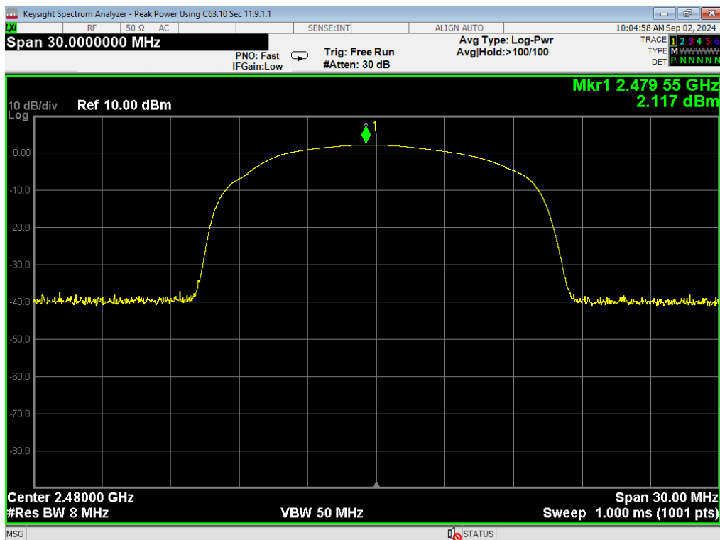
03, Peak Power, ANT GFSK, High
