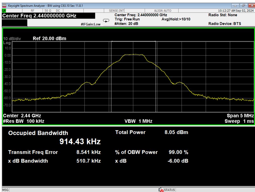
08, 6dB Bandwidth, ANT GFSK, Mid
