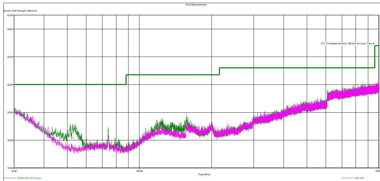
Figure 9 - Radiated Emissions Plot, GMSK 1MB
