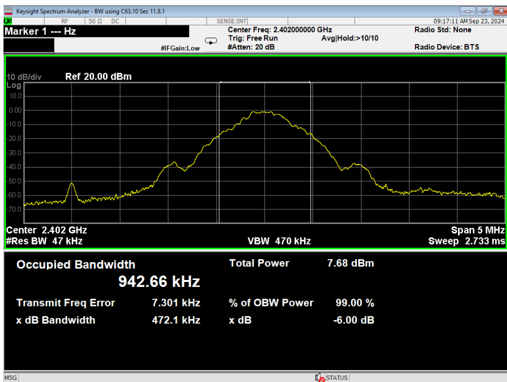
04, Occupied Bandwidth, ANT GFSK, Low
