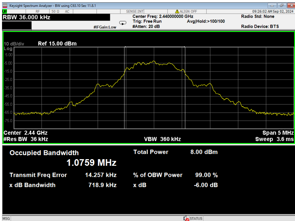
21, Occupied Bandwidth, BLE 1MB, Mid
