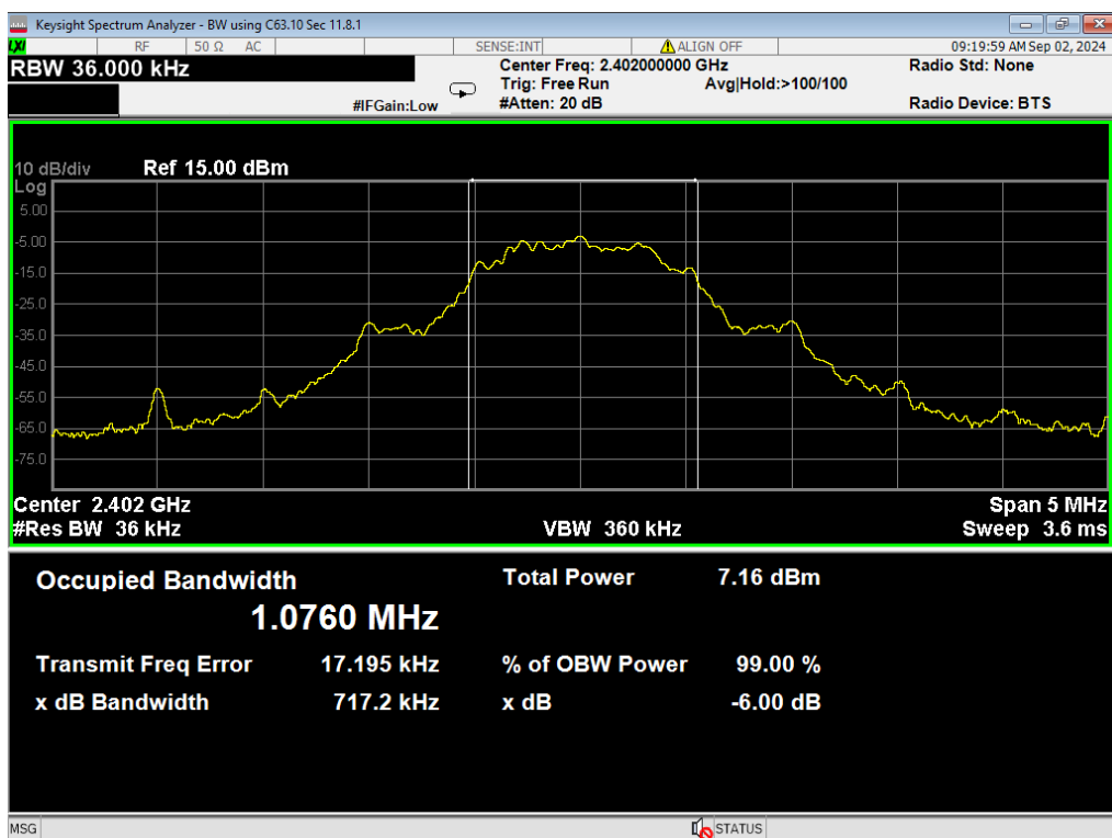
20, Occupied Bandwidth, BLE 1MB, Low
