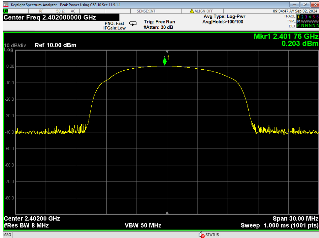
17, Peak Power, BLE 1MB, Low
