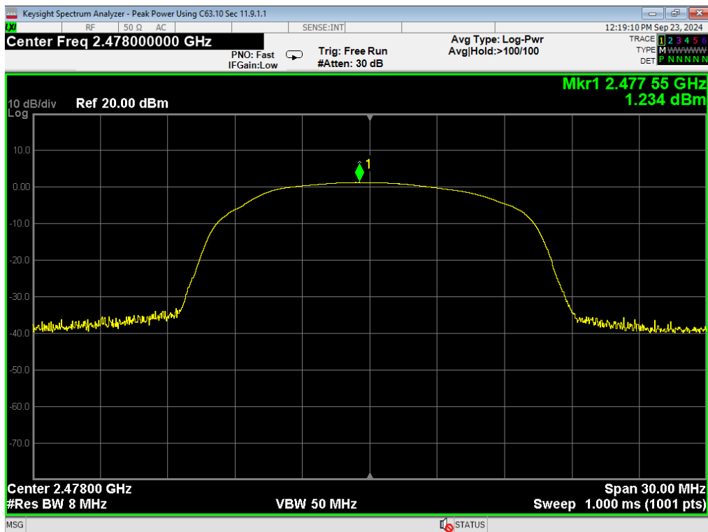
35, Peak Power, BLE 2MB, High
