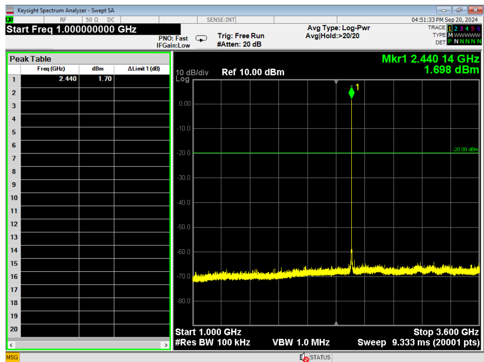
Figure 12 - Radiated Emissions Plot, GFSK, 1GHz – 3.6GHz, Mid
