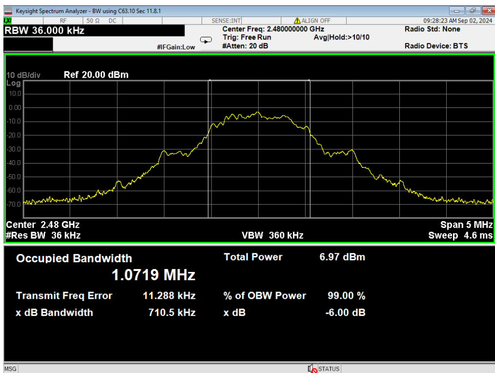
22, Occupied Bandwidth, BLE 1MB, High
