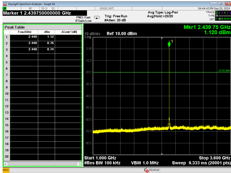
Figure 15 - Radiated Emissions Plot, GMSK 1MB, 1GHz – 3.6GHz, Mid
