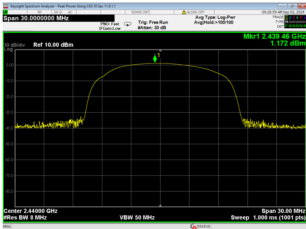
18, Peak Power, BLE 1MB, Mid
