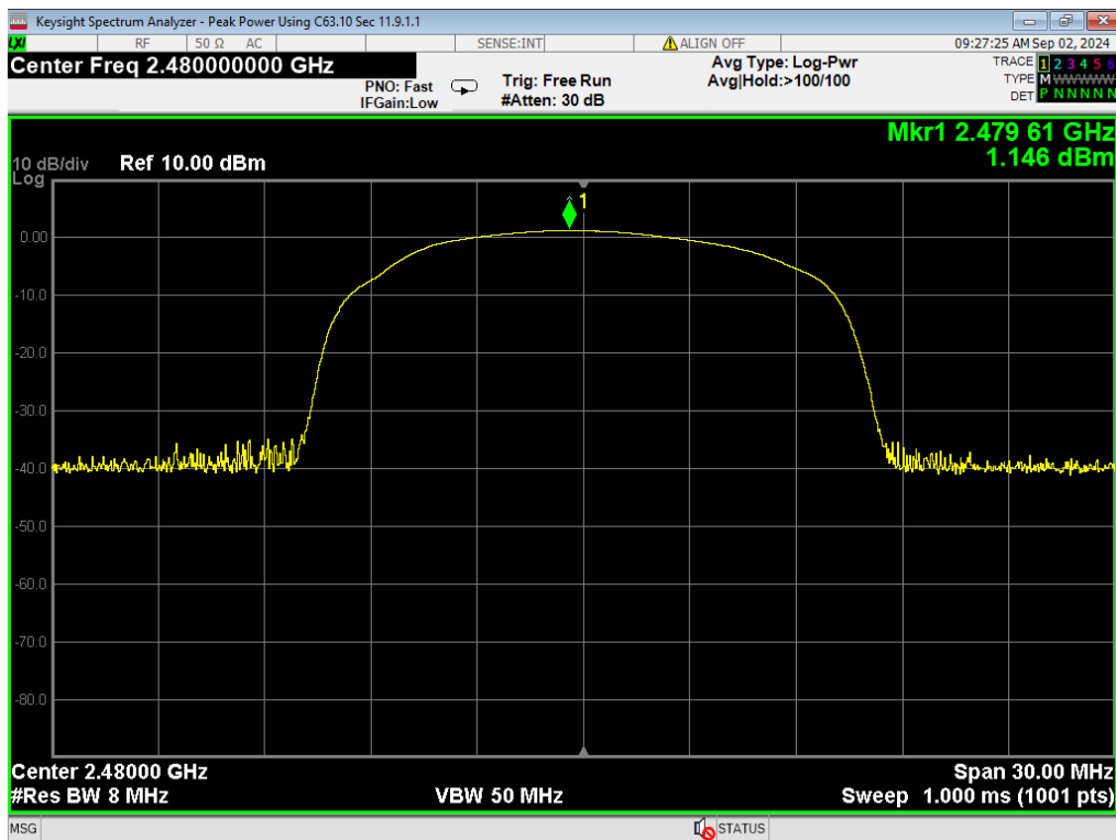
19, Peak Power, BLE 1MB, High
