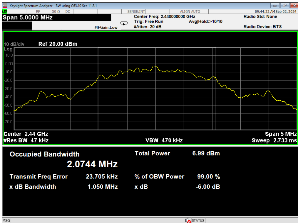
37, Occupied Bandwidth, BLE 2MB, Mid
