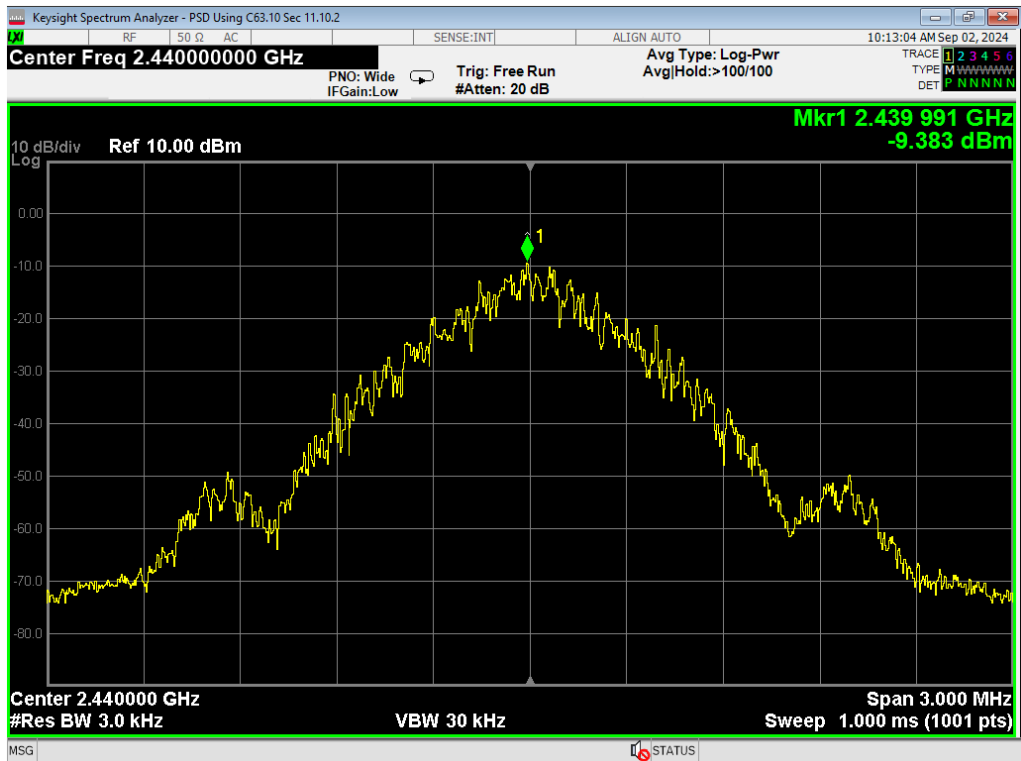
11, PSD, ANT GFSK, Mid
