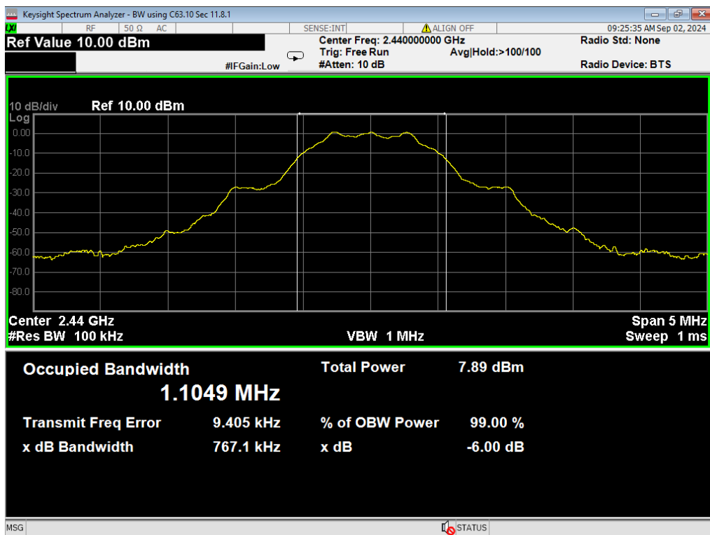
24, 6dB Bandwidth, BLE 1MB, Mid
