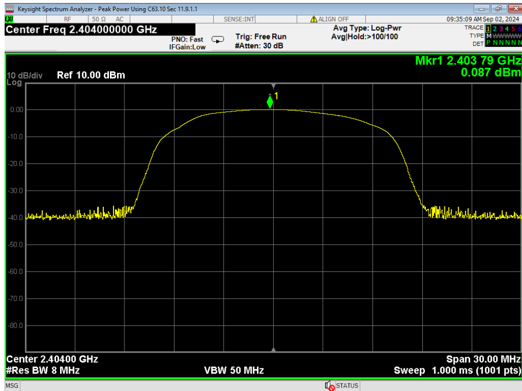
33, Peak Power, BLE 2MB, Low
