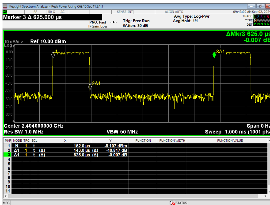
Figure 5 – Duty Cycle, GMSK 2MB
