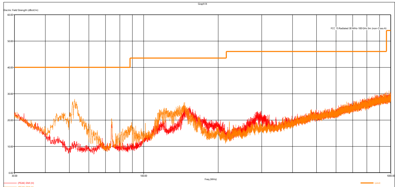
Figure 7 - Radiated Emissions Plot, Receive
