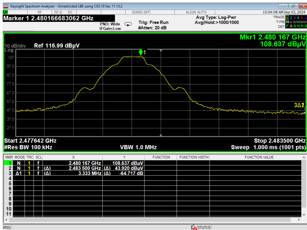
14, HBE Unrestricted, ANT GFSK
