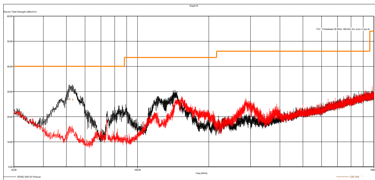
Figure 10 - Radiated Emissions Plot, GMSK 2MB
