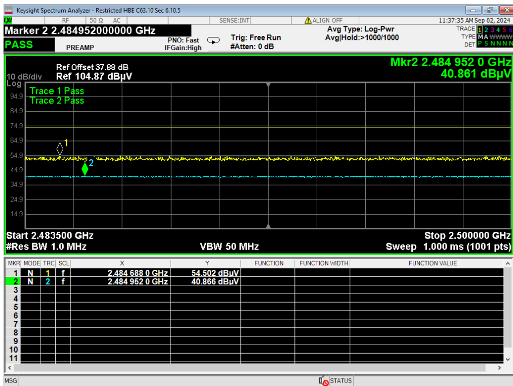
16, HBE Restricted, ANT GFSK
