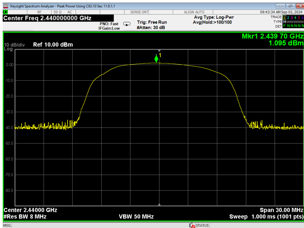
34, Peak Power, BLE 2MB, Mid
