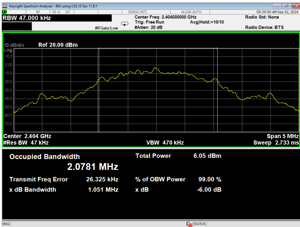
36, Occupied Bandwidth, BLE 2MB, Low
