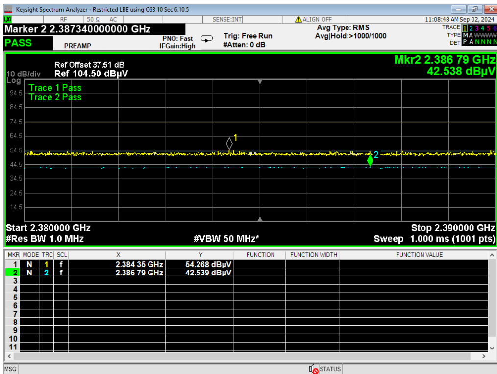
15, LBE Restricted, ANT GFSK
