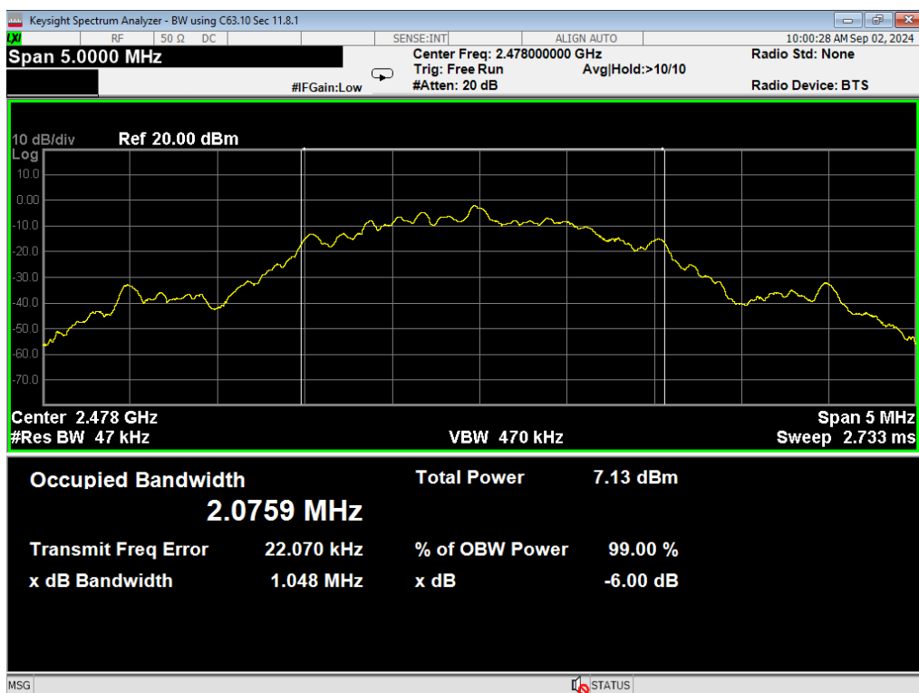
38, Occupied Bandwidth, BLE 2MB, High
