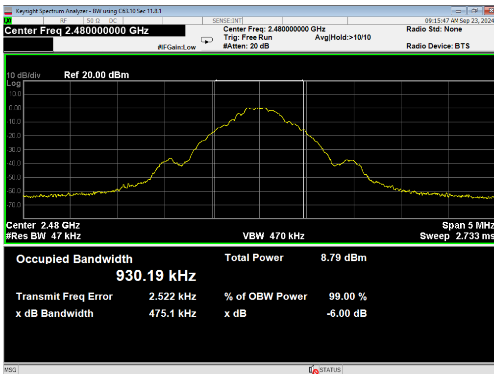
06, Occupied Bandwidth, ANT GFSK, High
