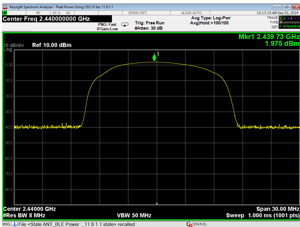
02, Peak Power, ANT GFSK, Mid
