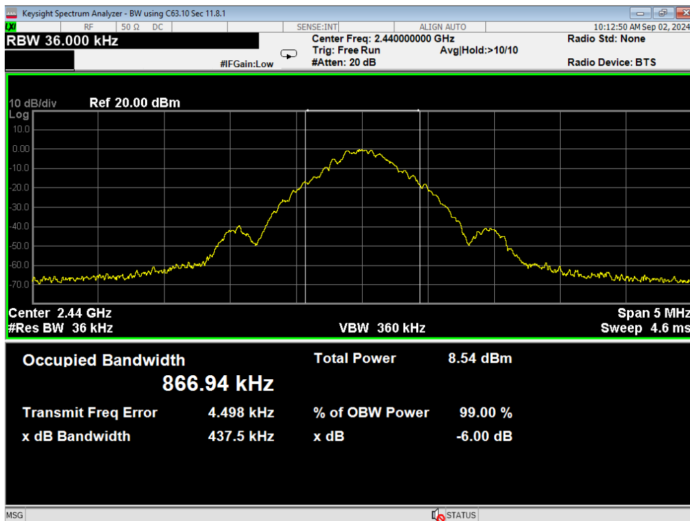
05, Occupied Bandwidth, ANT GFSK, Mid
