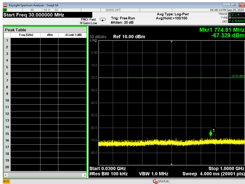
Figure 17 - Radiated Emissions Plot, GMSK 2MB, 30MHz – 1GHz, Mid
