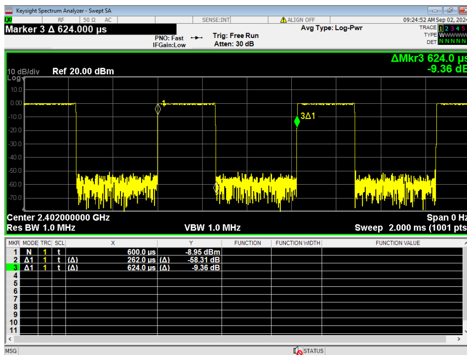
Figure 4 – Duty Cycle, GMSK 1MB
