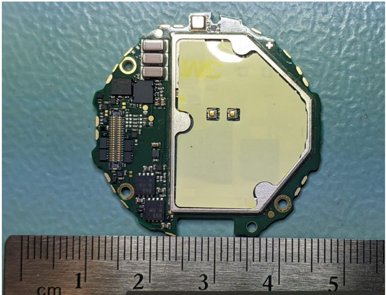
PCB Top (unshielded)
