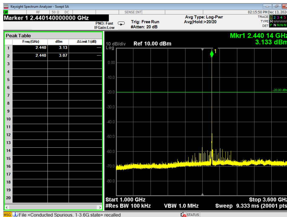
Figure 8 - Conducted Spurious emissions, GFSK, 1GHz – 3.6GHz, Mid
