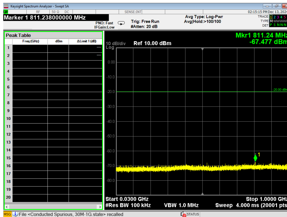
Figure 7 - Conducted Spurious emissions, GFSK, 30MHz – 1GHz, Mid
