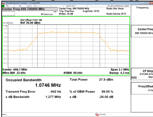
Band12 1.4MHz_Chain0 699.7MHz_NBI 0_QPSK 6_0
