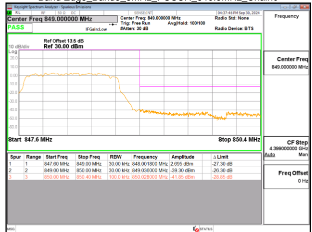
Band Edge_Band5_5MHz_PUSCH_846.5MHz_Chain0
