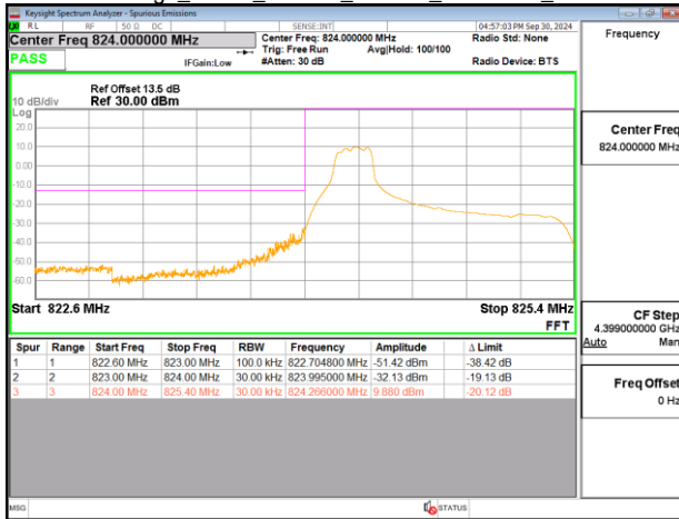
Band Edge_Band5_1.4MHz_PUSCH_824.7MHz_Chain0
