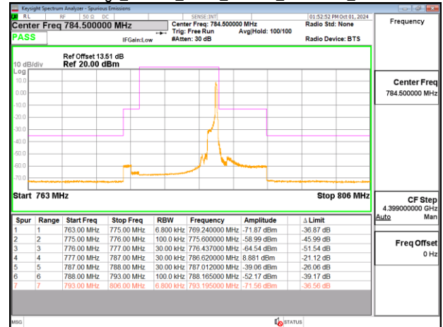
Band Edge_Band13_5MHz_PUSCH_784.5MHz_Chain0
