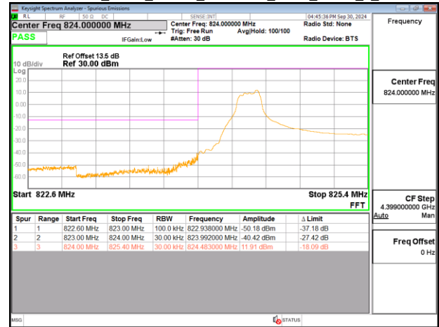
Band5_3MHz_Chain0_825.5MHz_NBI_0_QPSK_6_0
