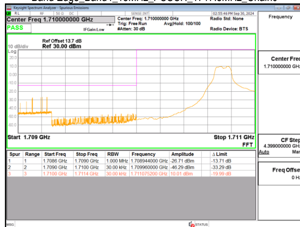
Band Edge_Band4_15MHz_PUSCH_1717.5MHz_Chain0
