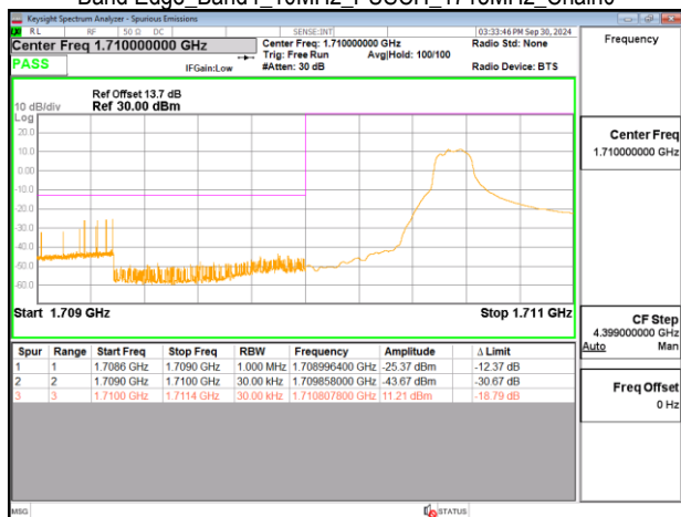
Band Edge_Band4_10MHz_PUSCH_1715MHz_Chain0
