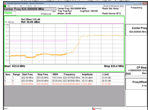
Band5_3MHz_Chain0_825.5MHz_NBI_0_QPSK_6_0
