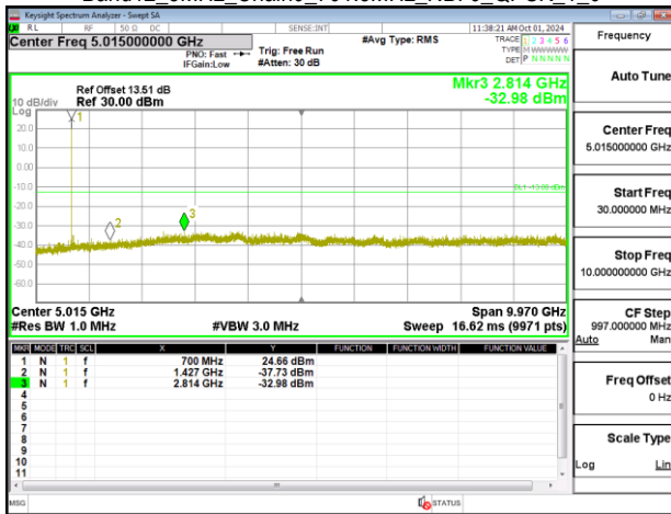
Band12_5MHz_Chain0_707.5MHz_NBI_0_QPSK_1_0
