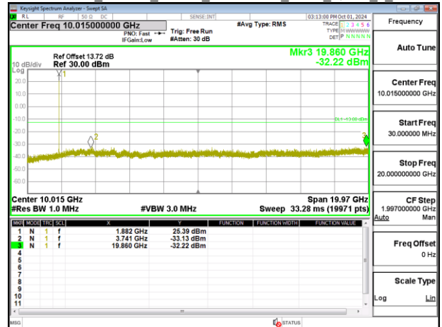
Band25_1.4MHz_Chain0_1882.5MHz_NBI_0_QPSK_1_0
