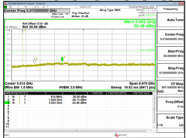
Band26-Part90s_5MHz_Chain0_819MHz_NBI_0_QPSK_1_0
