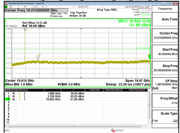
Band25_5MHz_Chain0_1882.5MHz_NBI 0_QPSK_1_0
