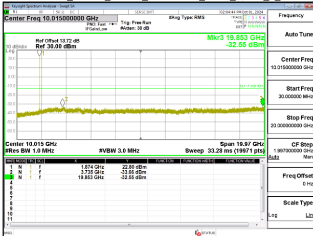
Band25_20MHz_Chain0_1882.5MHz_NBI_0_QPSK_1_0
