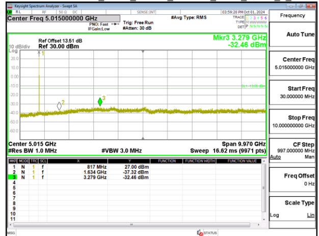
Band26-Part90s_5MHz_Chain0_819MHz_NBI_0_QPSK_1_0
