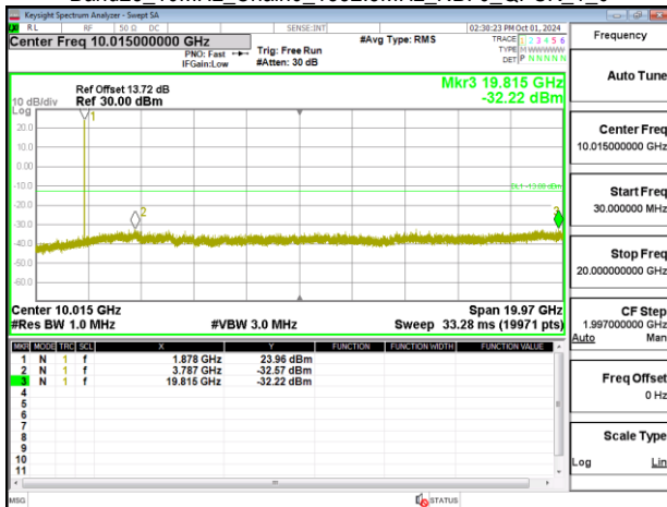
Band25_10MHz_Chain0_1882.5MHz_NBI 0_QPSK_1_0
