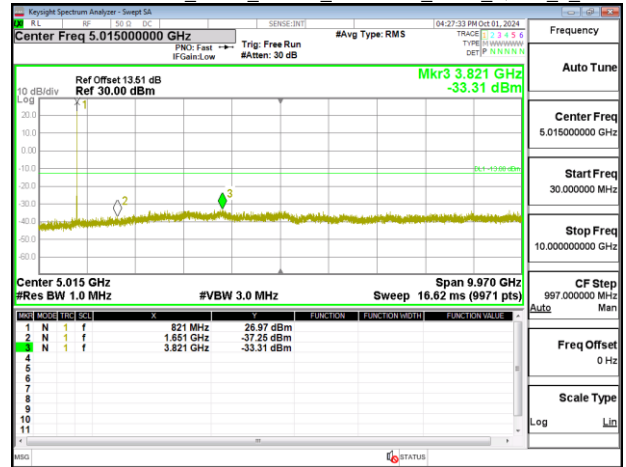
Band26-Part90s_5MHz_Chain0_816.5MHz_NBI_0_QPSK_1_0
