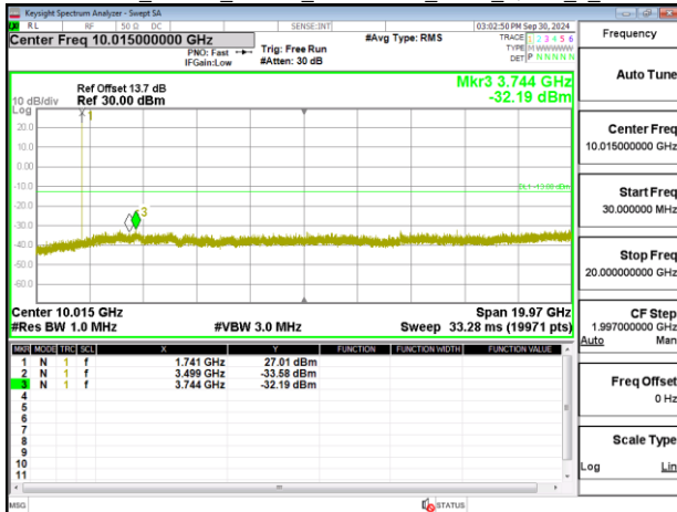
Band4_15MHz_Chain0_1747.5MHz_NBI_0_QPSK_1_0
