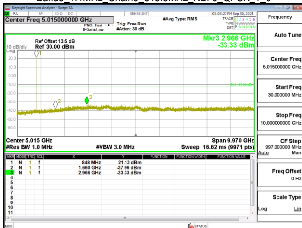
Band5_1.4MHz_Chain0_848.3MHz_NBI_0_QPSK_1_0
