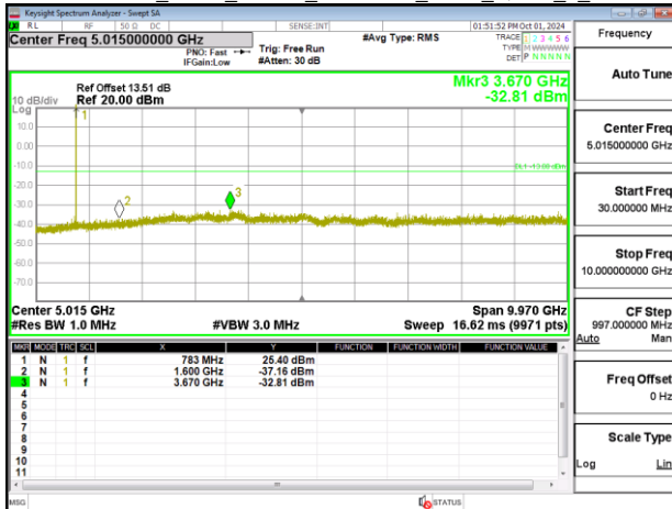
Band13_5MHz_Chain0_784.5MHz_NBI_0_QPSK_1_0
