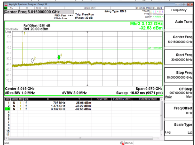
Band12_10MHz_Chain0_711MHz_NBI_0_QPSK_1_0
