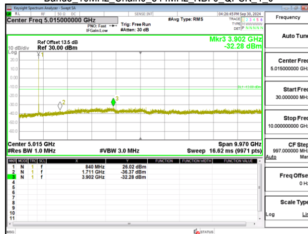
Band5_10MHz_Chain0_844MHz_NBI_0_QPSK_1_0
