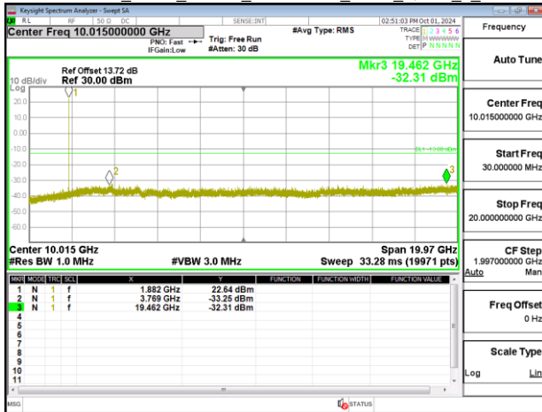
Band25_3MHz_Chain0_1882.5MHz_NBI 0_QPSK_1_0
