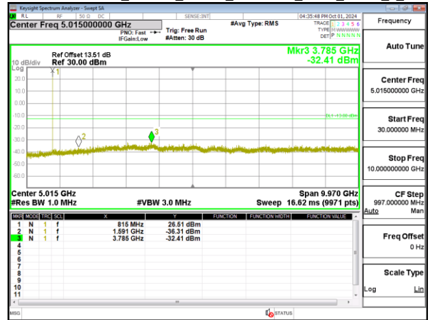
Band26-Part90s_1.4MHz_Chain0_819MHz_NBI_0_QPSK_1_0
