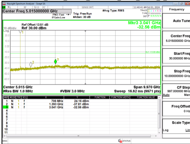
Band12_5MHz_Chain0_713.5MHz_NBI_0_QPSK_1_0
