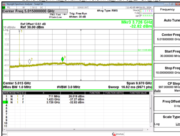
Band12_5MHz_Chain0_713.5MHz_NBI_0_QPSK_1_0
