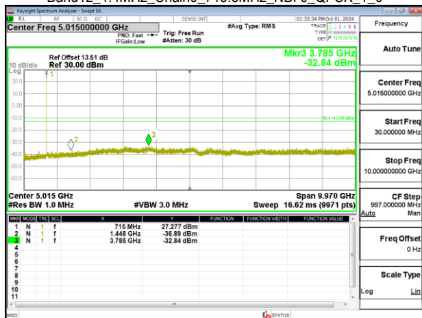
Band12_1.4MHz_Chain0_715.3MHz_NBI 0_QPSK_1_0
