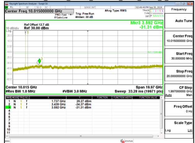
Band4_20MHz_Chain0_1745MHz_NBI_0_QPSK_1_0
