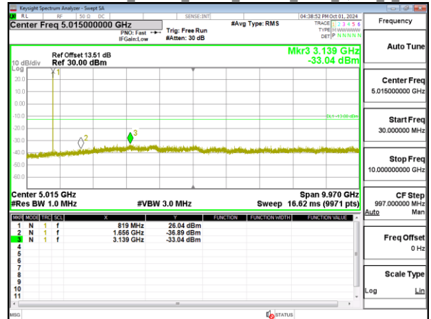
Band26-Part90s_1.4MHz_Chain0_819MHz_NBI_0_QPSK_1_0
