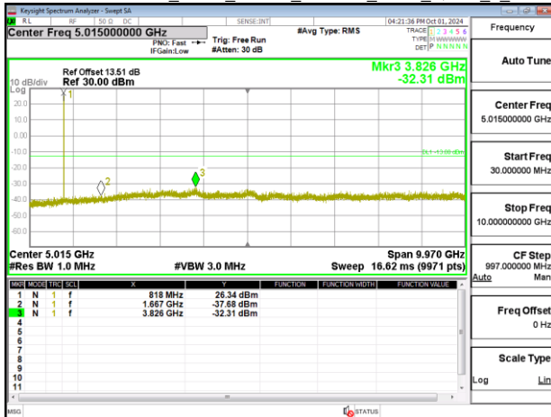
Band26-Part90s_3MHz_Chain0_819MHz_NBI_0_QPSK_1_0
