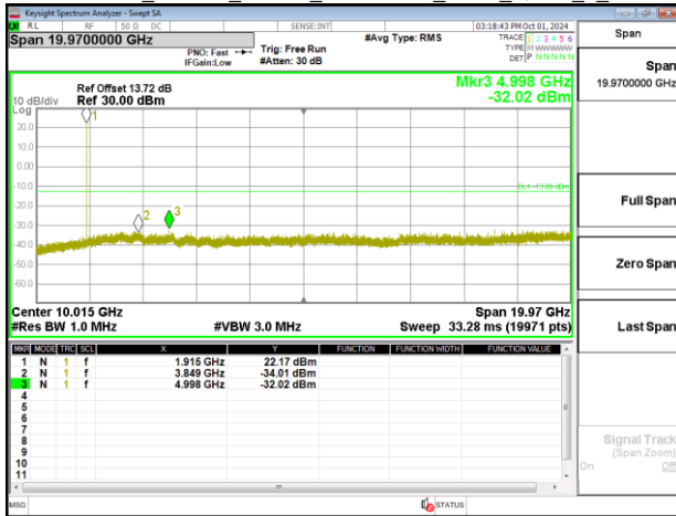
Band25_3MHz_Chain0_1851.5MHz_NBI 0_QPSK_1_0
