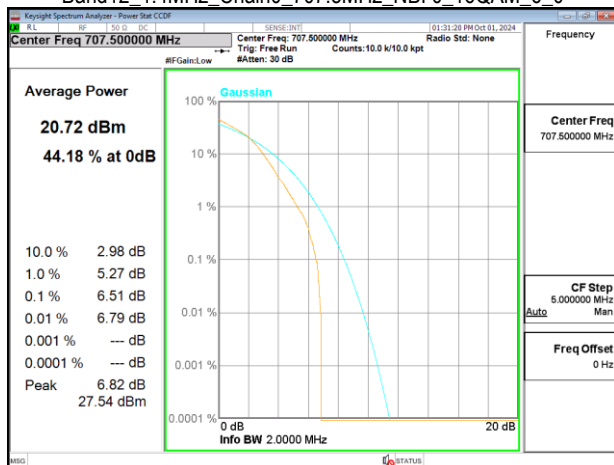
Band12_1.4MHz_Chain0_707.5MHz_NBI 0_16QAM_6_0
