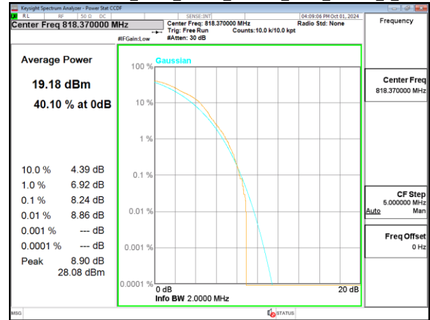
Band26-Part90s_5MHz_Chain0_819MHz_NBI 1_QPSK_6_0
