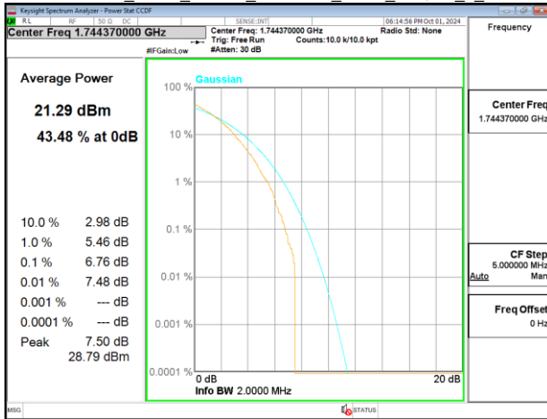
Band66_3MHz_Chain0_1745MHz_NBI 0_QPSK_6_0
