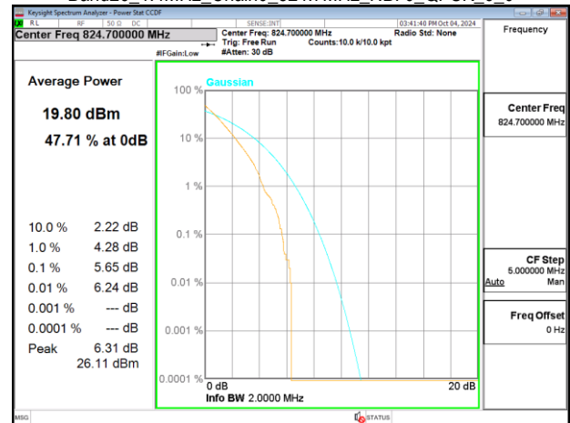
Band26_1.4MHz_Chain0_824.7MHz_NBI 0_QPSK_6_0
