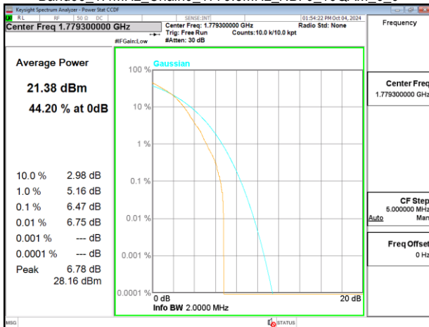
Band66_1.4MHz_Chain0_1779.3MHz_NBI 0_16QAM_6_0
