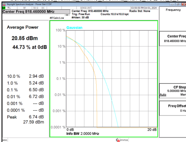
Band26-Part90s_10MHz_Chain0_819MHz_NBI 3_16QAM_6_0
