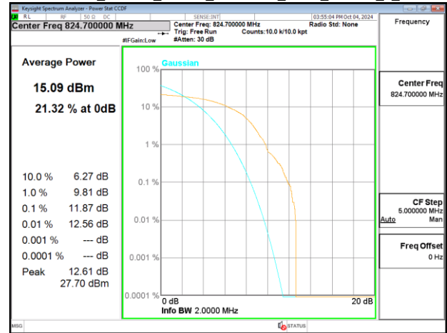
Band26_1.4MHz_Chain0_824.7MHz_NBI 0_QPSK_6_0
