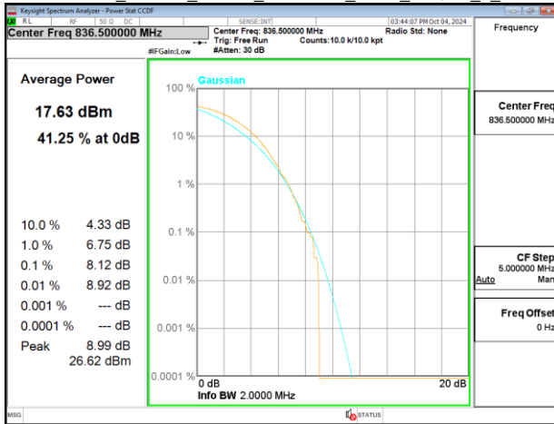
Band26_1.4MHz_Chain0_836.5MHz_NBI 0_QPSK_6_0
