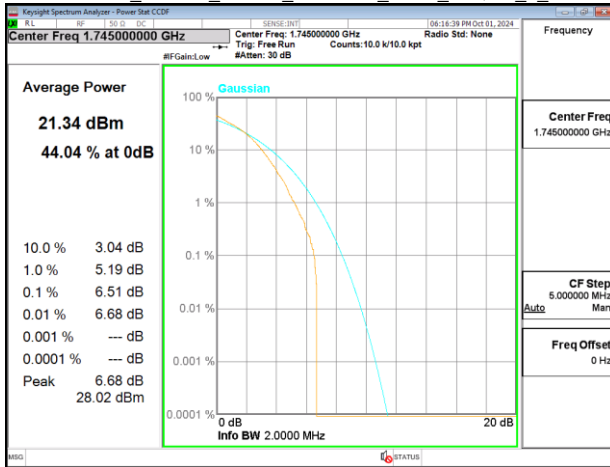
Band66_1.4MHz_Chain0_1745MHz_NBI 0_QPSK_6_0
