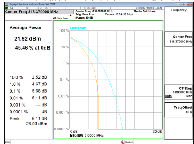
Band26-Part90s_5MHz_Chain0_819MHz_NBI 1_QPSK_6_0
