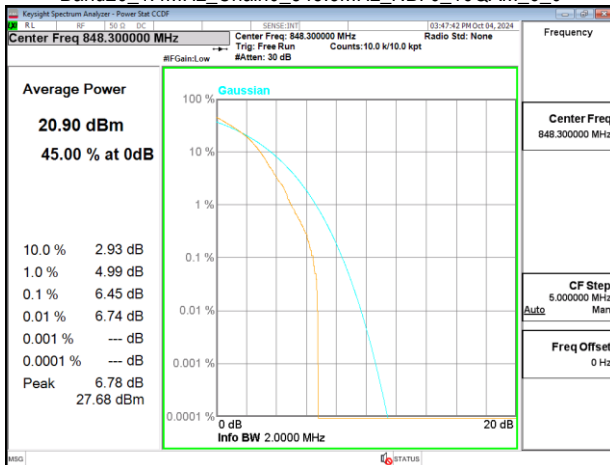
Band26_1.4MHz_Chain0_848.3MHz_NBI 0_16QAM_6_0
