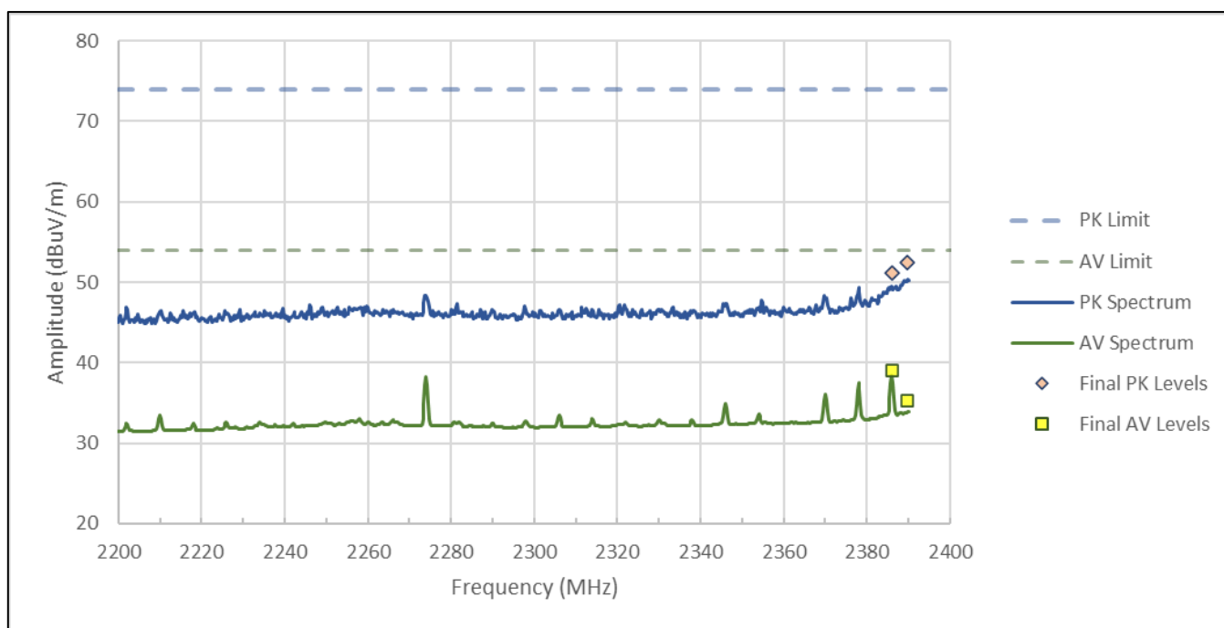
Figure RE04.1: FCC restricted band spectral data from 2200 to 2390 MHz
