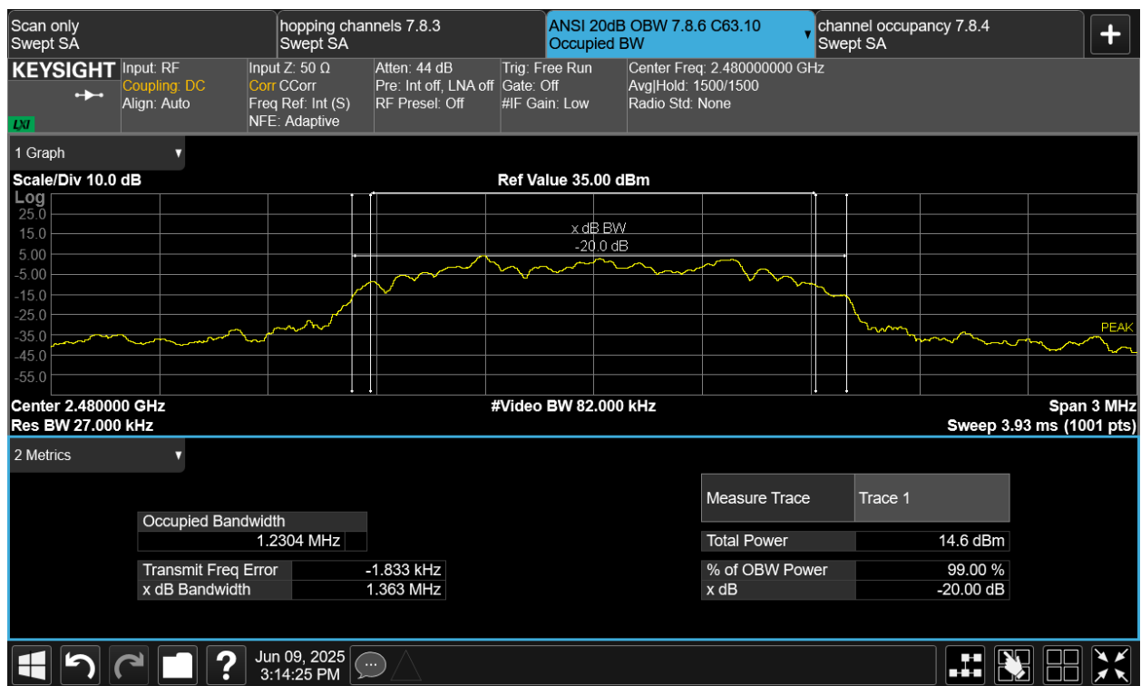
Figure TR51.2: Spectral data for Bluetooth EDR3 modulation at 2480 MHz
