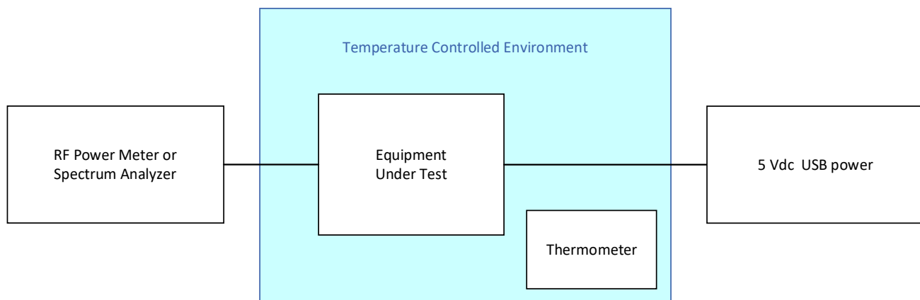
Figure TR01.2: Test equipment setup transmit power over temperature
