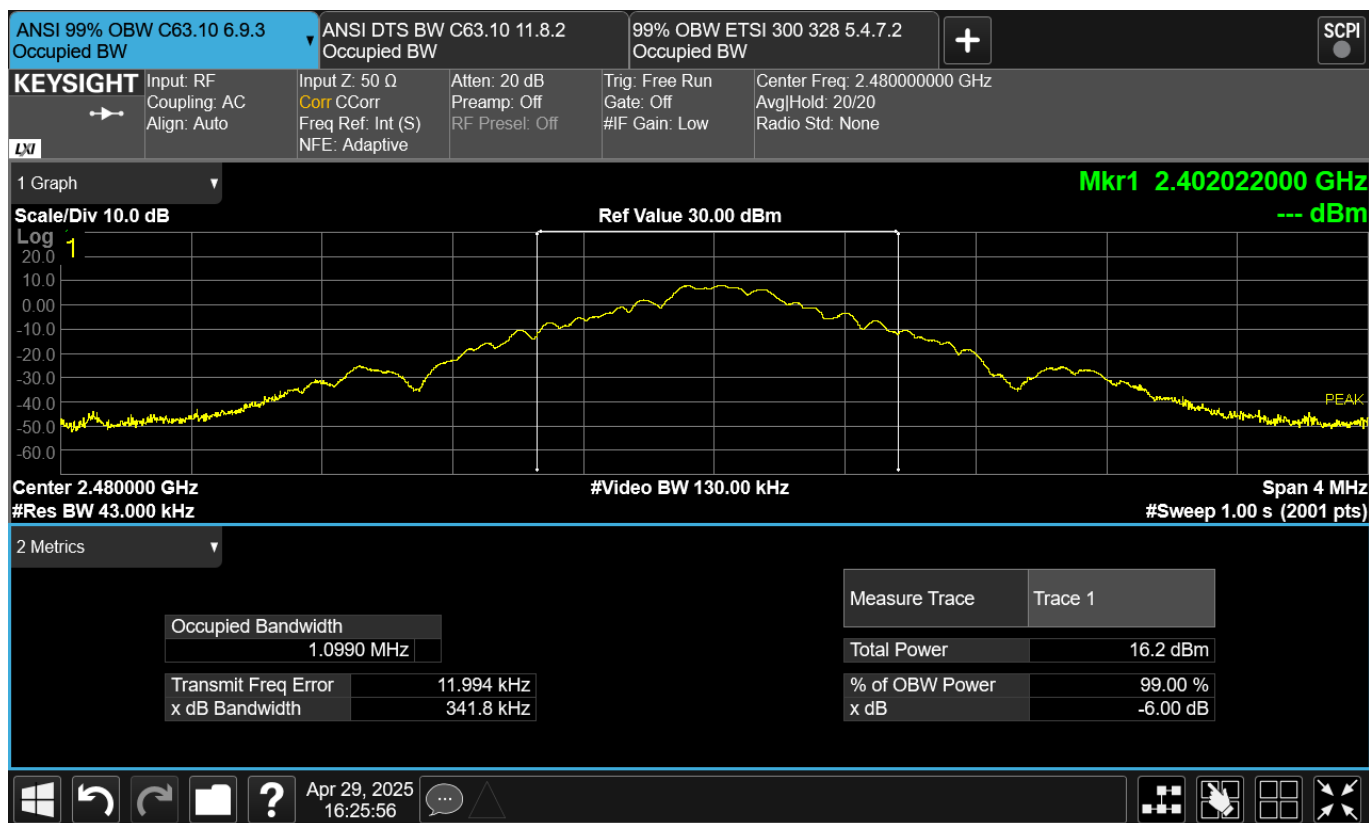
Figure TR09.4: Occupied bandwidth data for Bluetooth EDR3 at channel 2480 MHz
