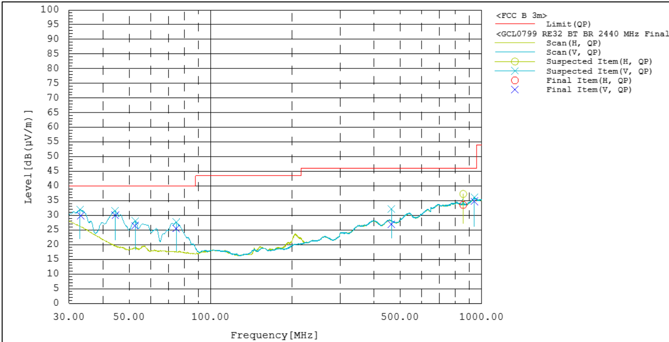
Figure RE32.1: Spectral data (BT, BR, 2440 MHz)
