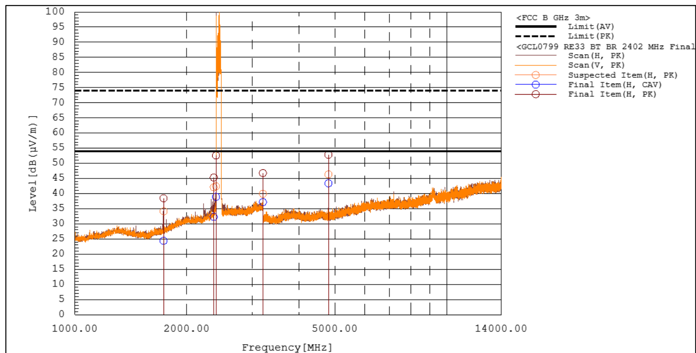
Figure RE33.1: Spectral data (BT, BR, 2402 MHz)
