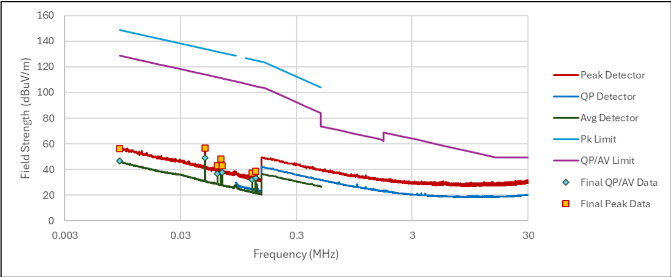
Figure RE31.1: Spectral data (BT, BR, 2440 MHz)
