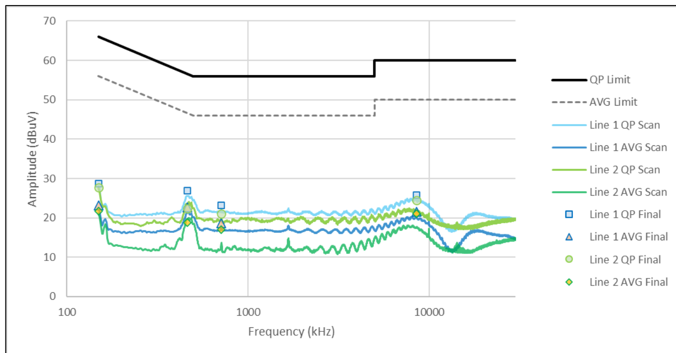
Figure CE01.1: Spectral data (BT, BR, 2440 MHz)
