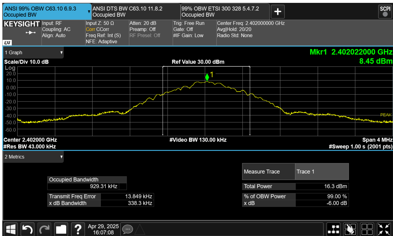
Figure TR09.2: Occupied bandwidth data for Bluetooth BR at channel 2402 MHz
