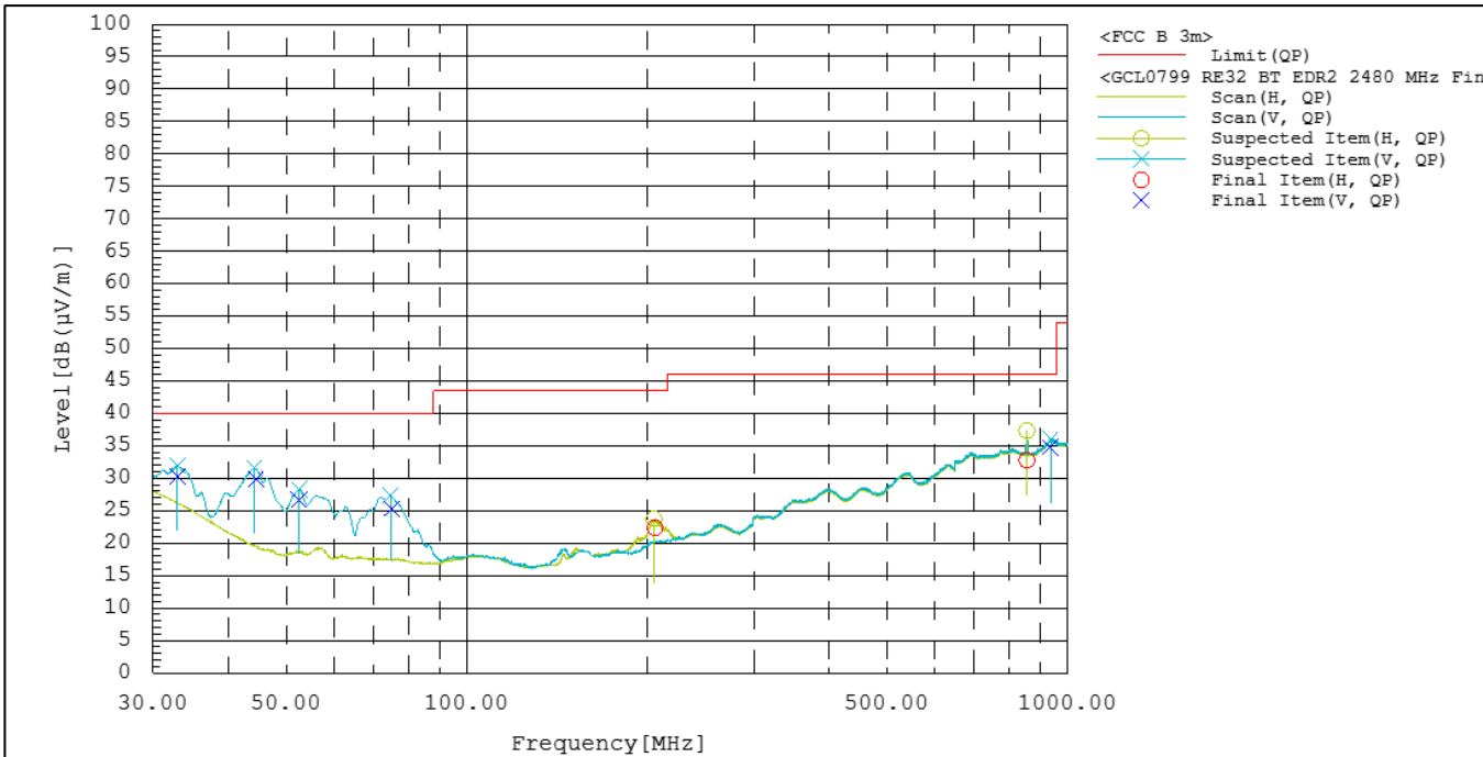
Figure RE32.2: Spectral data (BT, EDR2, 2480 MHz)
