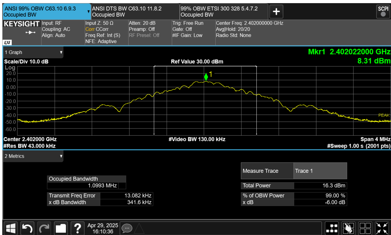
Figure TR09.3: Occupied bandwidth data for Bluetooth EDR2 at channel 2402 MHz
