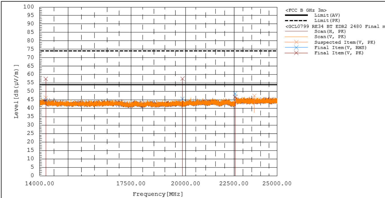
Figure RE34.2: Spectral data (BT, EDR2, 2480 MHz)
