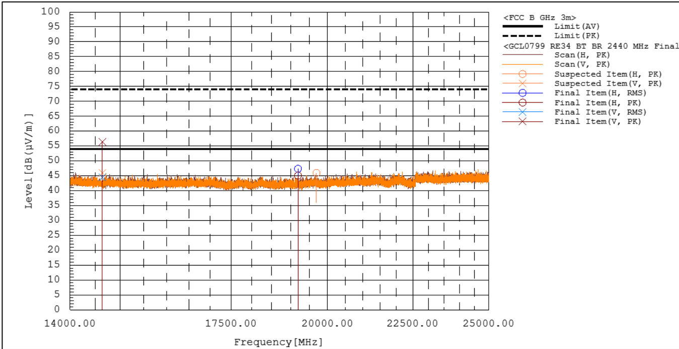
Figure RE34.1: Spectral data (BT, BR, 2440 MHz)
