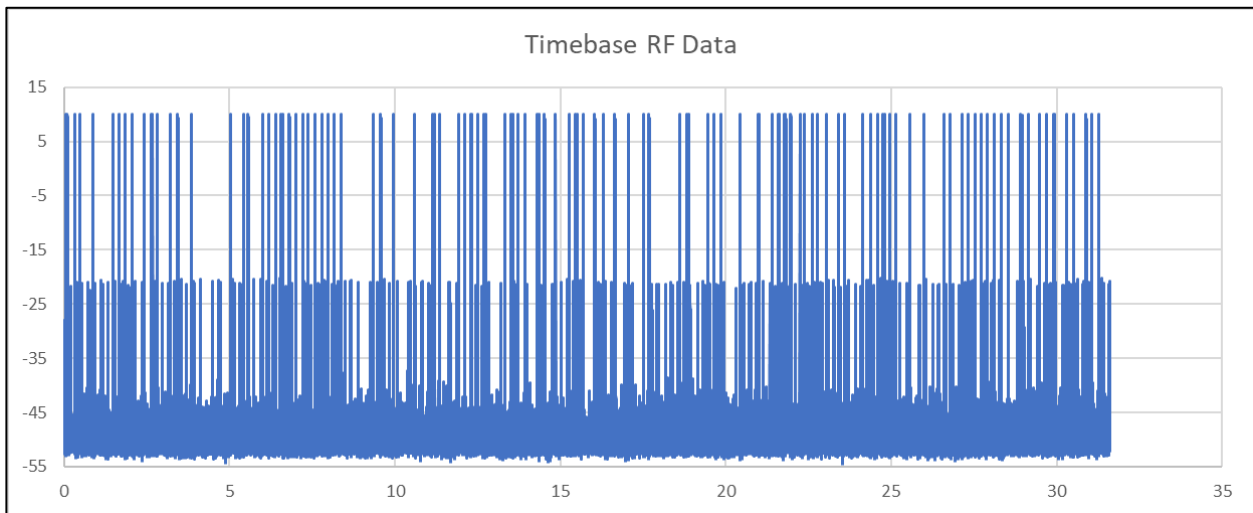
Figure TR51.3: Channel Occupancy time data for Bluetooth EDR3 modulation at 2428 MHz
