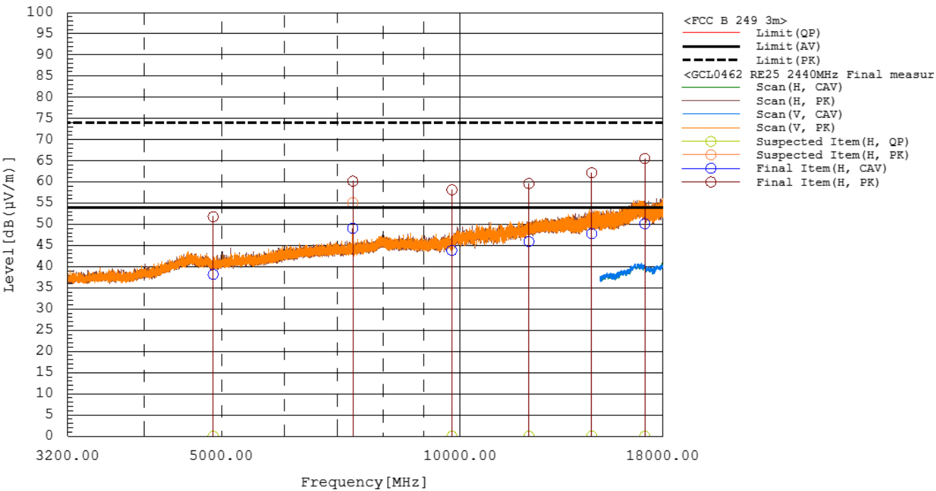
Figure RE25.2: Spectral data (X orientation, 2440 MHz)
