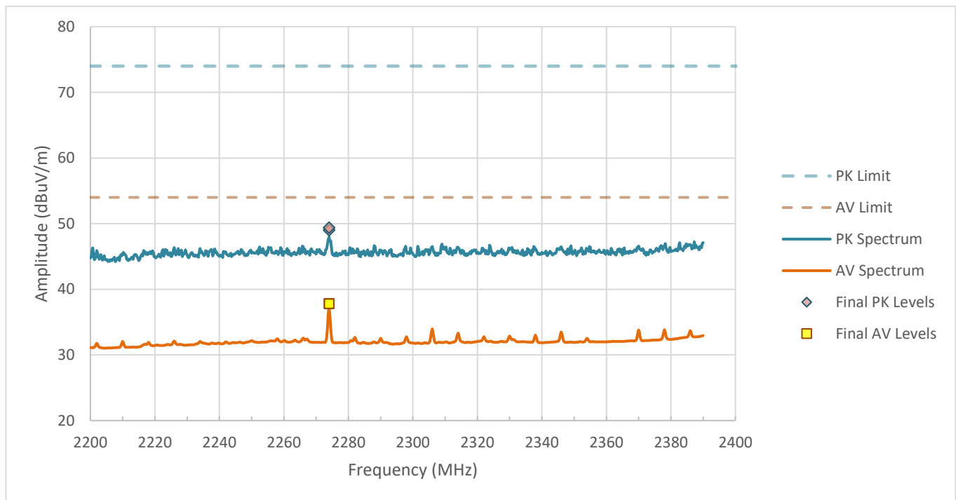
Figure RE04.1: FCC restricted band spectral data from 2200 to 2390 MHz (ANT, X orientation)
