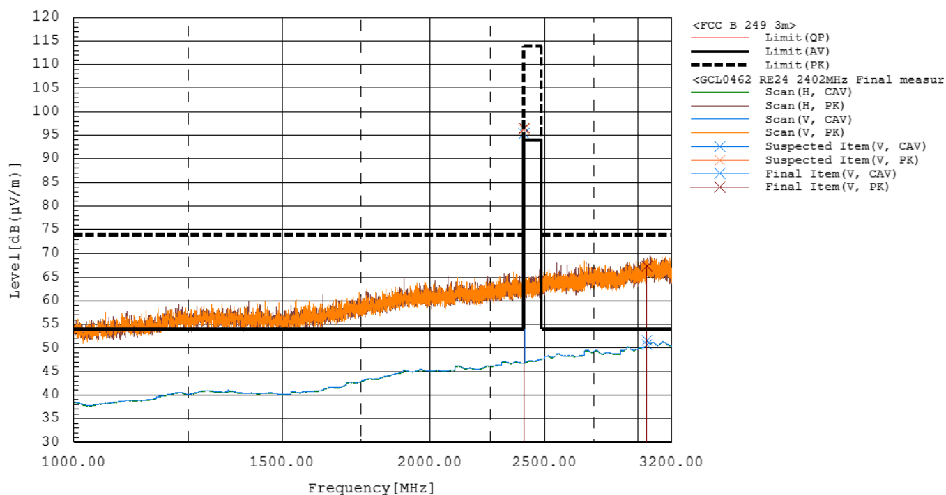
Figure RE24.1: Spectral data (X orientation, ANT 2402MHz)
