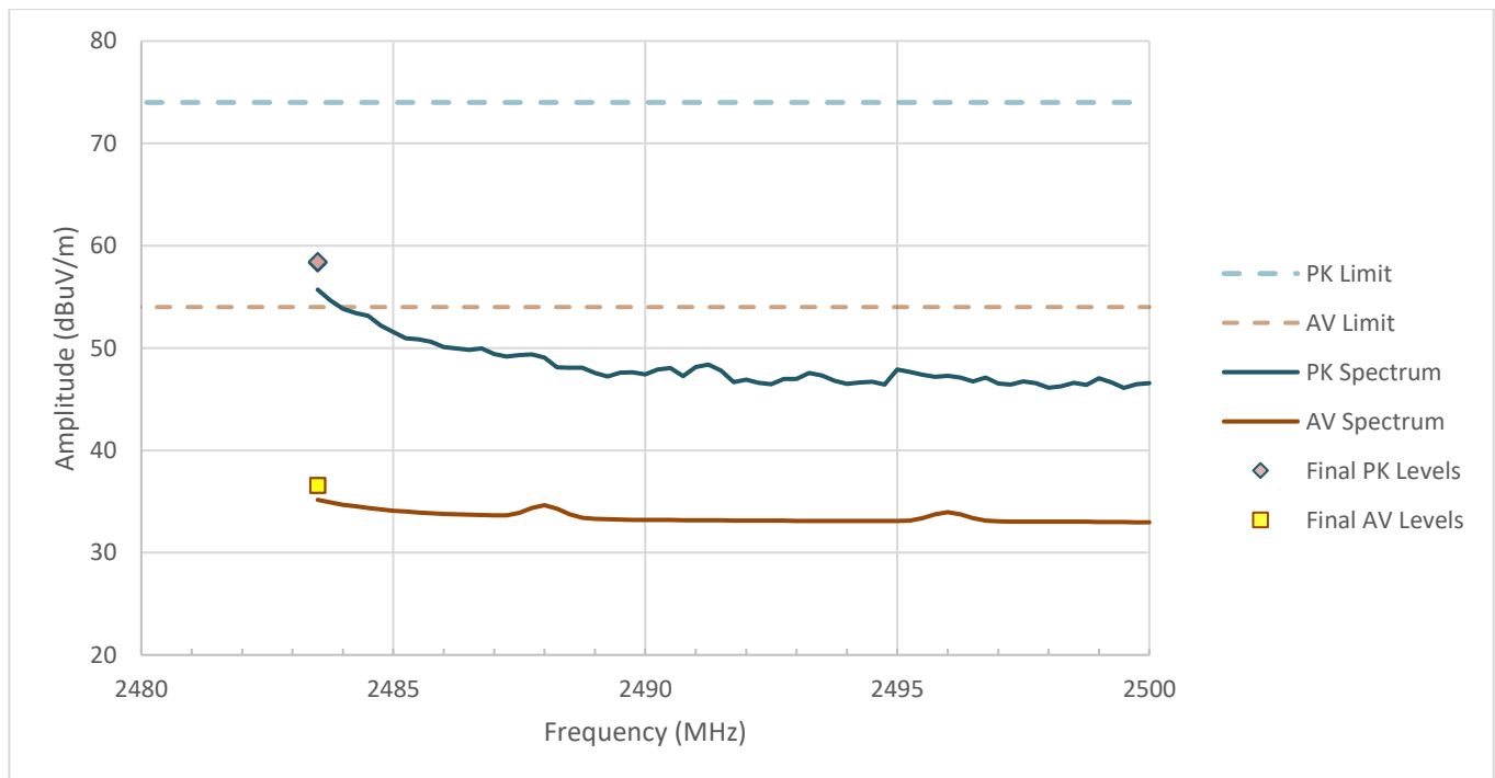
Figure RE04.2: FCC restricted band spectral data from 2483.5 to 2500 MHz (ANT, X orientation)
