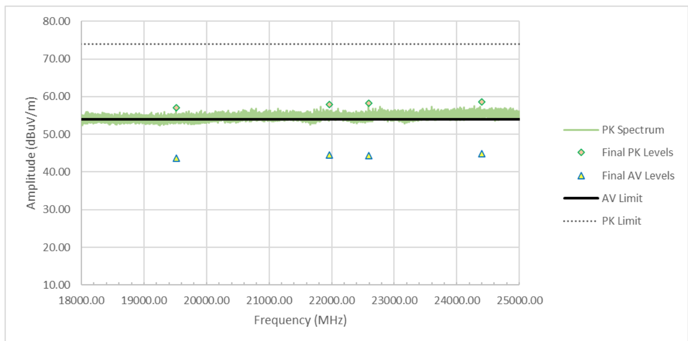
Figure RE26.1: Spectral data
