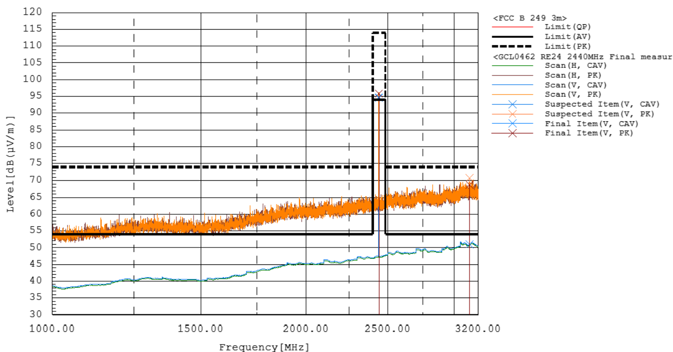
Figure RE24.2: Spectral data (X orientation, ANT 2440MHz)
