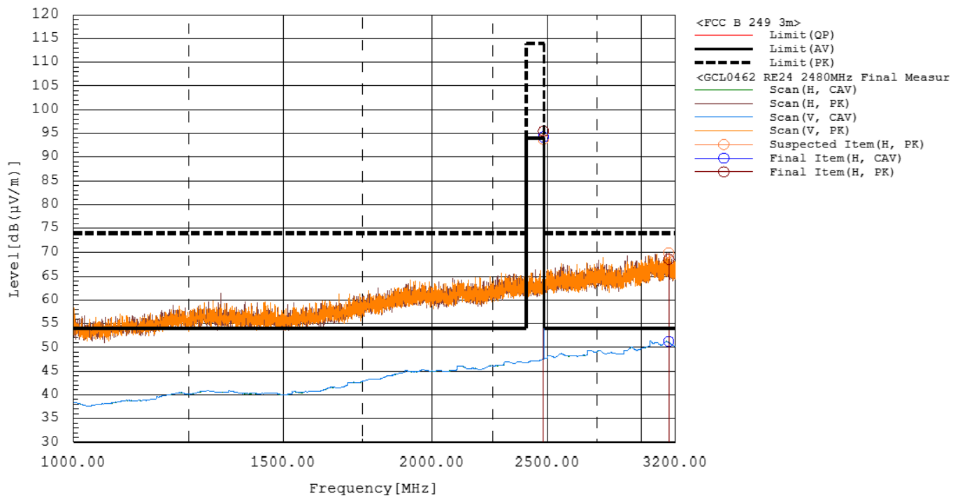
Figure RE24.3: Spectral data (X orientation, ANT 2480MHz)
