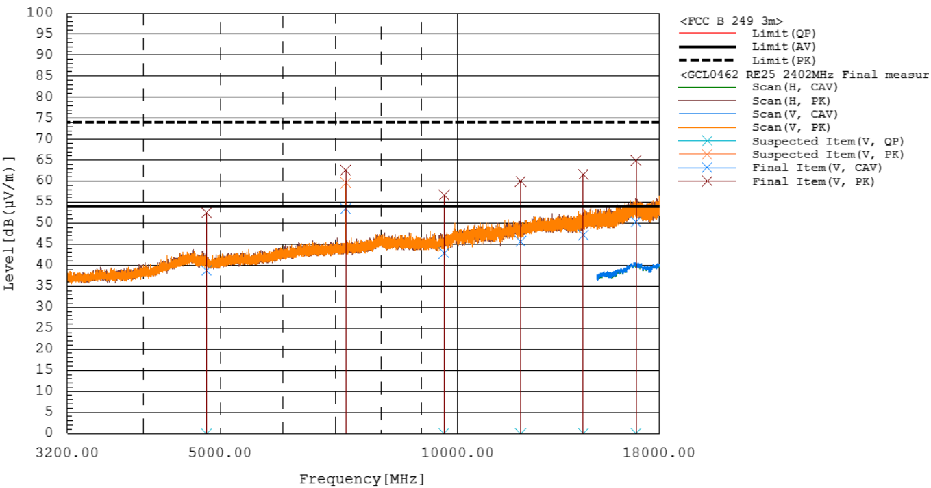
Figure RE25.1: Spectral data (X orientation, 2402 MHz)
