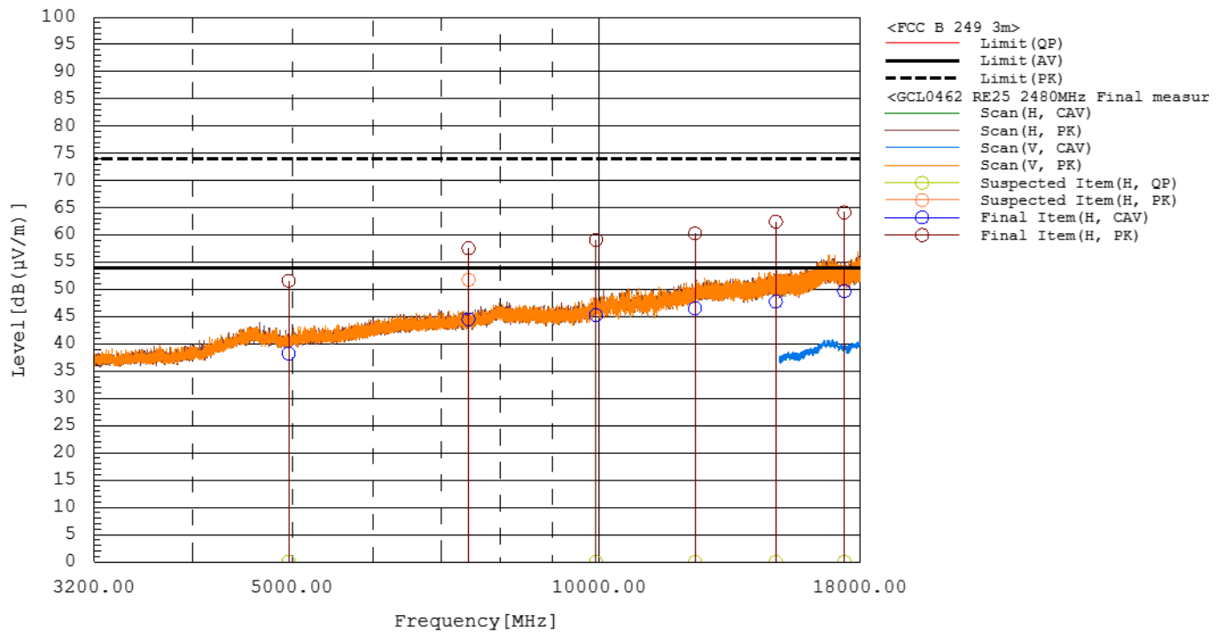
Figure RE25.3: Spectral data (X orientation, 2480 MHz)
