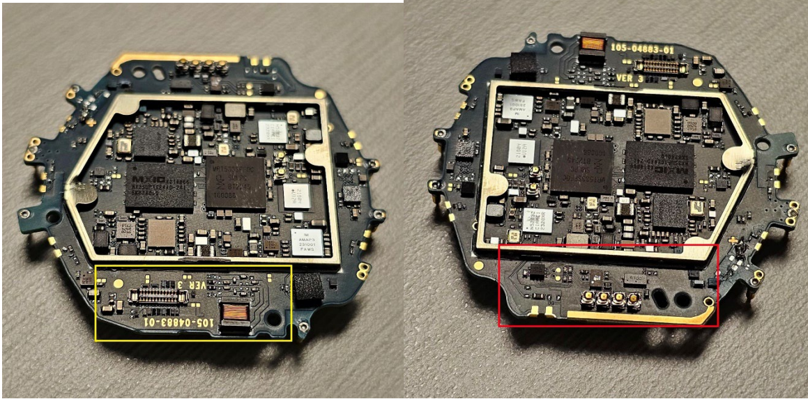
13.56 MHz (Yellow) and 2.4 GHz (RED)
