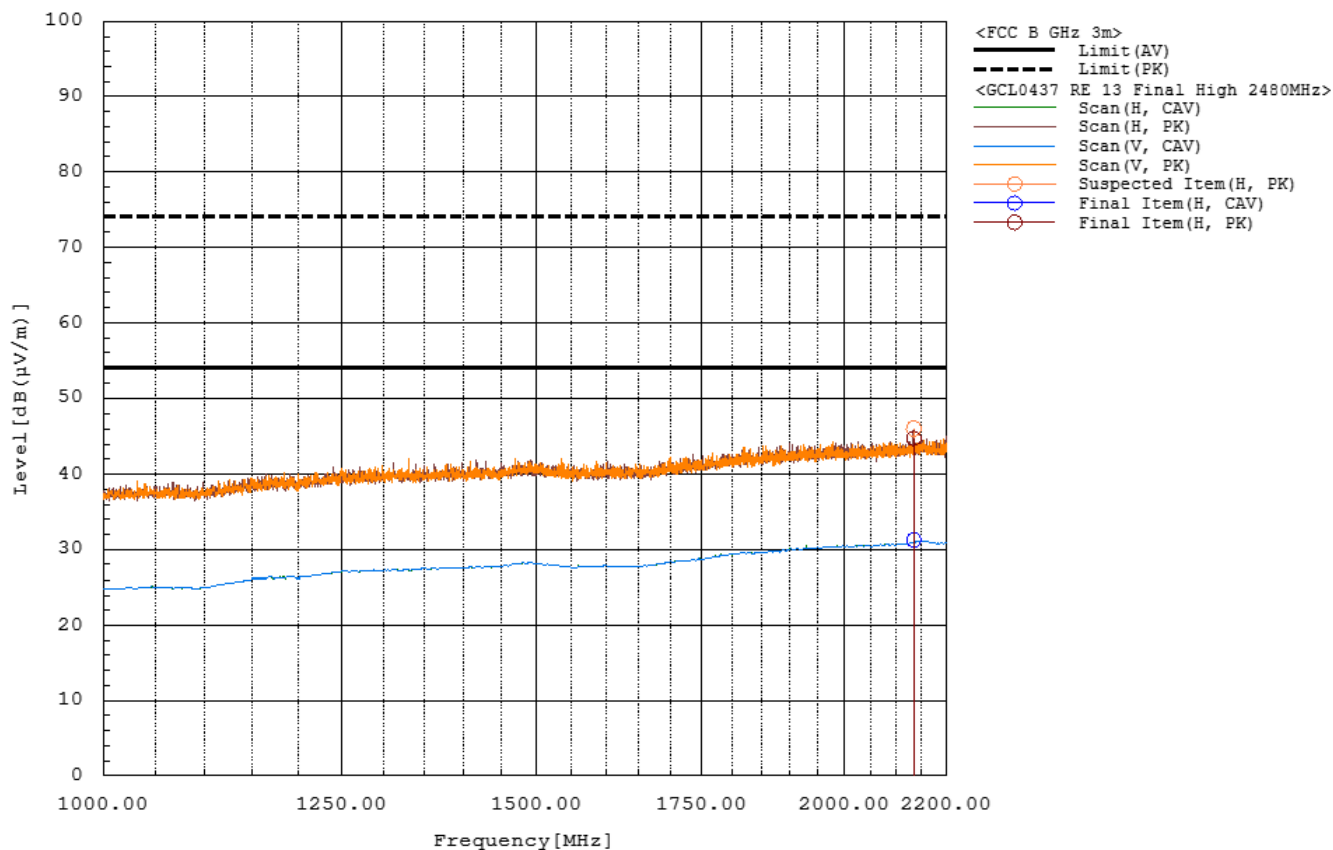
Figure RE06.3: Spectral data (2480MHz)
