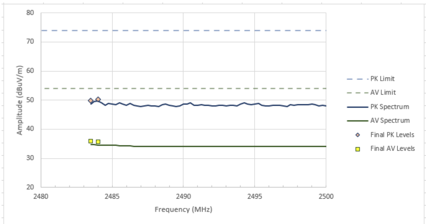
Figure RE03.4: FCC restricted band spectral data from 2483.5 to 2500 MHz (2Mb)
