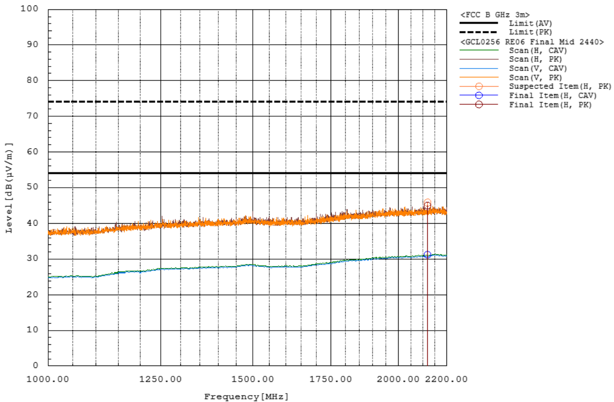
Figure RE06.2: Spectral data (2440MHz)
