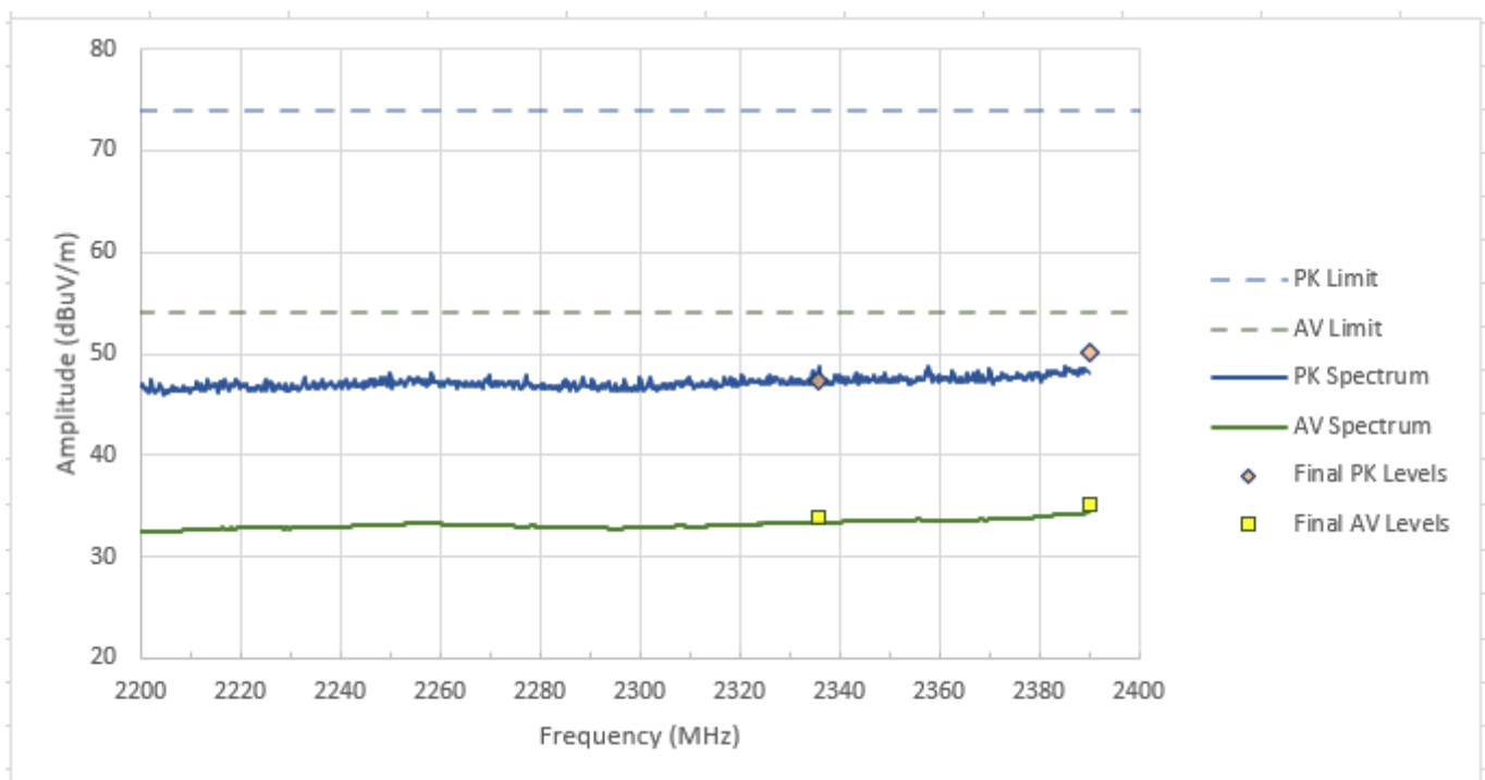
Figure RE03.3: FCC restricted band spectral data from 2200 to 2390 MHz (2Mb)
