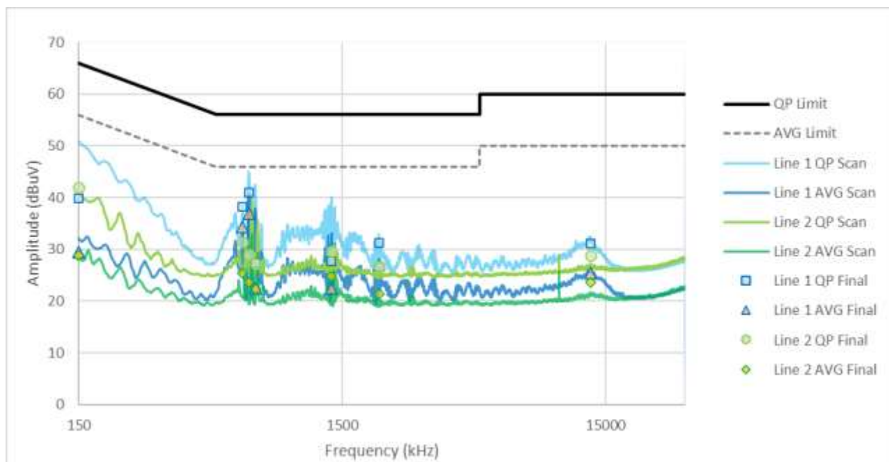
Figure CE01.1: Spectral data
