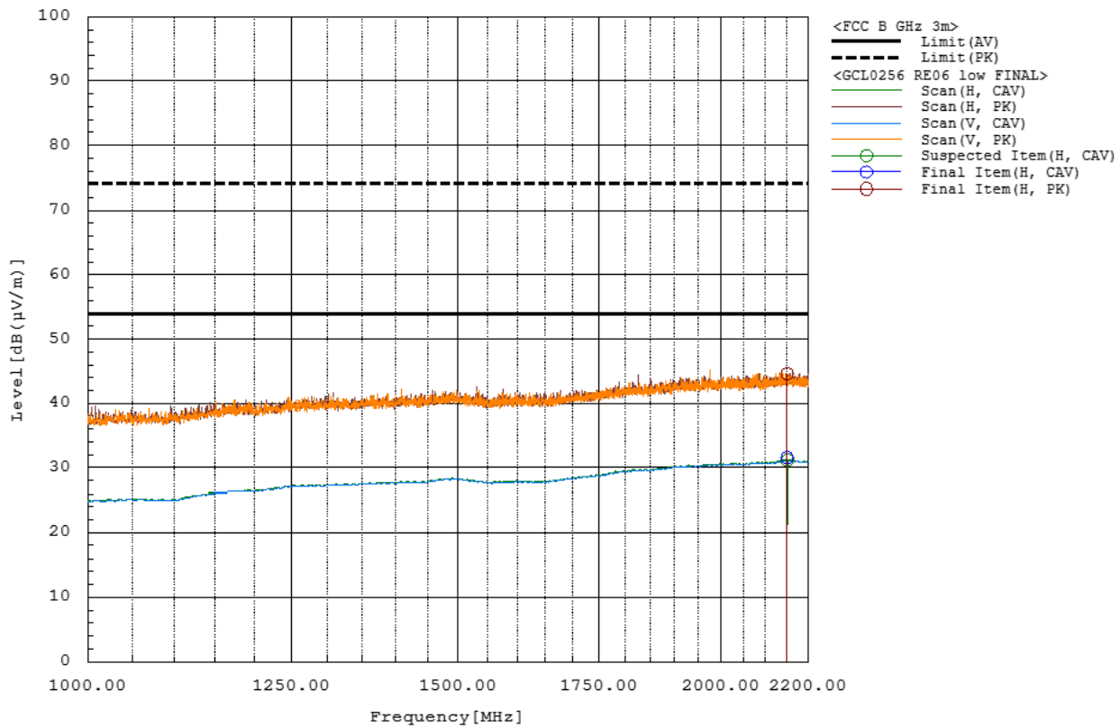
Figure RE06.1: Spectral data (2402MHz)
