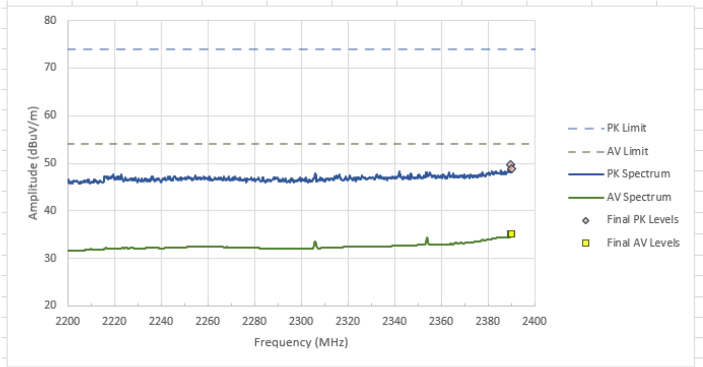
Figure RE03.1: FCC restricted band spectral data from 2200 to 2390 MHz (1Mb)
