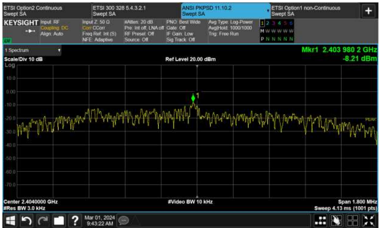
Figure TR35.3: Test data for BLE 2 Mbps, 2404 MHz.
