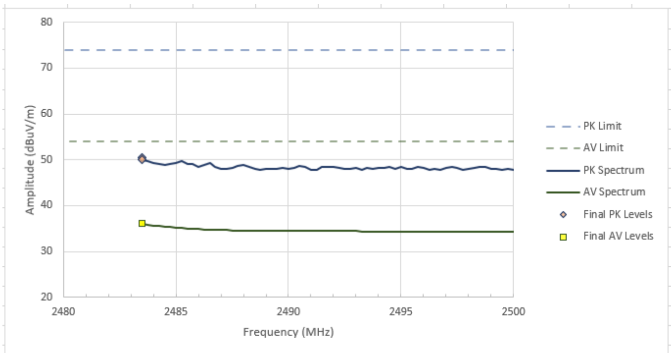
Figure RE03.2: FCC restricted band spectral data from 2483.5 to 2500 MHz (1Mb)
