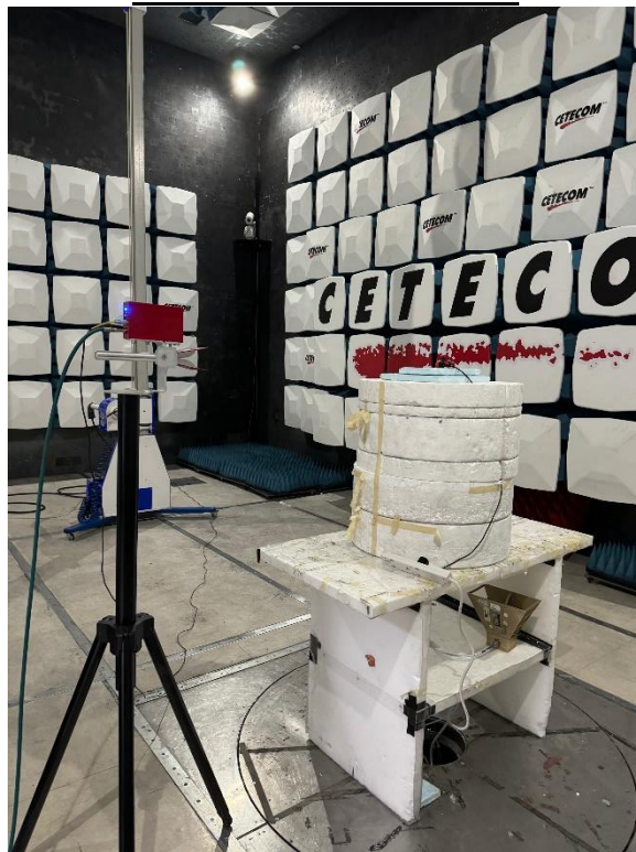
18 GHz to 26 GHz Rear View
