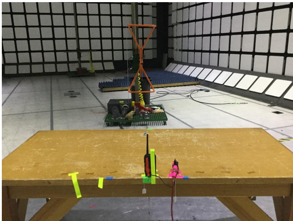
30 MHz-1 GHz – Z-axis
