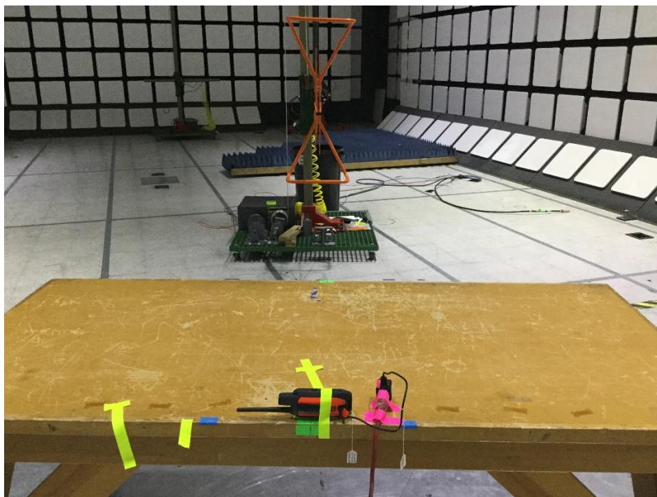
30 MHz-1 GHz – Y-axis
