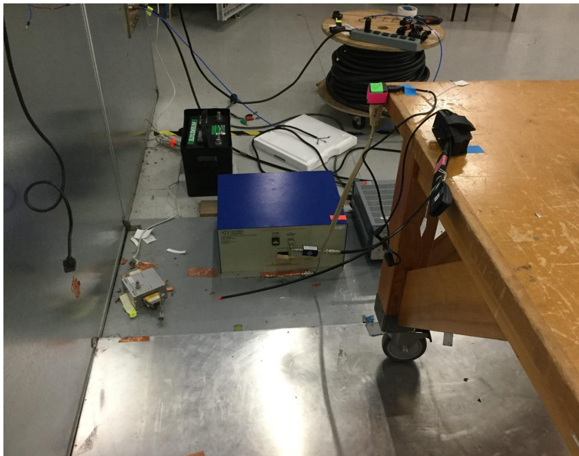
Conducted Emissions
