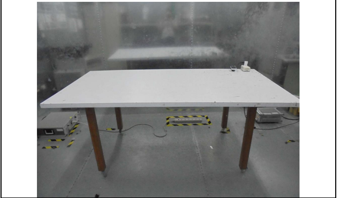
Conducted Emission Test ( Power mount mode )
