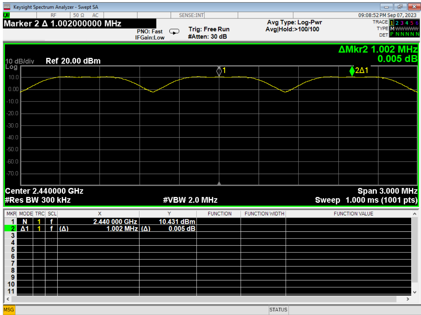
15 Frequency Separation
