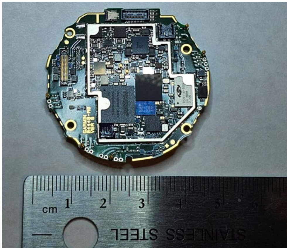
PCB Top (unshielded)
