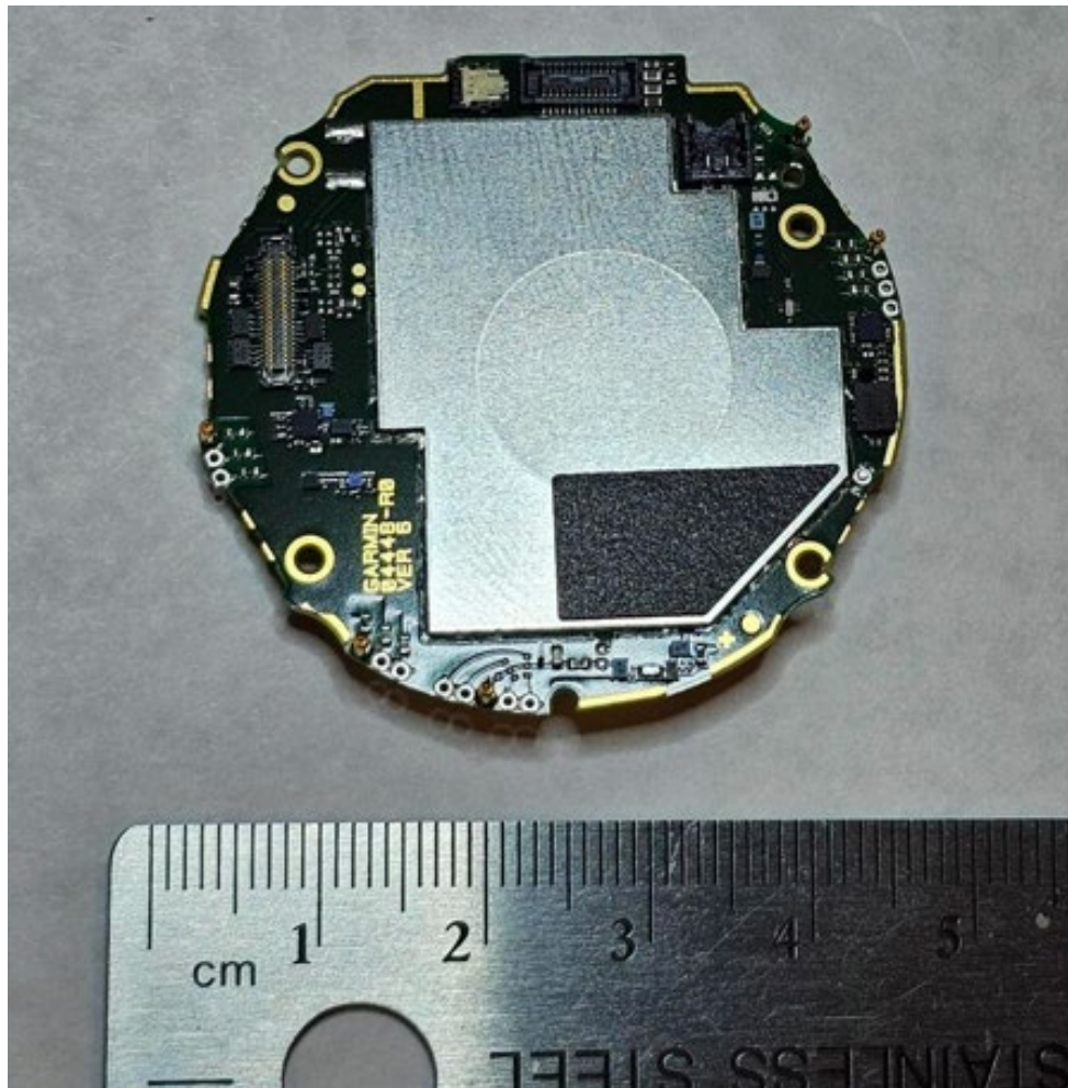
PCB Top (Shielded)
