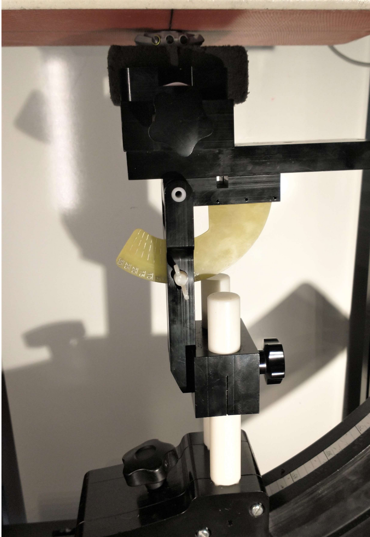
Figure C.1 – Photo – Setup: Extremity, DUT Back
