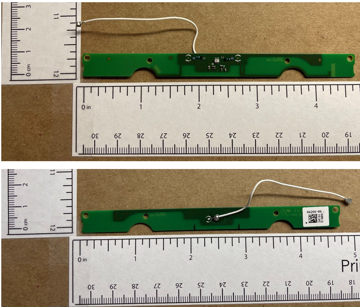
GNSS Receiver Antenna (Common to both models)
