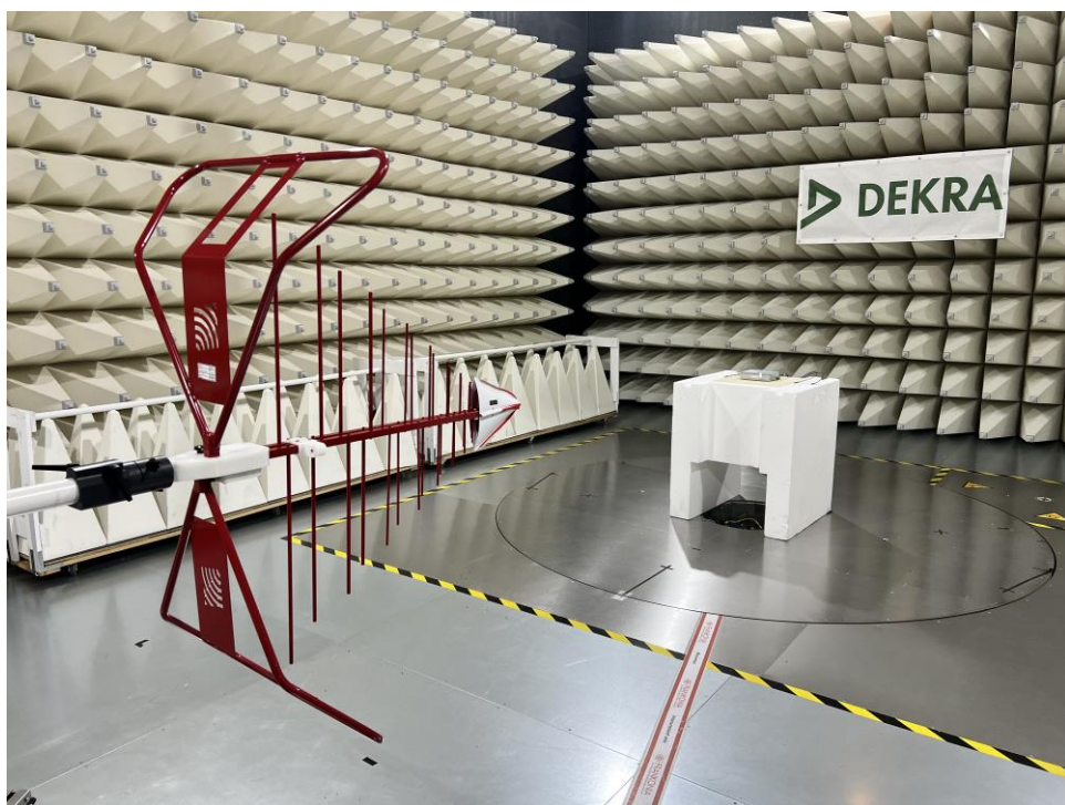
Figure B6. Low Range Radiated Emission test setup
