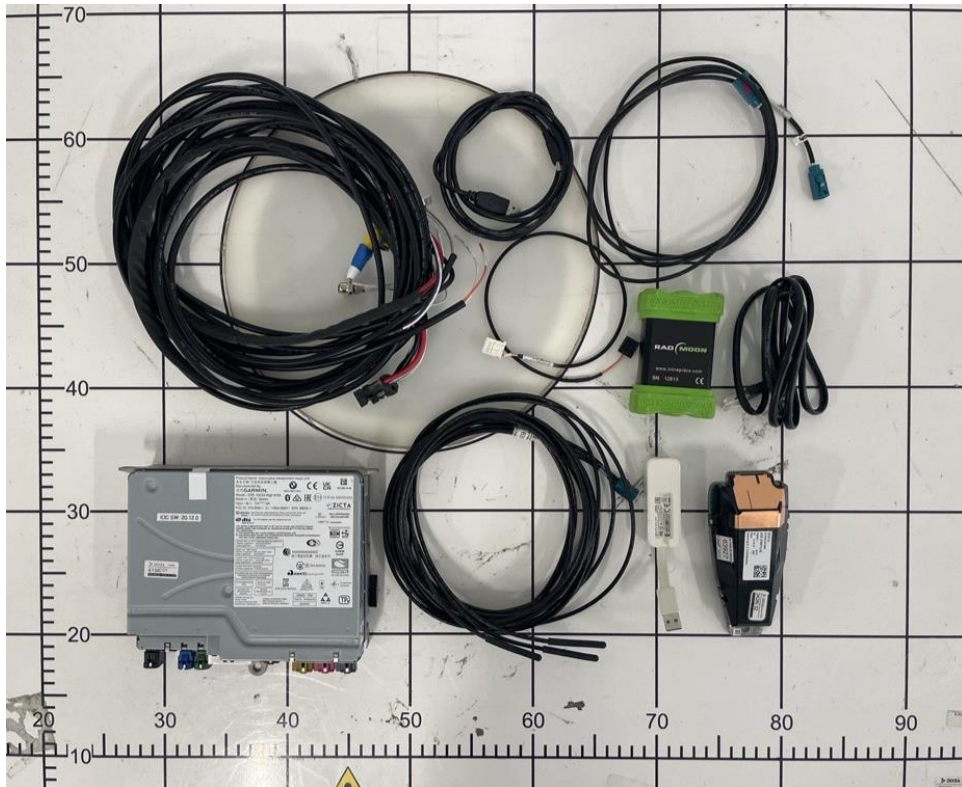
Figure B5. Front View of DUT with Accessories
