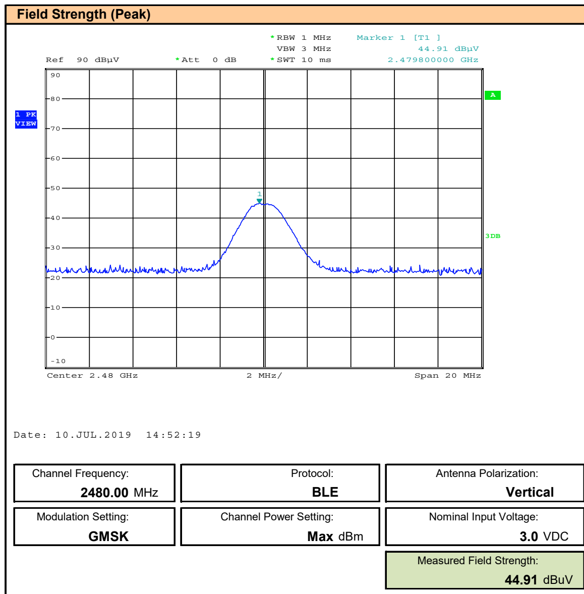
Plot 10.23 – Field Strength, BLE, 2480MHz, Vertical, Peak
