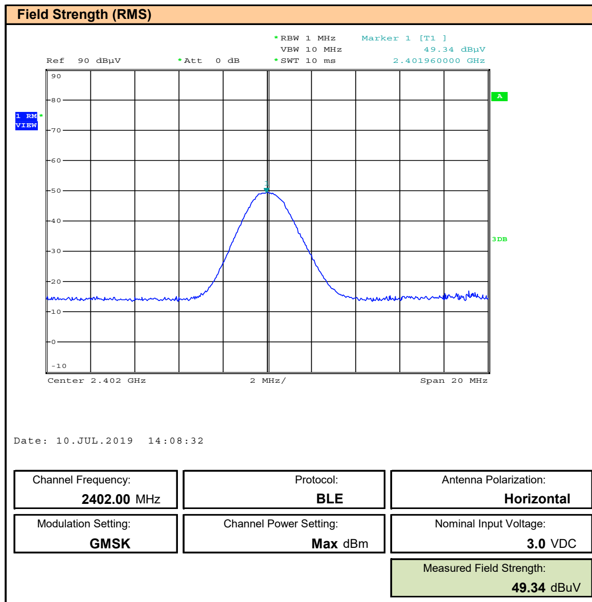
Plot 10.14 – Field Strength, BLE, 2402MHz, Horizontal, RMS
