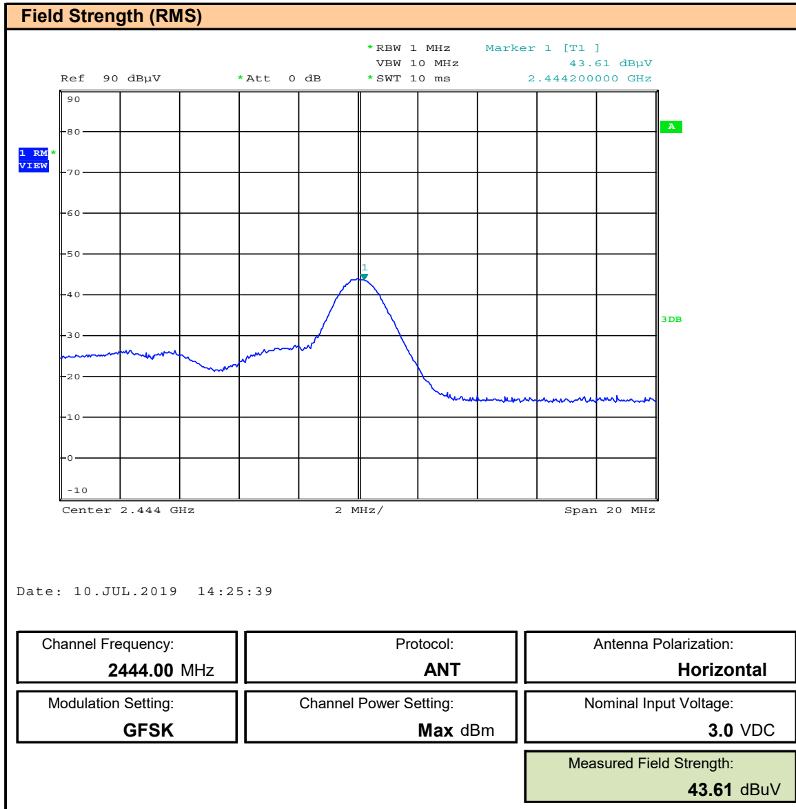
Plot 10.6 – Field Strength, ANT, 2444MHz, Horizontal, RMS
