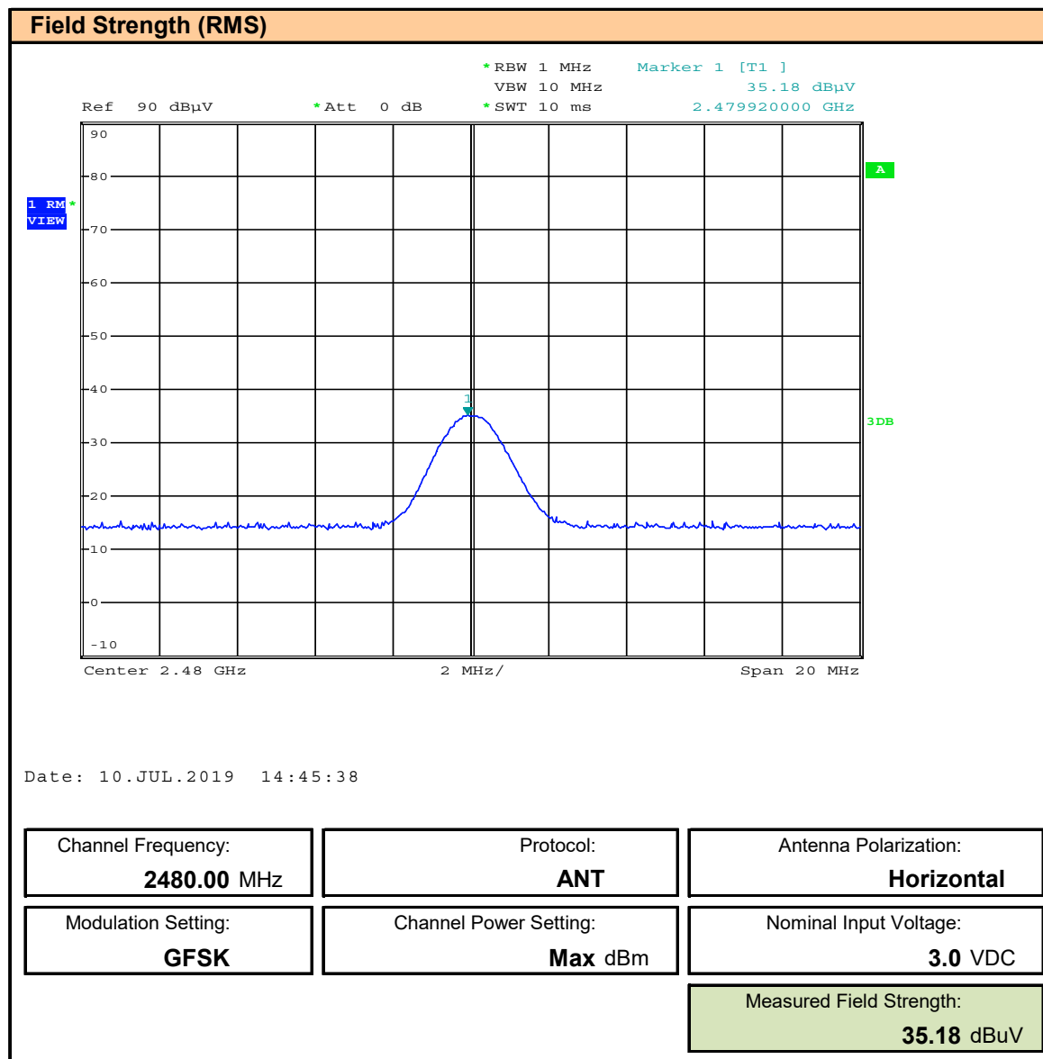
Plot 10.10 – Field Strength, ANT, 2480MHz, Horizontal, RMS
