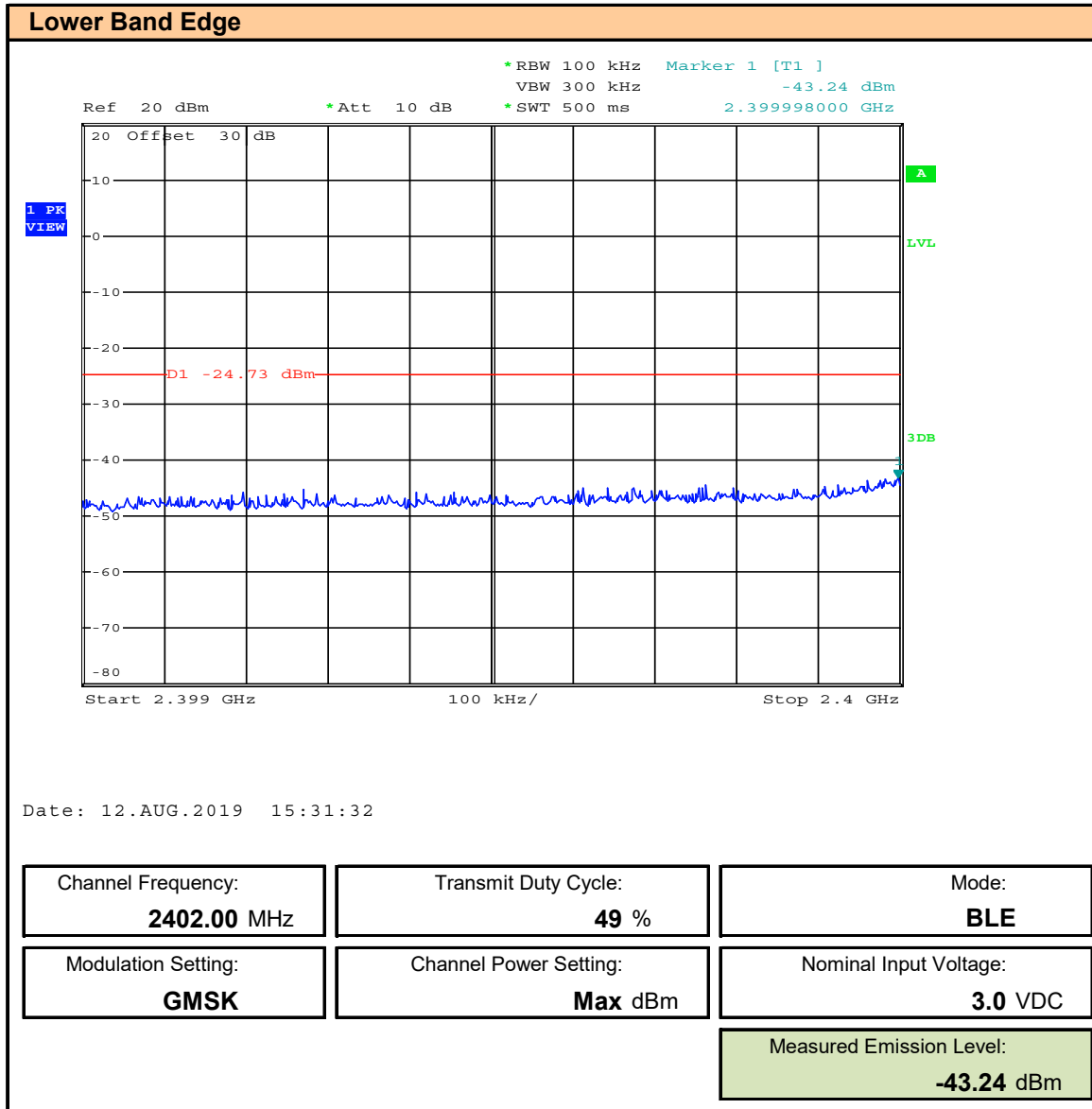
Plot 11.3 – 2402MHz, BLE, Lower Band Edge
