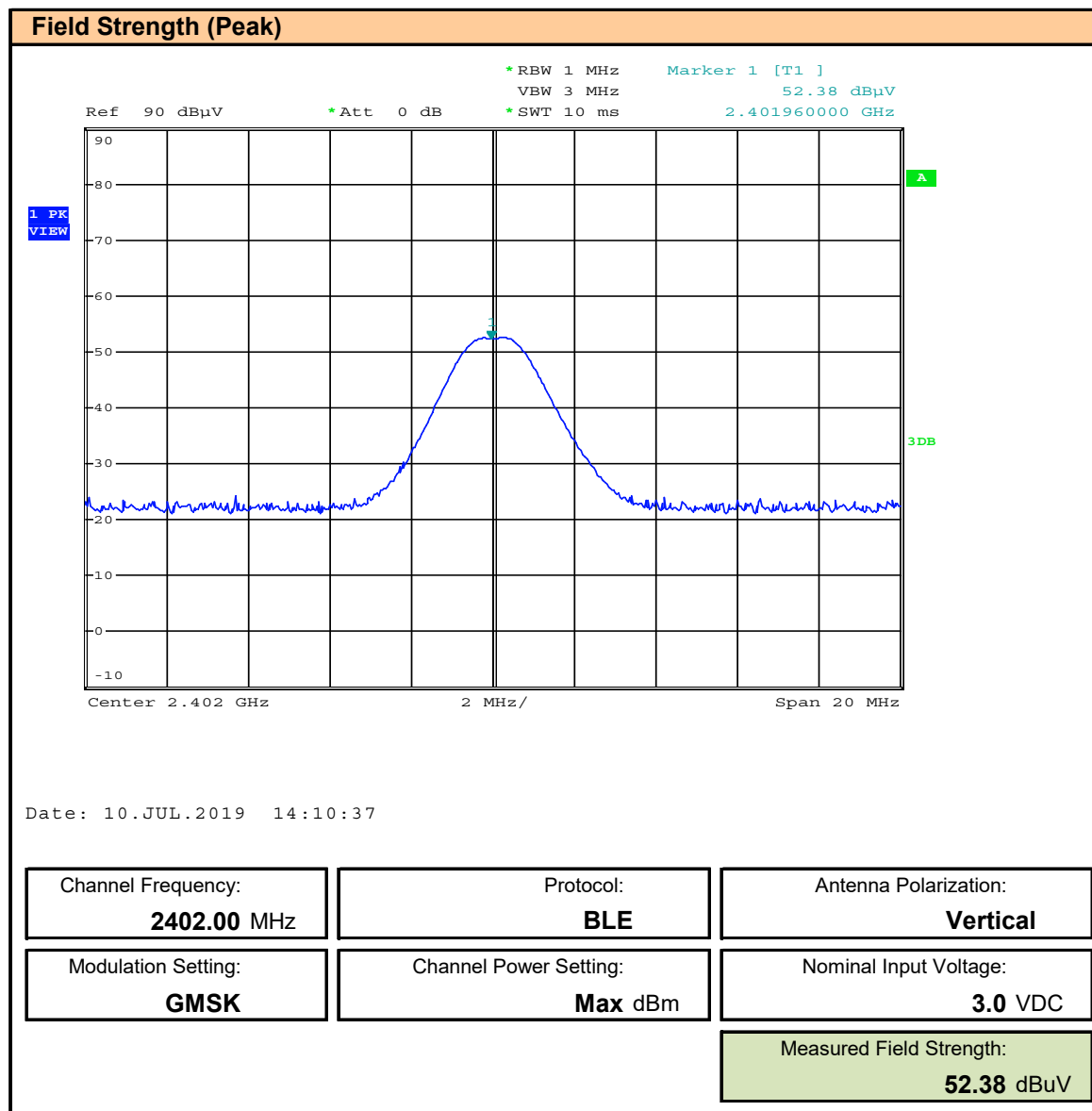
Plot 10.15 – Field Strength, BLE, 2402MHz, Vertical, Peak
