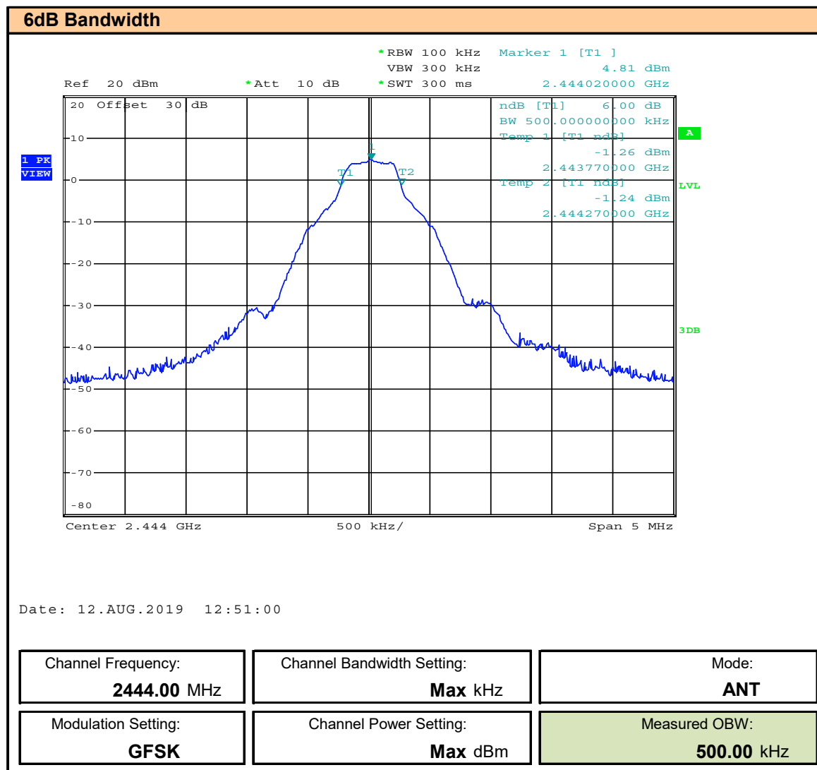
Plot 9.2 – 6dB Bandwidth, 2444MHz, ANT
