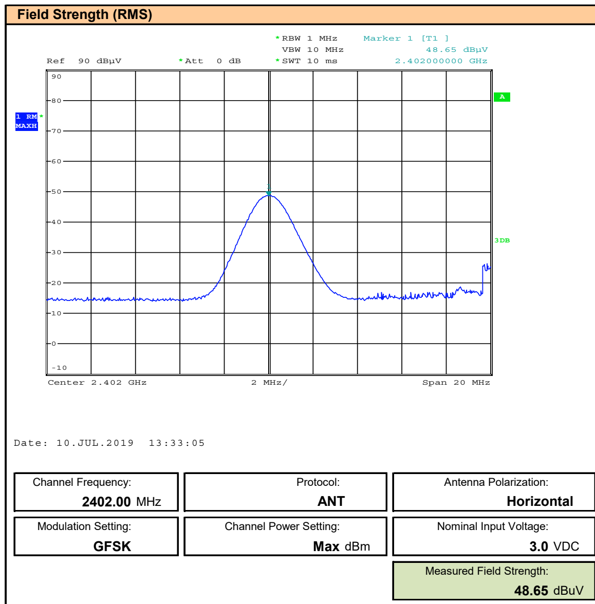
Plot 10.2 – Field Strength, ANT, 2402MHz, Horizontal, RMS
