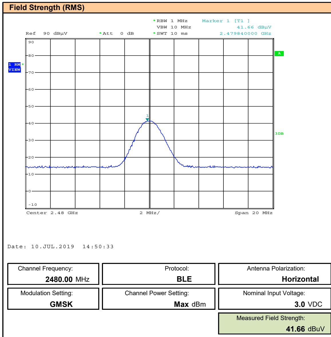
Plot 10.22 – Field Strength, BLE, 2480MHz, Horizontal, RMS
