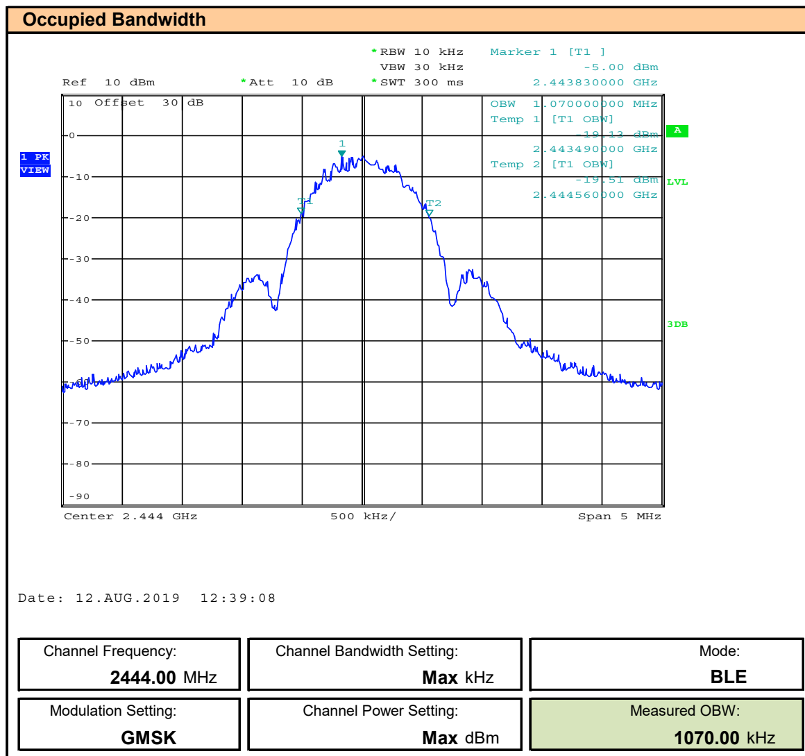
Plot 8.5 – Occupied Bandwidth – 2444MHz, BLE
