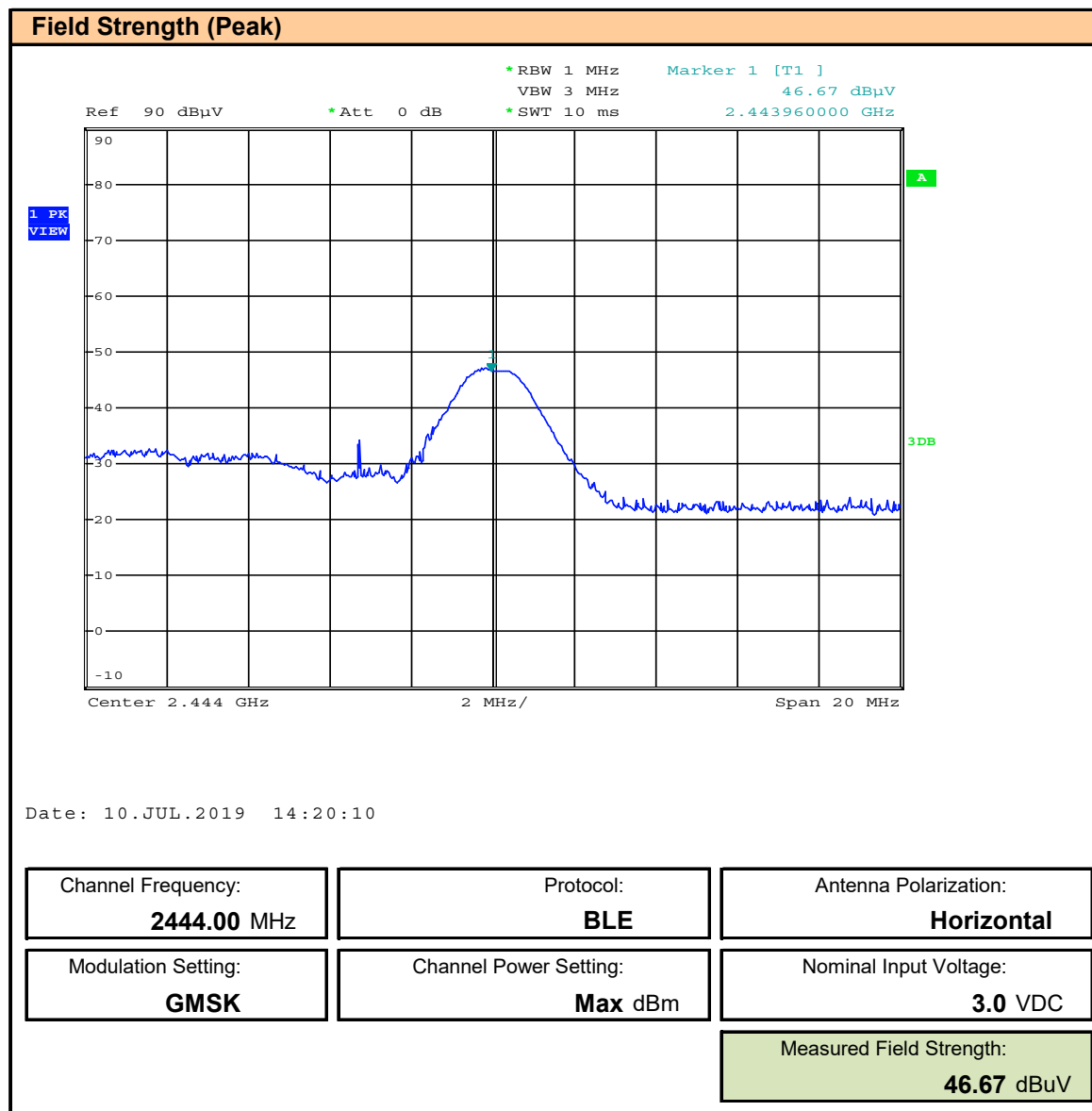
Plot 10.17 – Field Strength, BLE, 2444MHz, Horizontal, Peak
