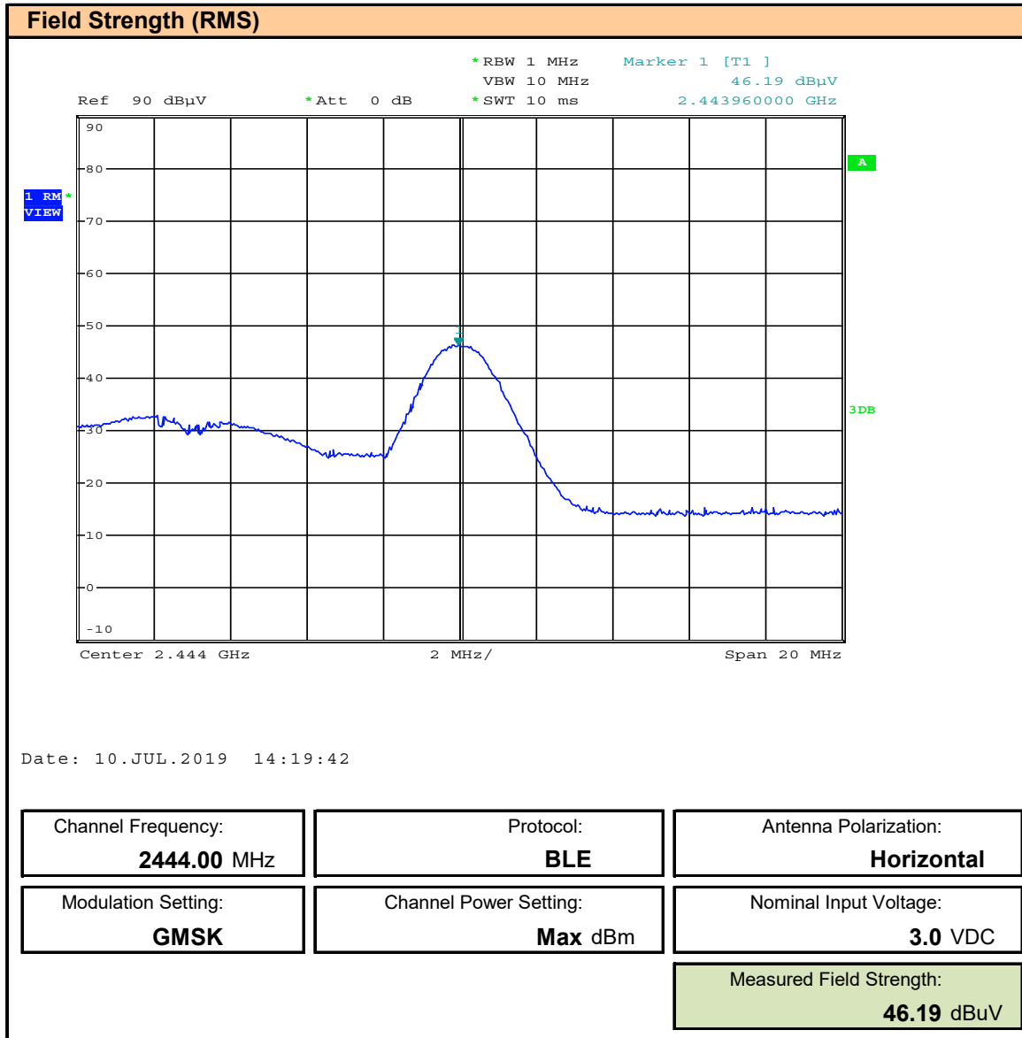
Plot 10.18 – Field Strength, BLE, 2444MHz, Horizontal, RMS
