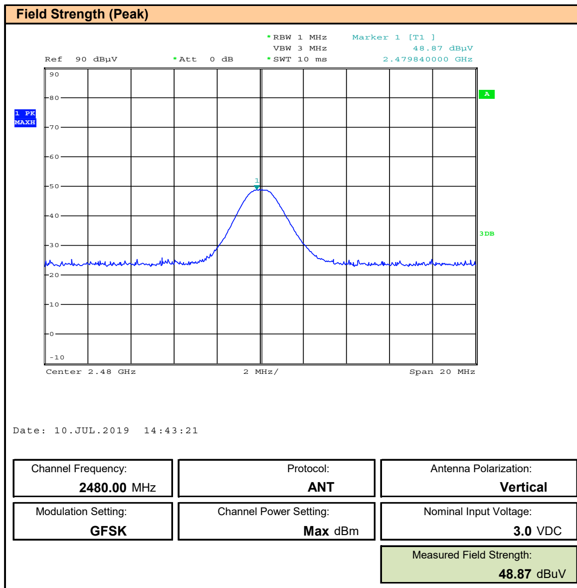
Plot 10.11 – Field Strength, ANT, 2480MHz, Vertical, Peak
