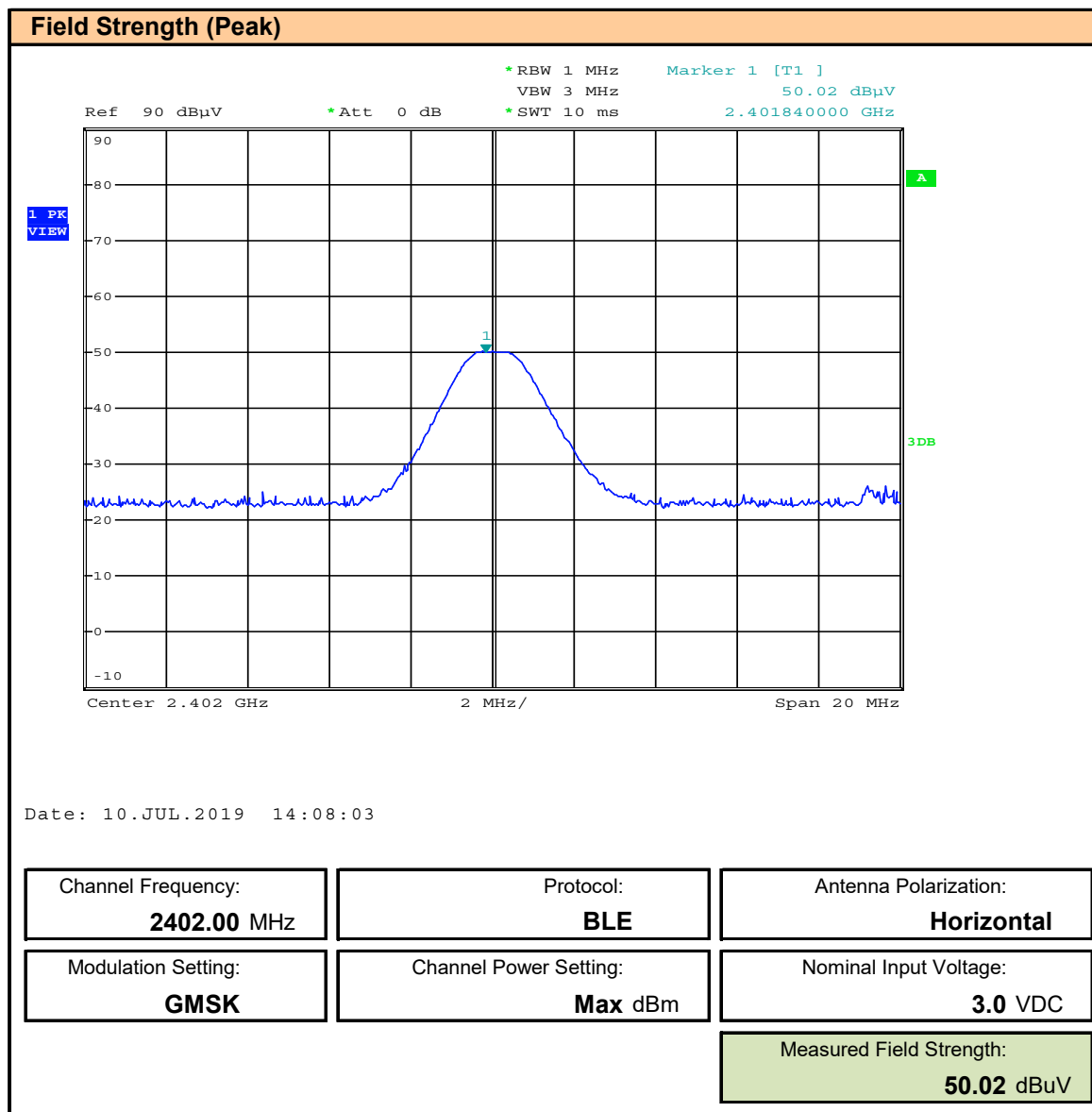
Plot 10.13 – Field Strength, BLE, 2402MHz, Horizontal, Peak
