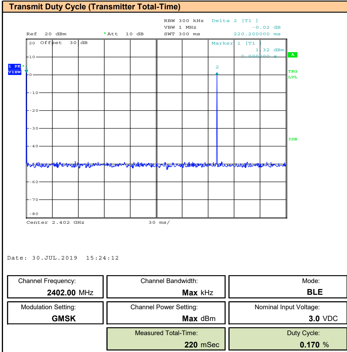
Plot 7.4 – Duty Cycle – Normal Operation, BLE, Total-Time
