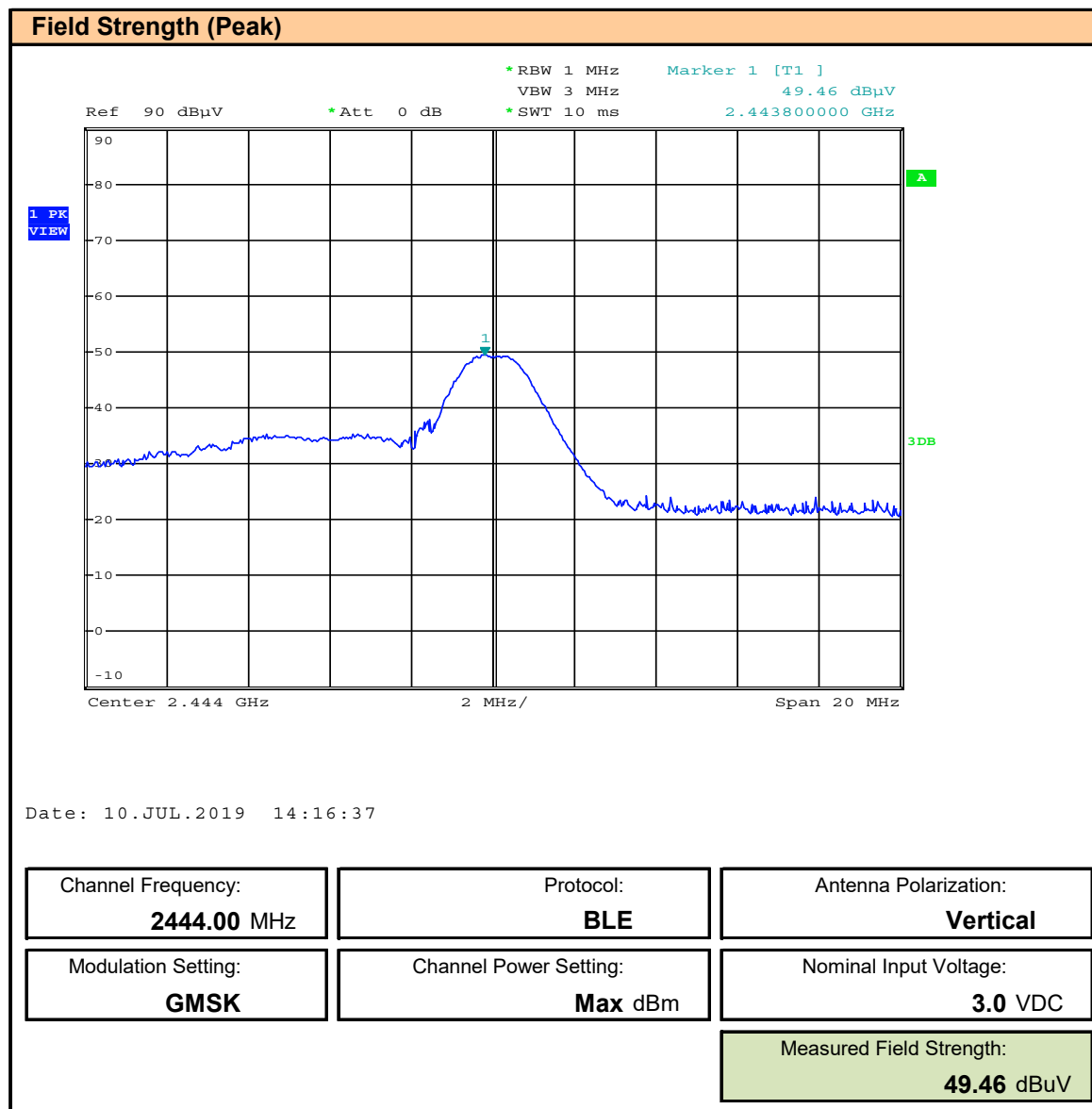
Plot 10.19 – Field Strength, BLE, 2444MHz, Vertical, Peak
