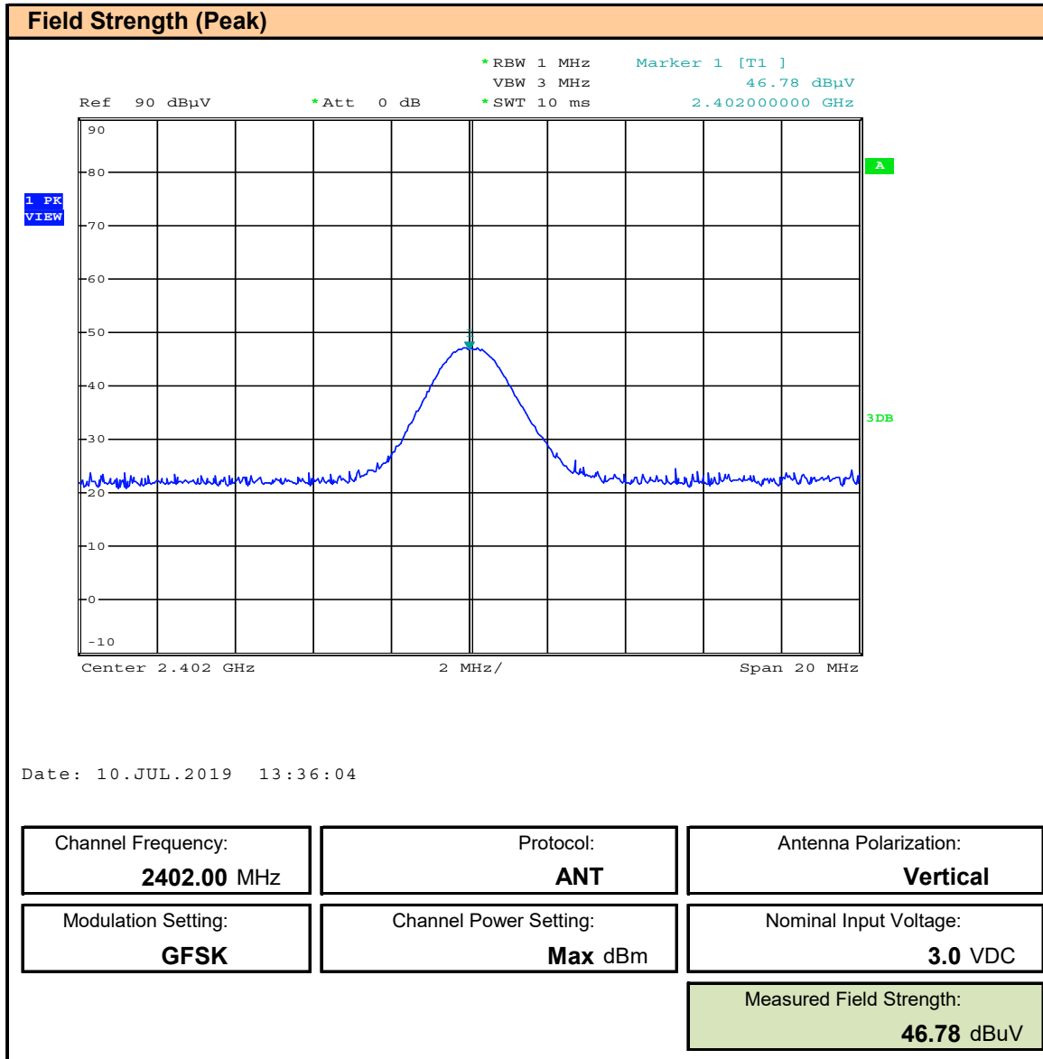
Plot 10.3 – Field Strength, ANT, 2402MHz, Vertical, Peak
