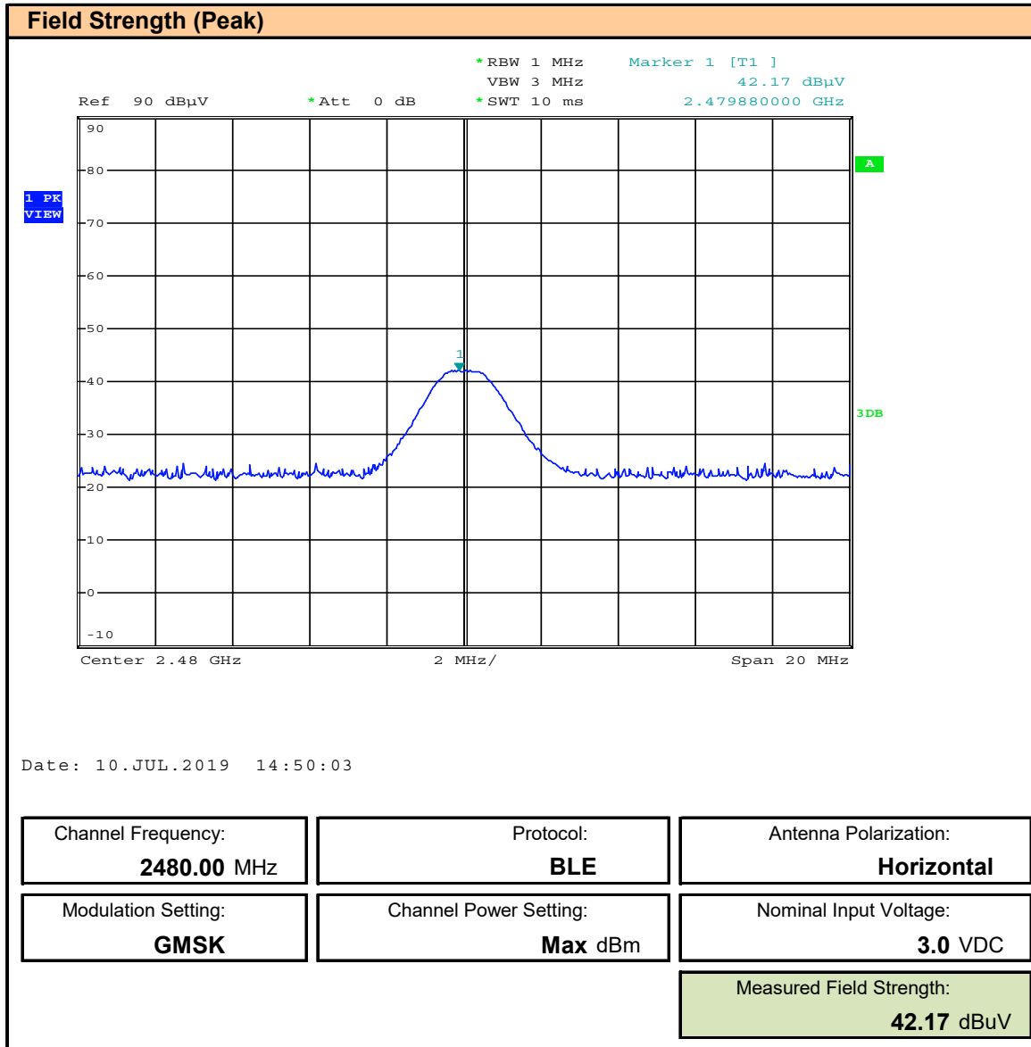
Plot 10.21 – Field Strength, BLE, 2480MHz, Horizontal, Peak
