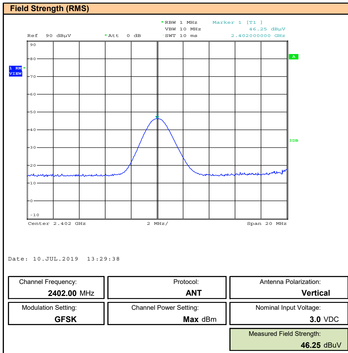
Plot 10.4 – Field Strength, ANT, 2402MHz, Vertical, RMS
