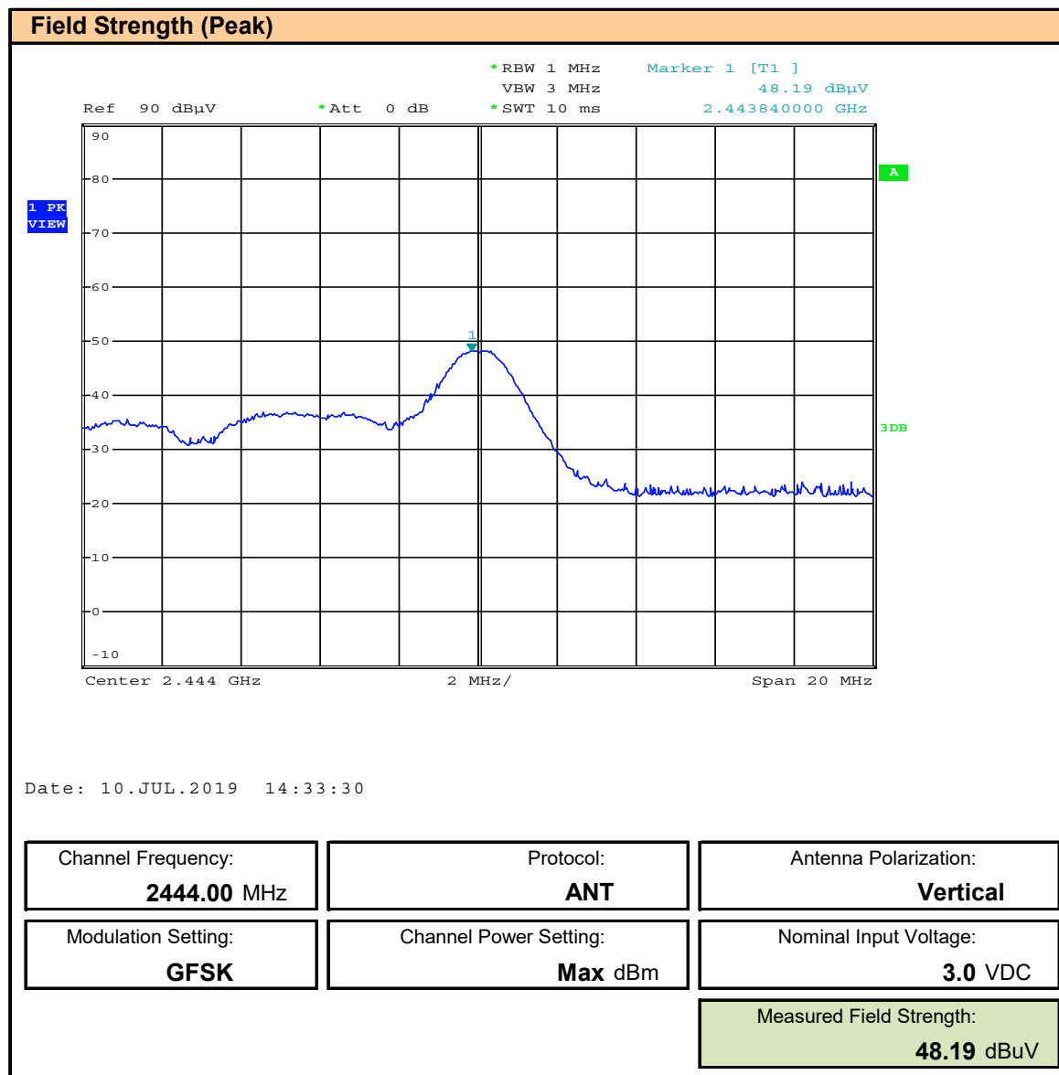
Plot 10.7 – Field Strength, ANT, 2444MHz, Vertical, Peak
