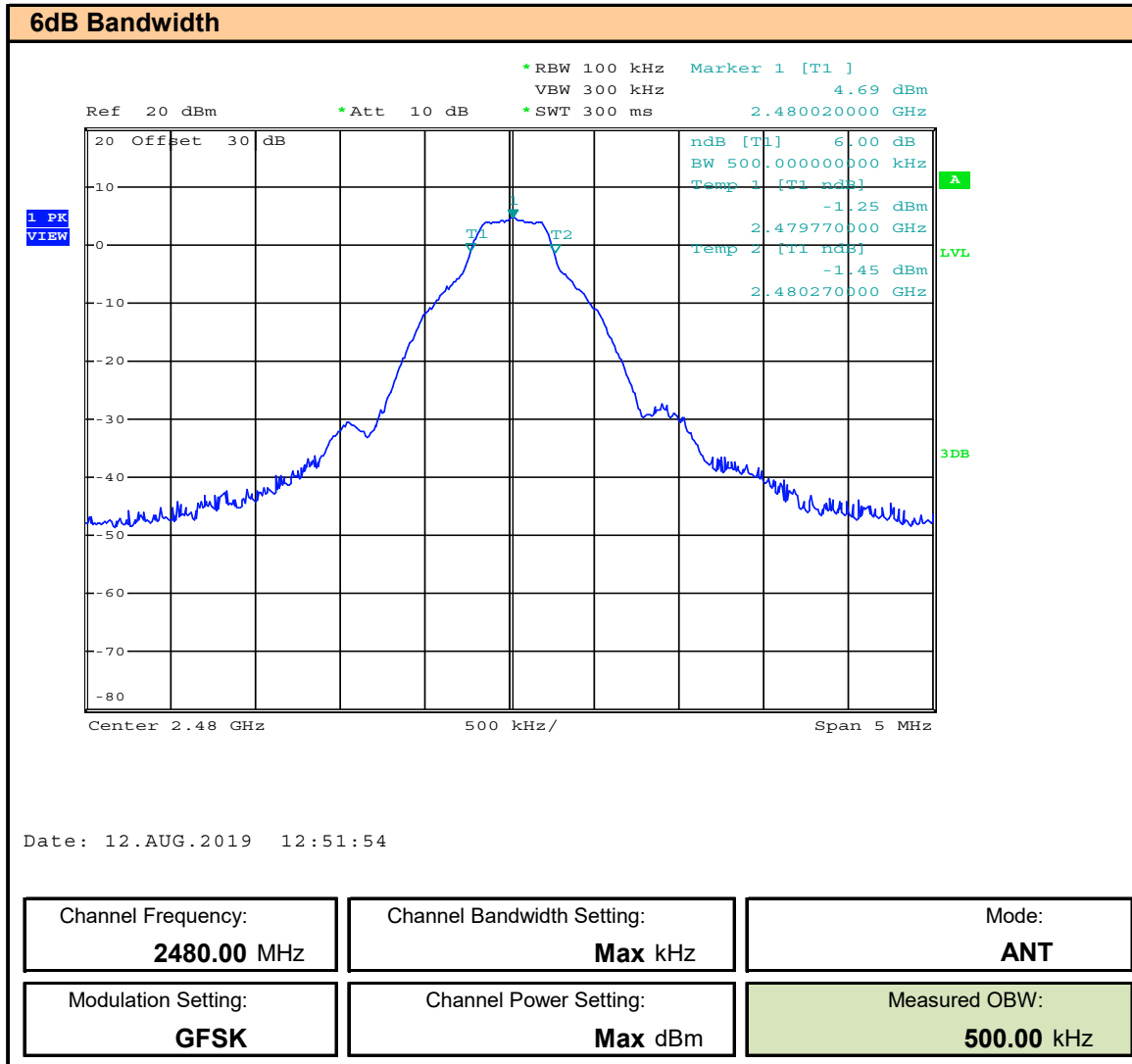
Plot 9.3 – 6dB Bandwidth, 2480MHz, ANT
