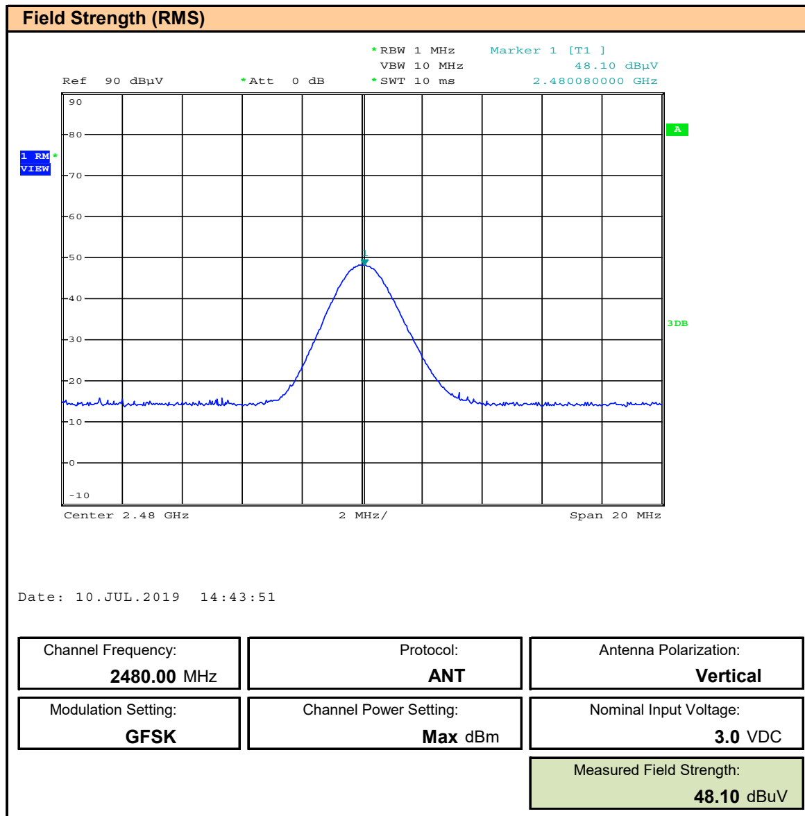
Plot 10.12 – Field Strength, ANT, 2480MHz, Vertical, RMS
