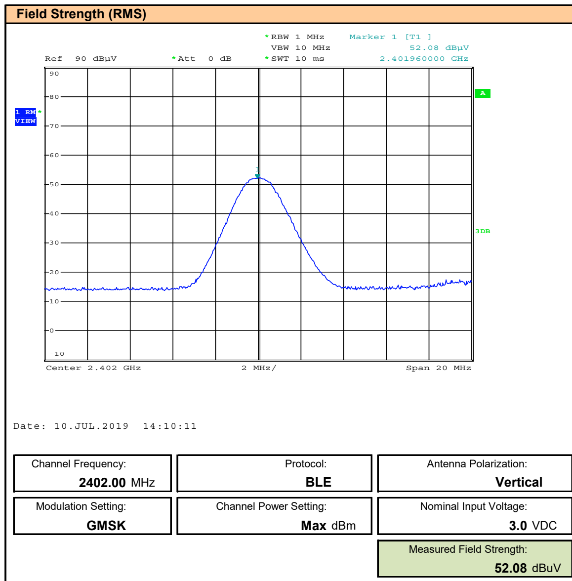
Plot 10.16 – Field Strength, BLE, 2402MHz, Vertical, RMS
