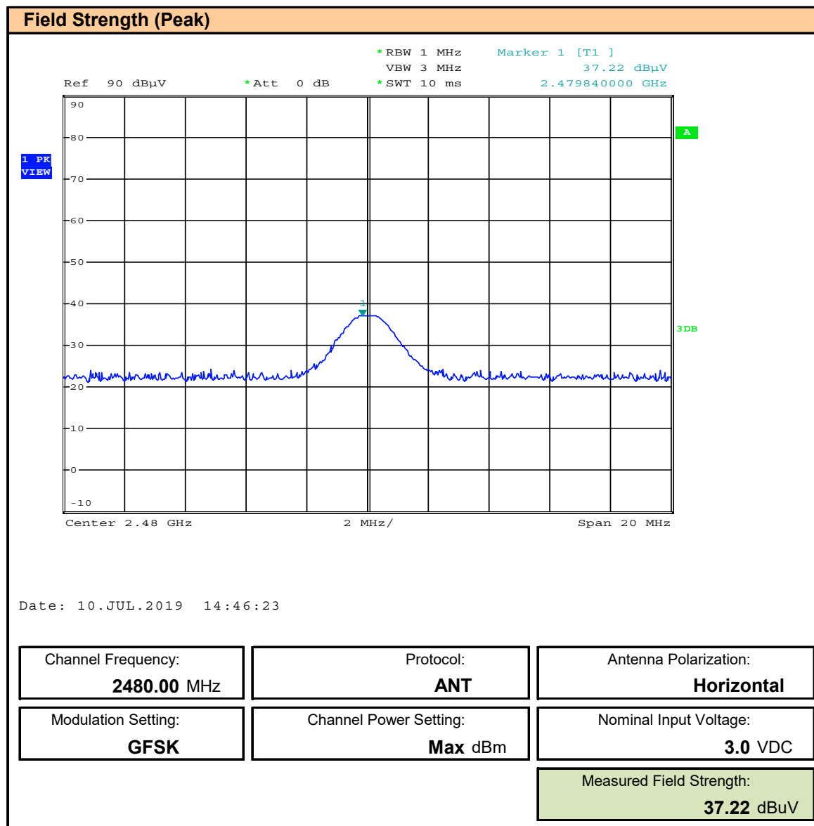
Plot 10.9 – Field Strength, ANT, 2480MHz, Horizontal, Peak
