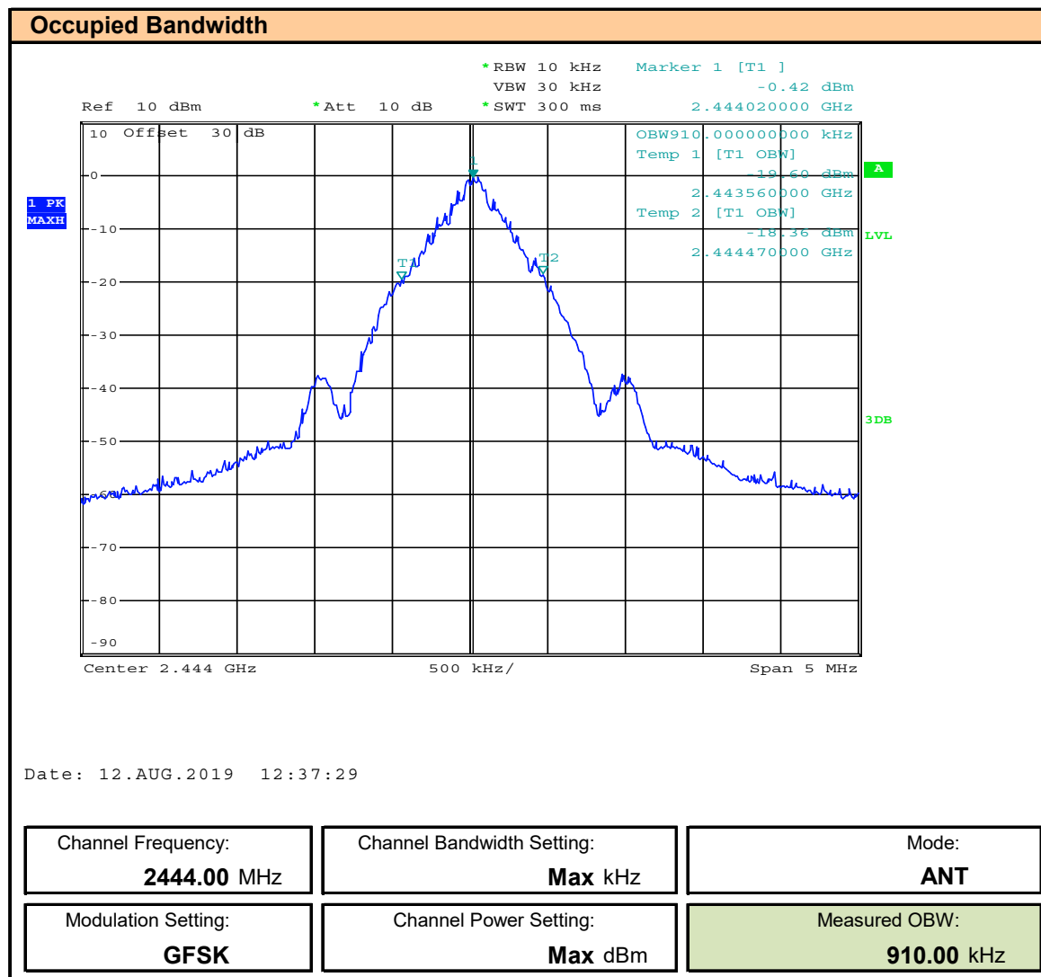
Plot 8.2 – Occupied Bandwidth – 2444MHz, ANT
