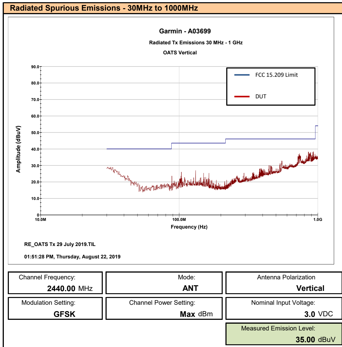
Plot 12.4 – Spurious Emissions - 30MHz – 1000MHz, Vertical
