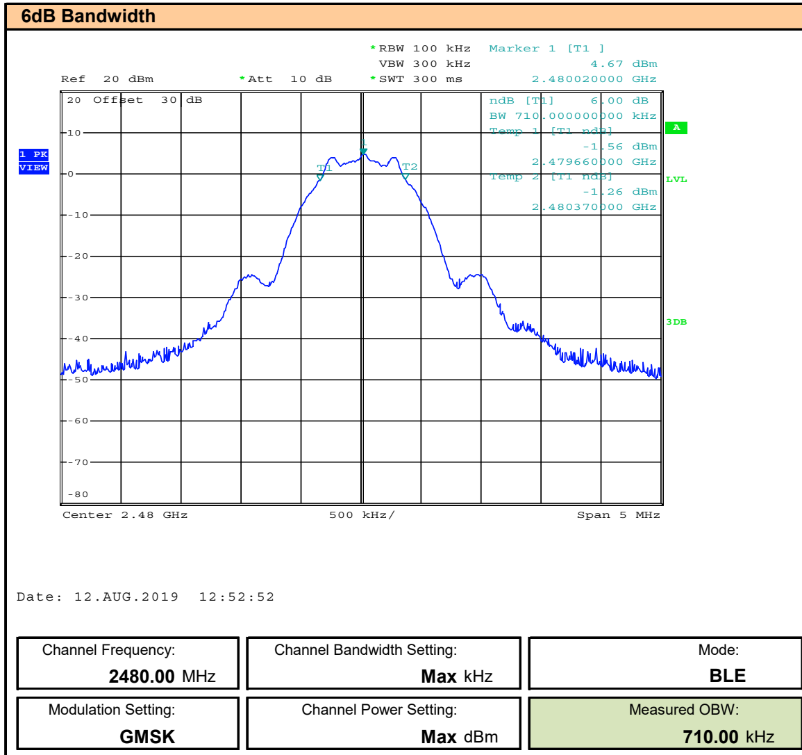
Plot 9.6 – 6dB Bandwidth, 2480MHz, BLE
