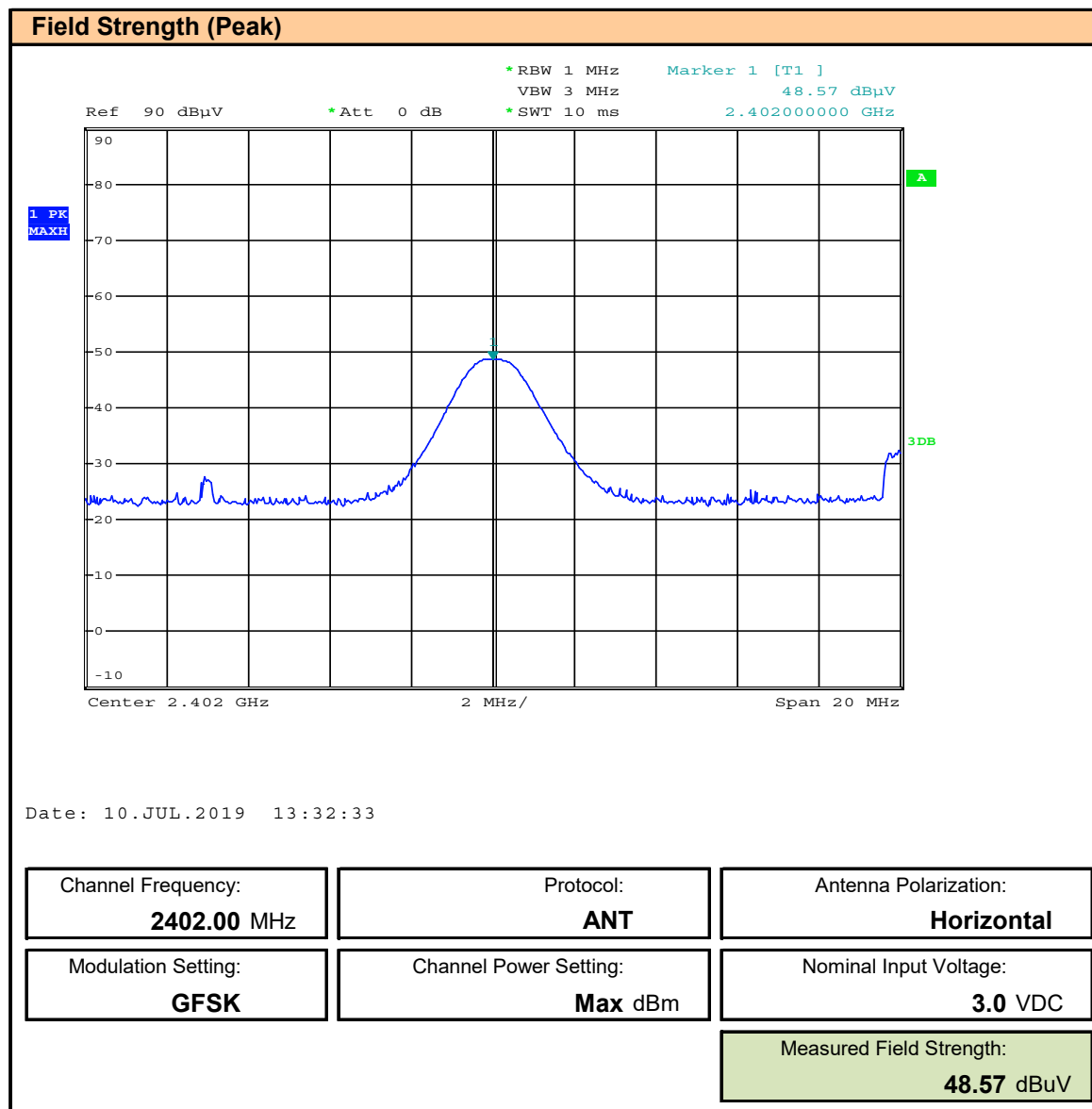
Plot 10.1 – Field Strength, ANT, 2402MHz, Horizontal, Peak
