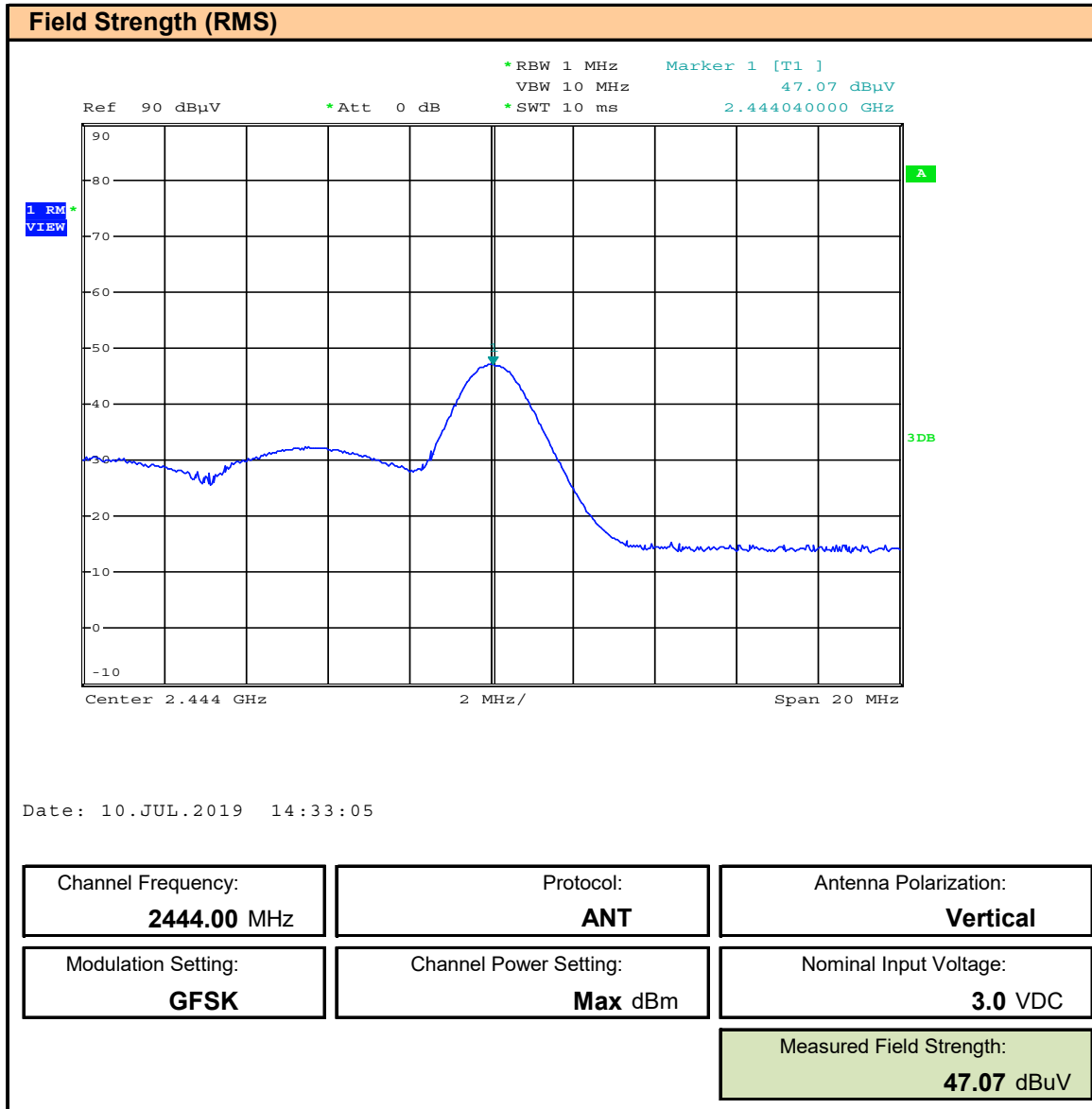
Plot 10.8 – Field Strength, ANT, 2444MHz, Vertical, RMS
