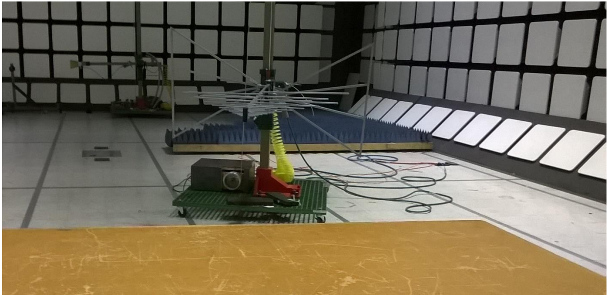
Figure 1 - Radiated Emissions test Setup, 30 MHz - 1 GHz, EUT not shown
