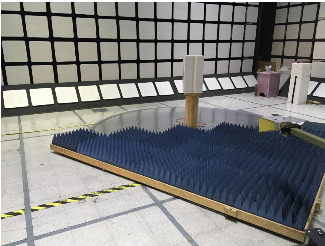
Figure 2 - Radiated Emissions test Setup, 1 GHz - 25 GHz, EUT not shown
