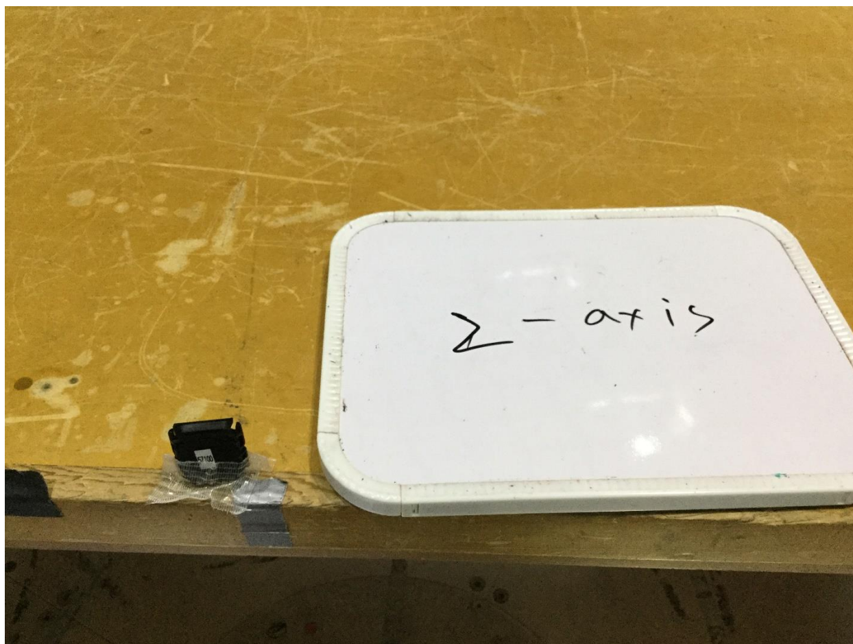
Figure 3 - Radiated Emissions test Setup, 30 MHz - 1 GHz
