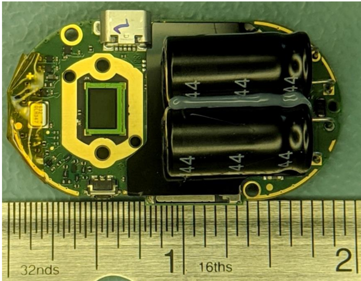
Front of PCB with lens removed
