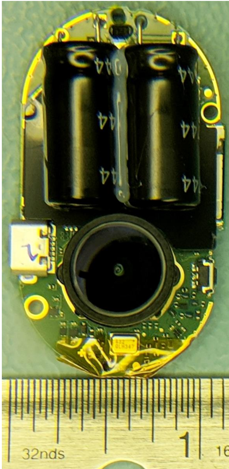
Front of PCB with lens
