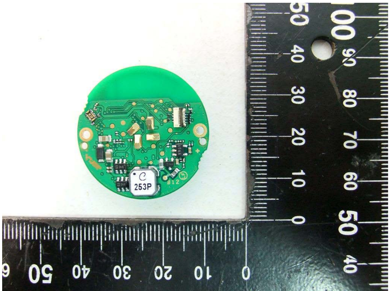
Figure 3 - PCB Bottom
