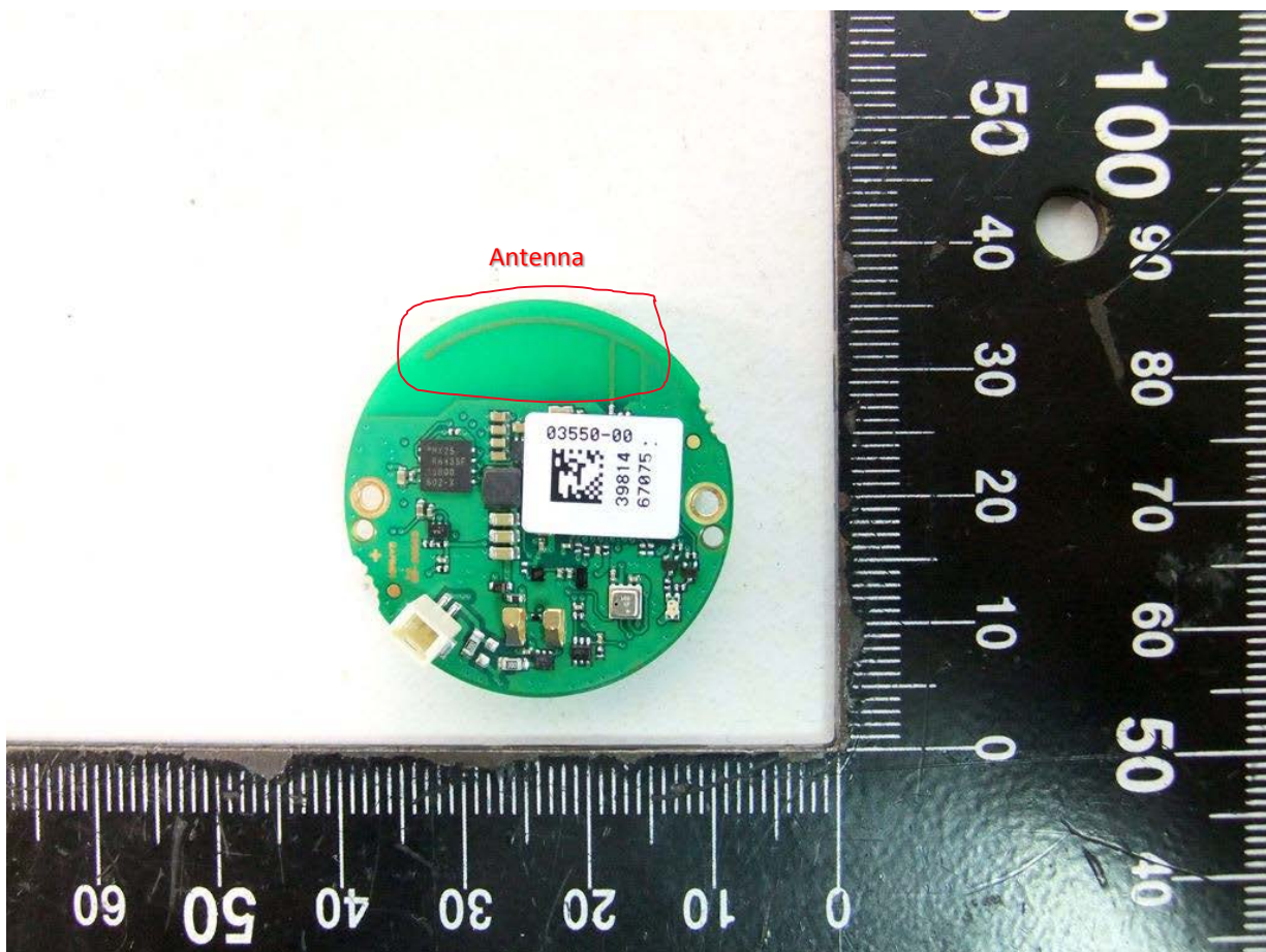
Figure 2 - PCB Top
