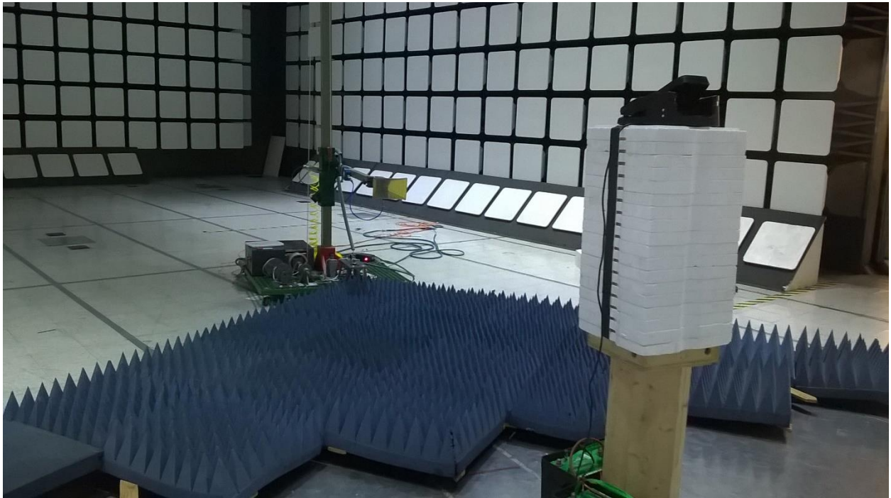
Radiated emissions test setup, 1 – 25 GHz
