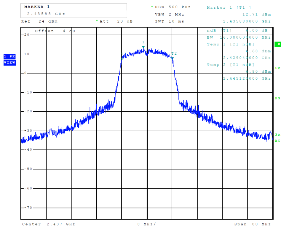
Figure 12 Plot of Transmitter 6-dB Occupied Bandwidth (802.11 g-mode)
