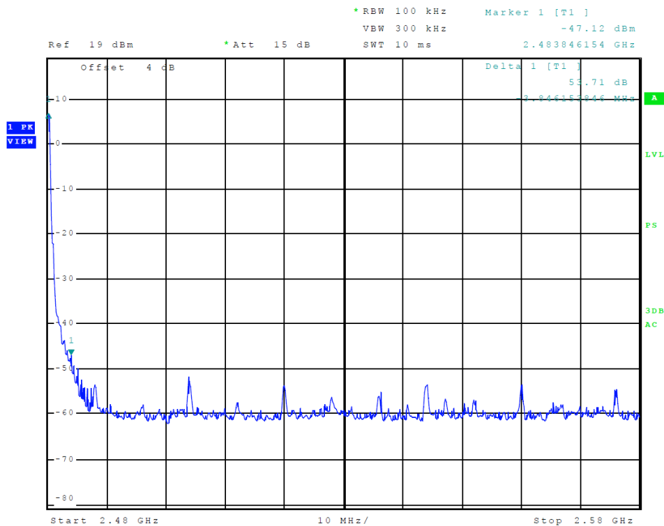
Figure 13 Plot of Transmitter Emissions (High Band Edge, BLE GMSK)
