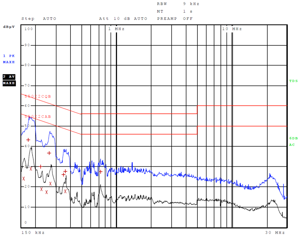
Figure 1 AC Line Conducted emissions of EUT line 1 (#2, EUT – AC Adapter)
