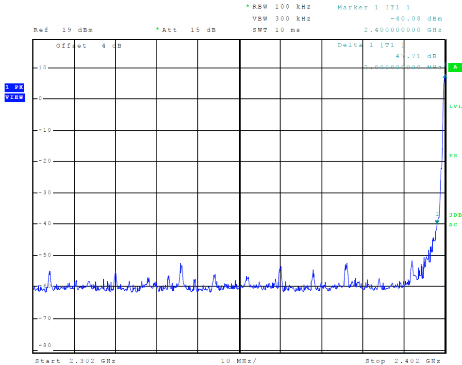
Figure 12 Plot of Transmitter Emissions (Low Band Edge, BLE GMSK)
