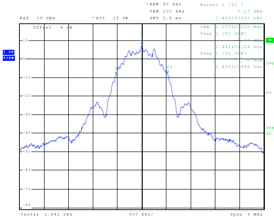
Figure 10 Plot of Transmitter Emissions (99% Occupied Bandwidth, BLE GMSK)
