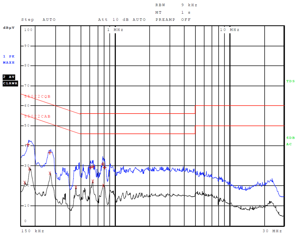
Figure 2 AC Line Conducted emissions of EUT line 2 (#2, EUT – AC Adapter)
