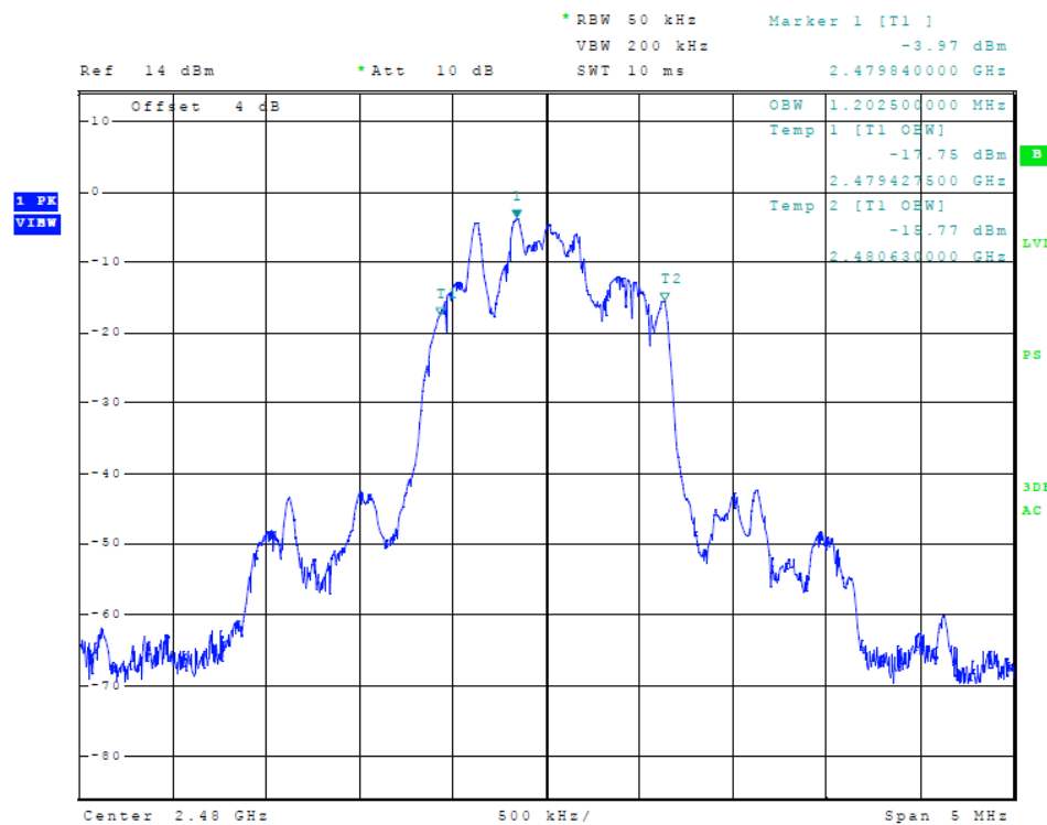
Figure 16 Plot of Transmitter Emissions (99% Occupied Bandwidth, 8-DPSK)
