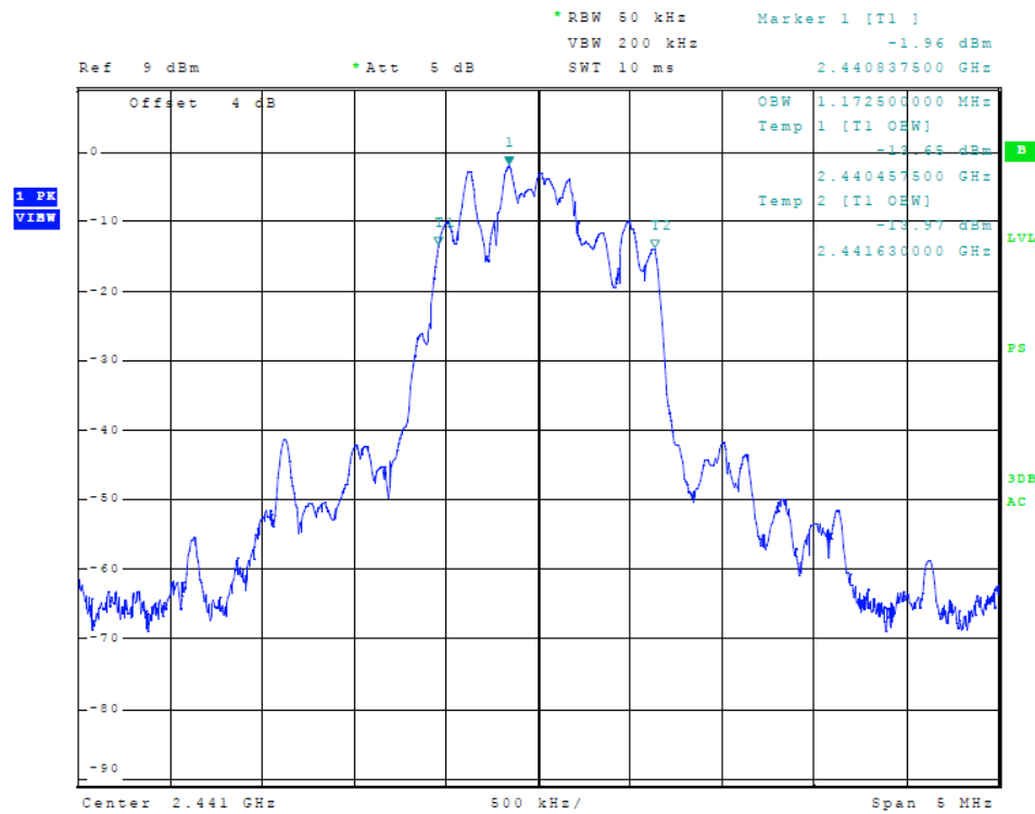
Figure 12 Plot of Transmitter Emissions (99% Occupied Bandwidth, \pi/4 DQPSK)
