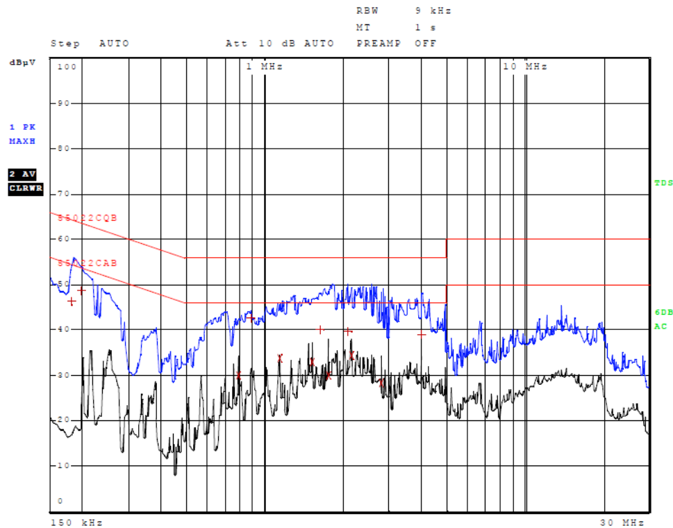
Figure 5 AC Line Conducted emissions of EUT line 1 (#3, EUT, USB CPU Adapter)
