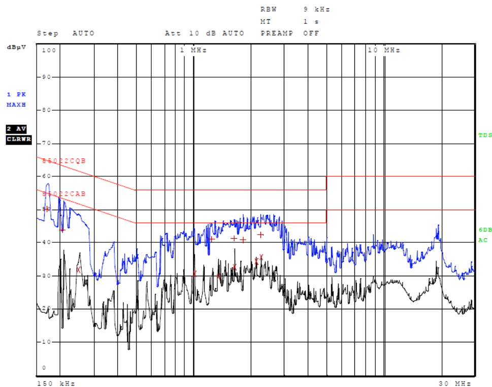
Figure 6 AC Line Conducted emissions of EUT line 2 (#3, EUT, USB CPU Adapter)
