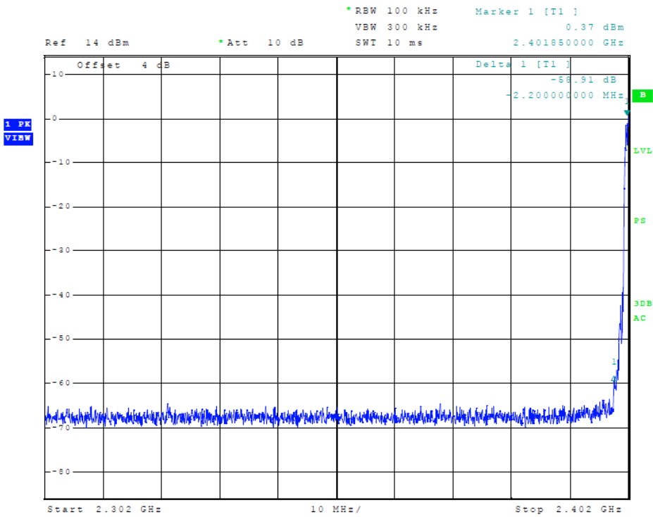
Figure 17 Plot of Transmitter Emissions (Low Band Edge, 8-DPSK)
