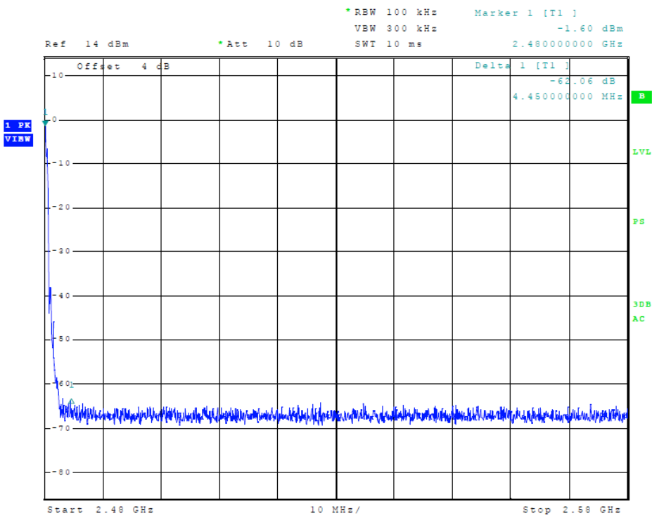
Figure 18 Plot of Transmitter Emissions (High Band Edge, 8-DPSK)
