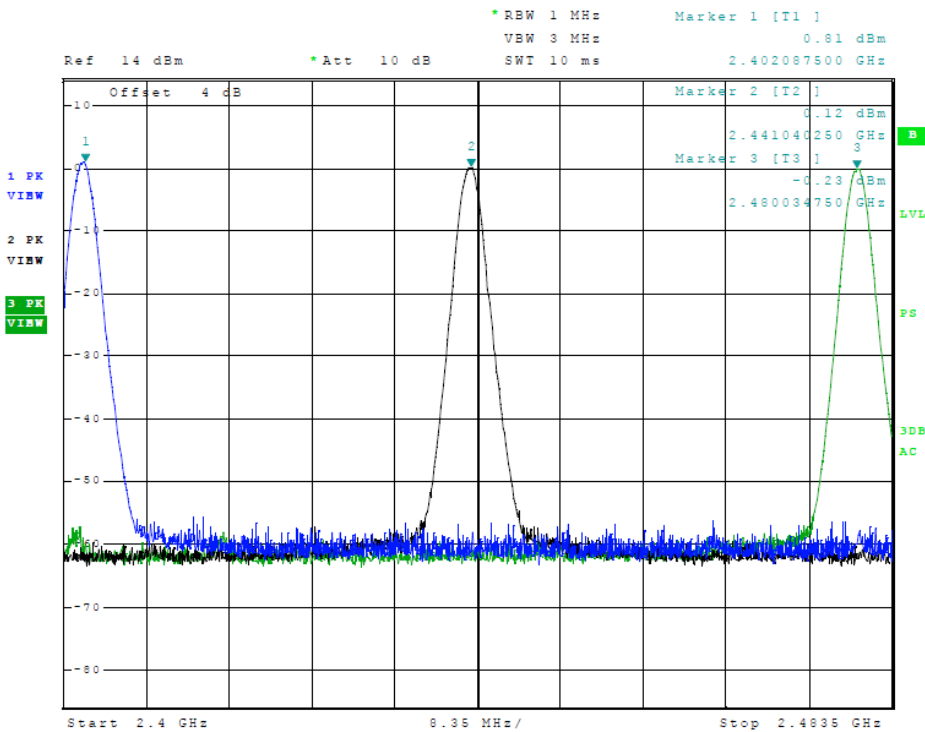
Figure 15 Plot of Transmitter Emissions (Operation in 2402-2480 MHz, 8-DPSK)
