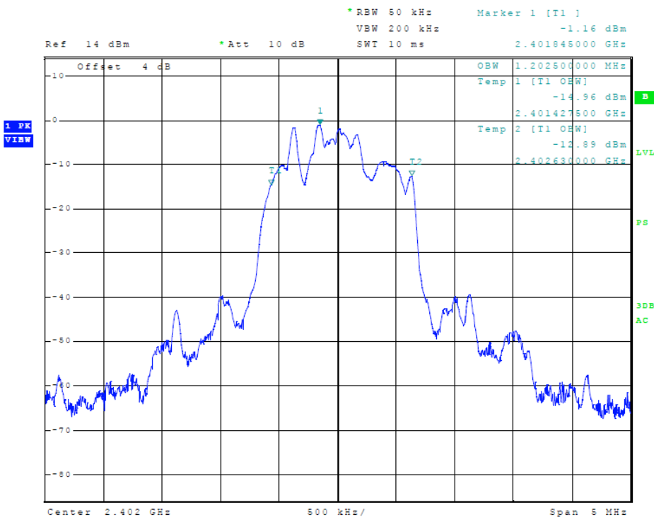
Figure 16 Plot of Transmitter Emissions (99% Occupied Bandwidth, 8-DPSK)
