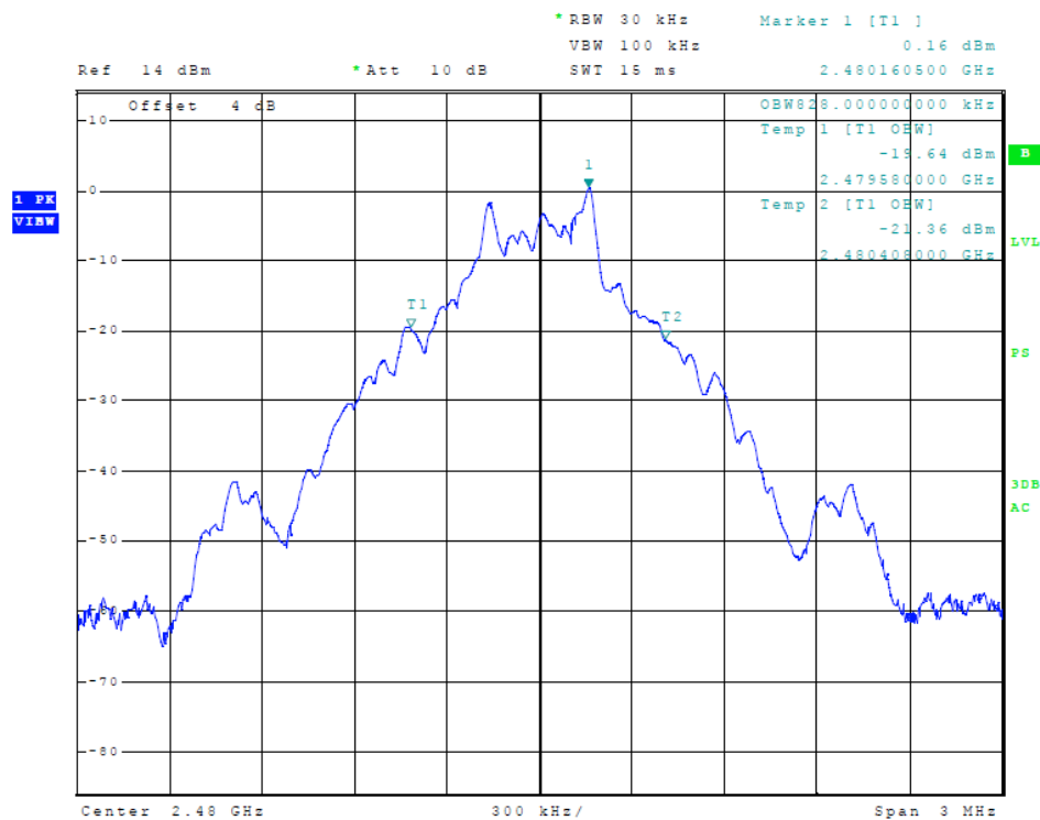
Figure 8 Plot of Transmitter Emissions (99% Occupied Bandwidth, GFSK)
