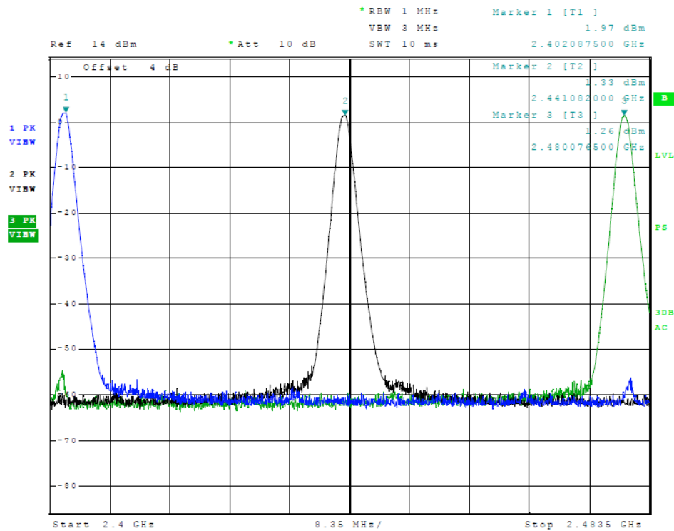
Figure 7 Plot of Transmitter Emissions (Operation in 2402-2480 MHz. GFSK)
