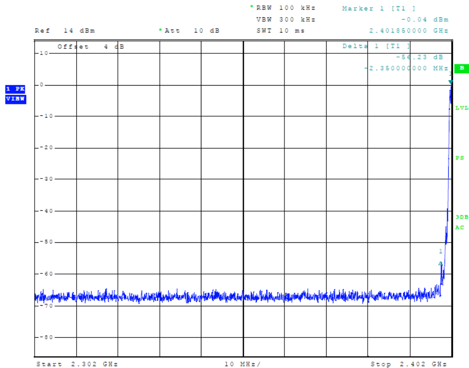
Figure 13 Plot of Transmitter Emissions (Low Band Edge, \pi/4 DQPSK)
