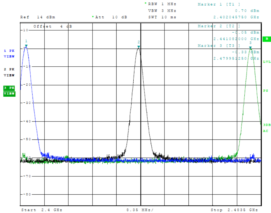
Figure 11 Plot of Transmitter Emissions (Operation in 2402-2480 MHz, \pi/4 DQPSK)
