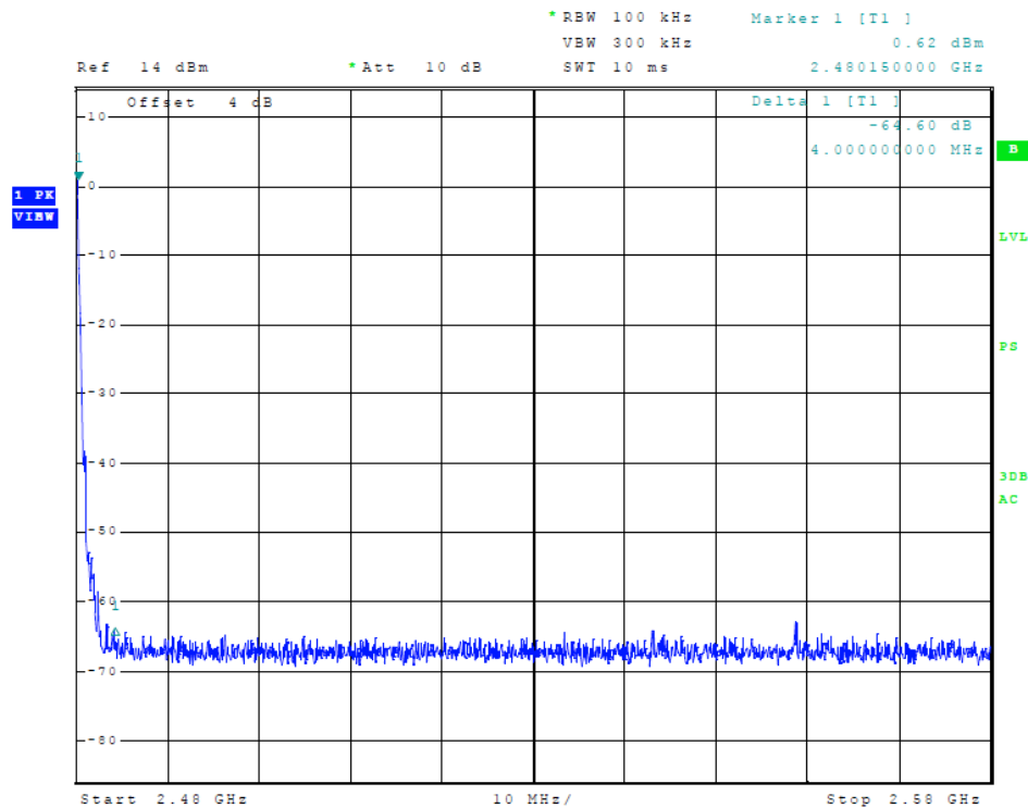
Figure 10 Plot of Transmitter Emissions (High Band Edge, GFSK)
