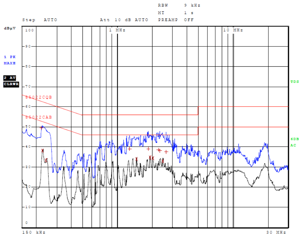
Figure 6 AC Line Conducted emissions of EUT line 2 (#6, EUT, USB CPU Adapter)
