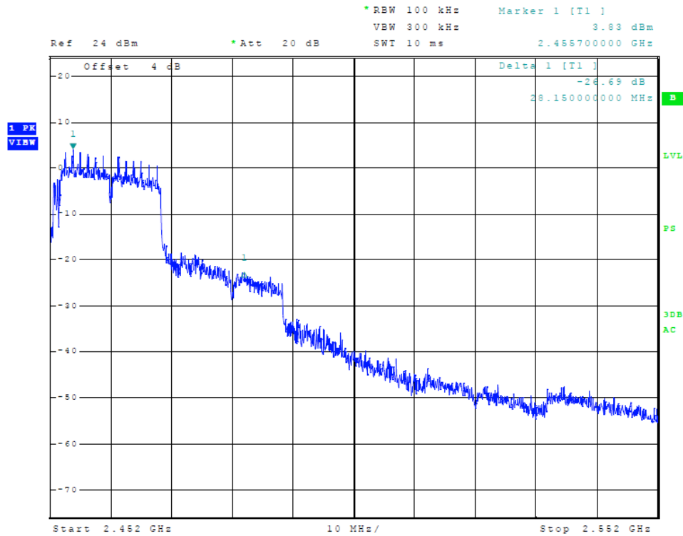
Figure 15 Plot of Upper Band Edge (802.11 n40-mode)
