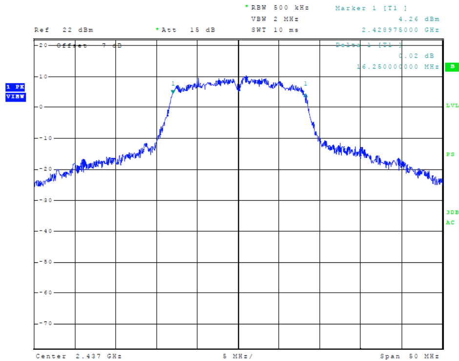
Figure 17 Plot of Transmitter 6-dB Occupied Bandwidth (802.11 g-mode)
