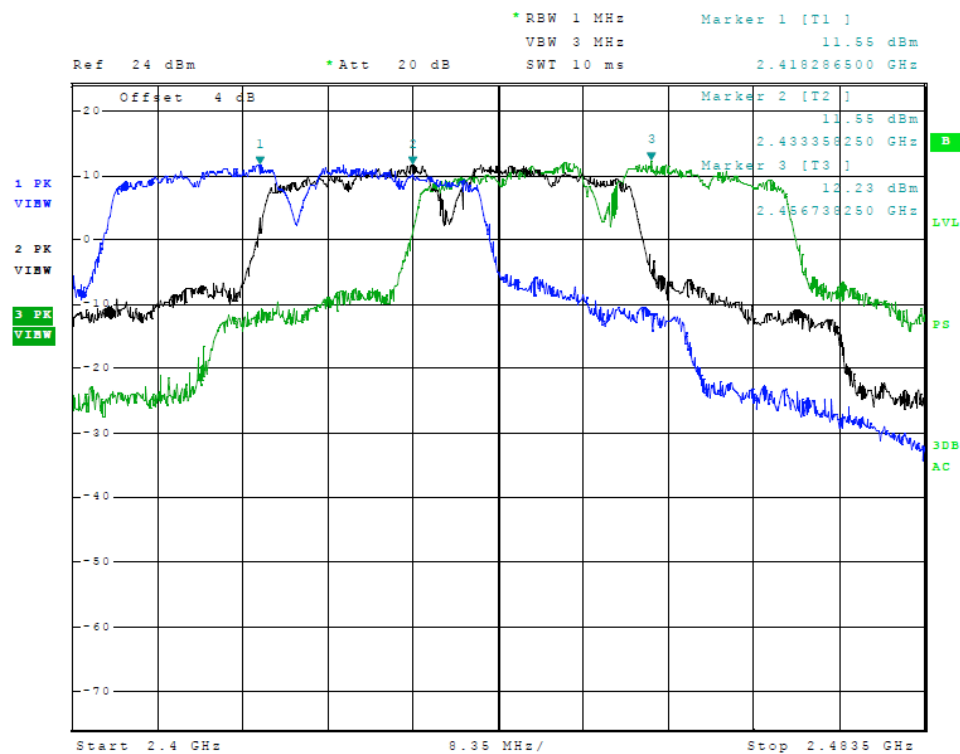
Figure 9 Plot of Transmitter Emissions in Operational Frequency (802.11 n40-Mode)
