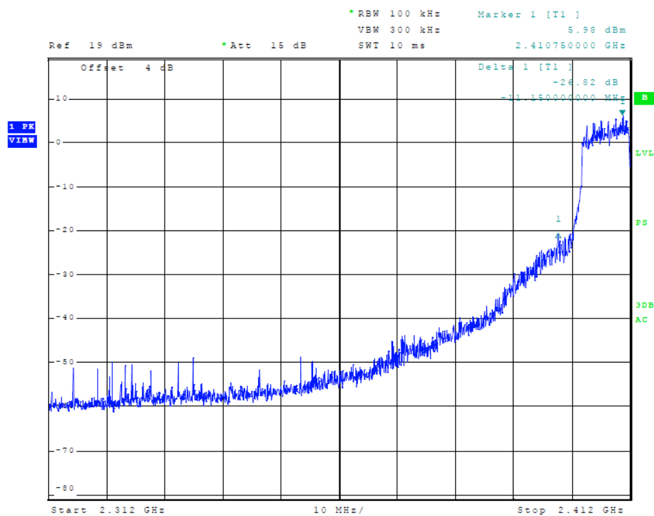
Figure 11 Plot of Lower Band Edge (802.11 g-mode)
