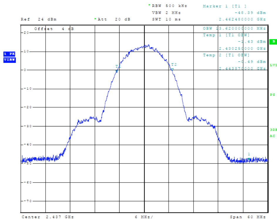
Figure 19 Plot of Transmitter 99% Occupied Bandwidth (802.11 b-mode)
