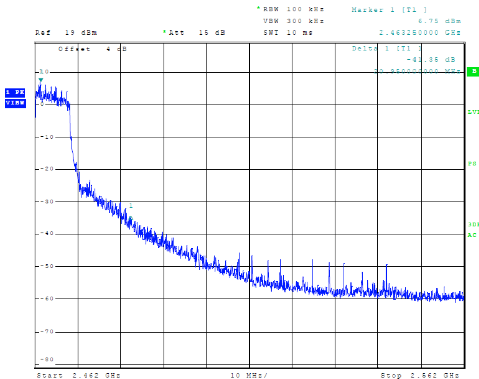
Figure 14 Plot of Upper Band Edge (802.11 g-mode)
