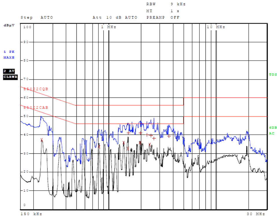
Figure 5 AC Line Conducted emissions of EUT line 1 (#6, EUT, USB CPU Adapter)
