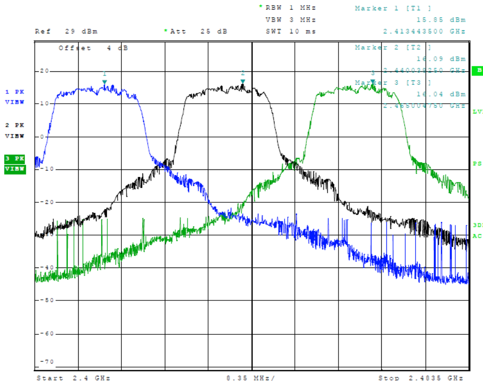
Figure 8 Plot of Transmitter Emissions in Operational Frequency (802.11 g-Mode)
