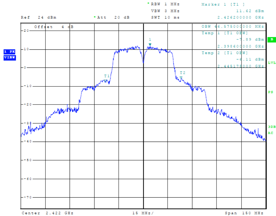
Figure 21 Plot of Transmitter 99% Occupied Bandwidth (802.11 n40-mode)
