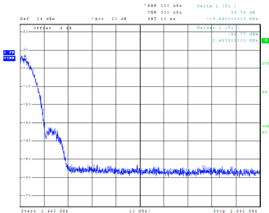
Figure 13 Plot of Upper Band Edge (802.11 b-mode)
