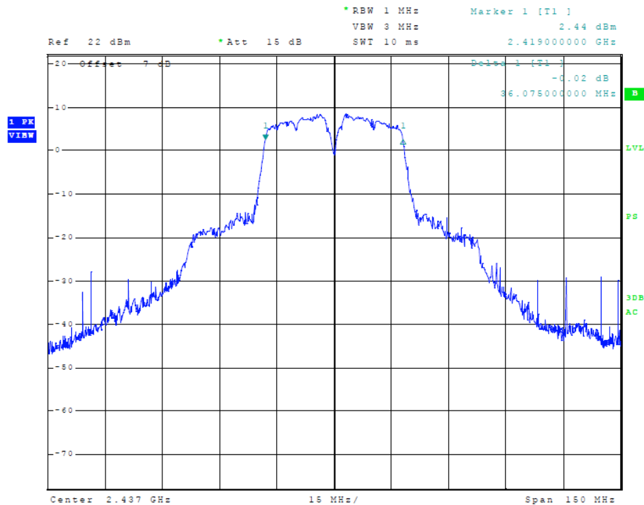
Figure 18 Plot of Transmitter 6-dB Occupied Bandwidth (802.11 n40-mode)
