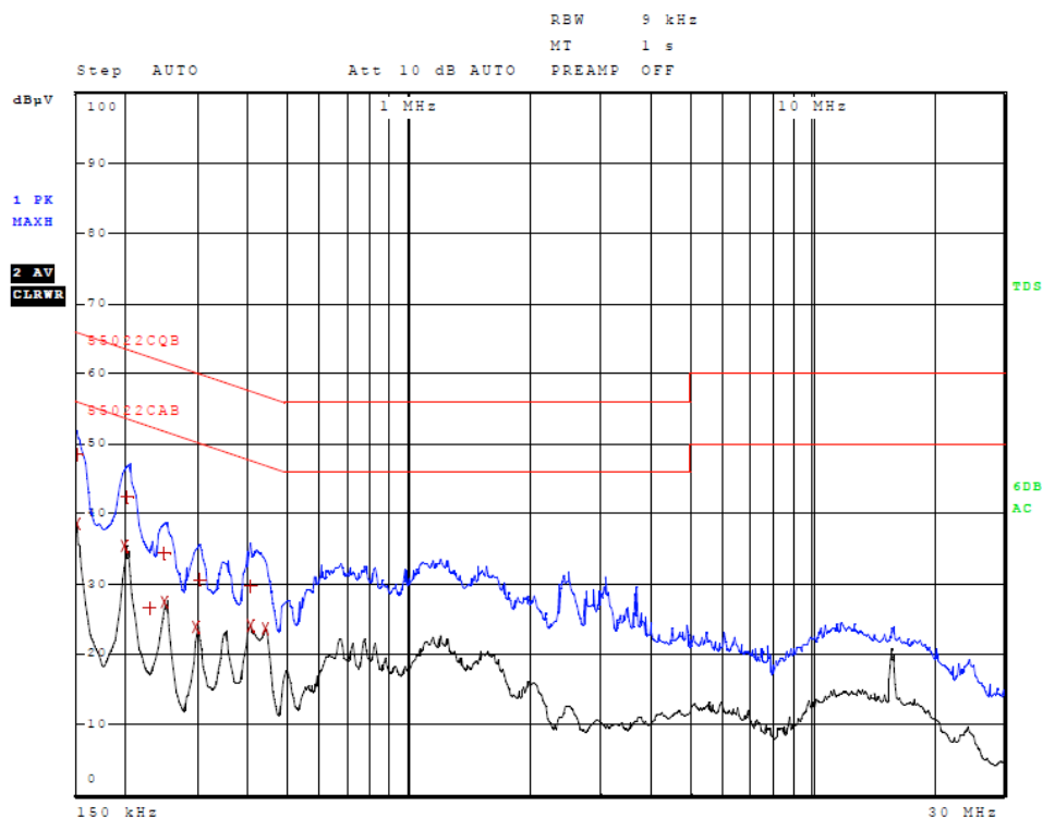
Figure 3 AC Line Conducted emissions of EUT line 1 (#2, EUT, 86 Adapter)
