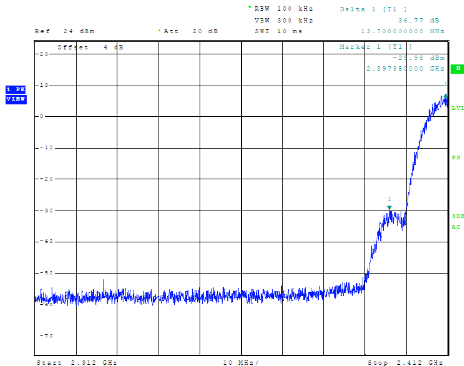
Figure 10 Plot of Lower Band Edge (802.11 b-mode)
