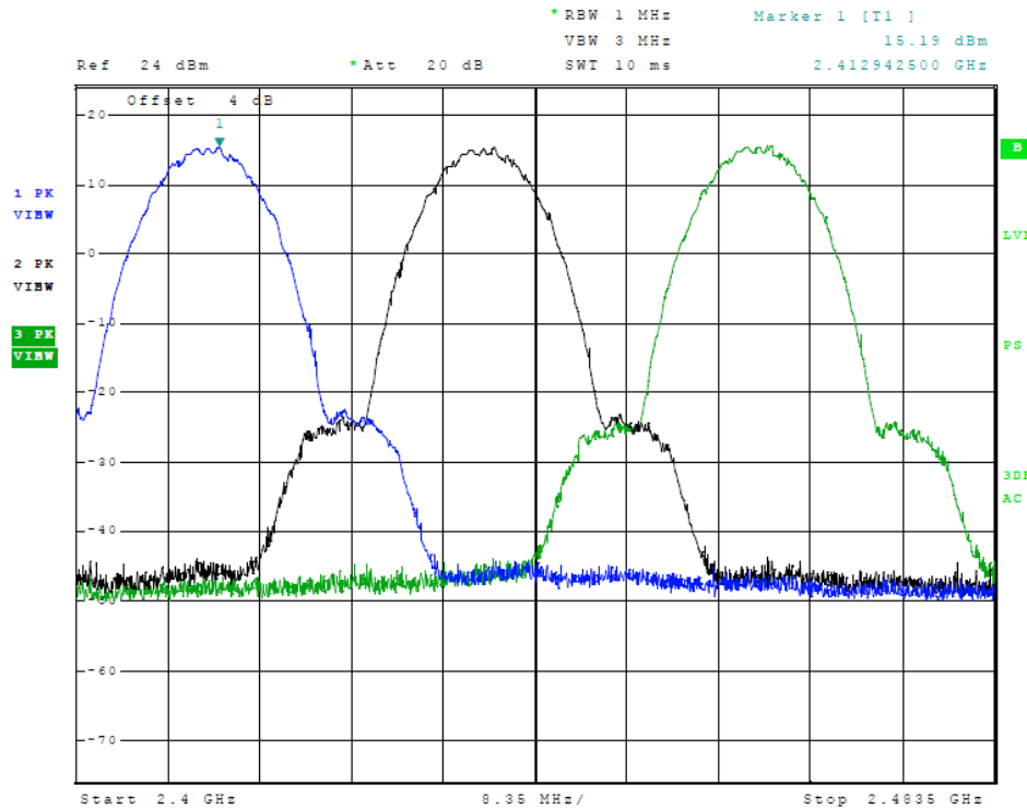
Figure 7 Plot of Transmitter Emissions in Operational Frequency (802.11 b-Mode)
