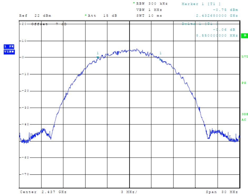
Figure 16 Plot of Transmitter 6-dB Occupied Bandwidth (802.11 b-mode)
