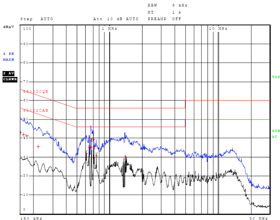
Figure 1 AC Line Conducted emissions of EUT line 1 (#2, EUT, 96 Adapter)
