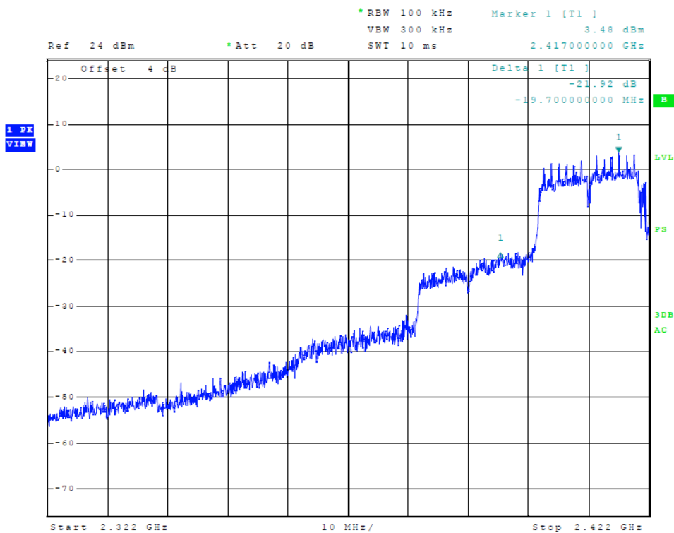
Figure 12 Plot of Lower Band Edge (802.11 n40-mode)
