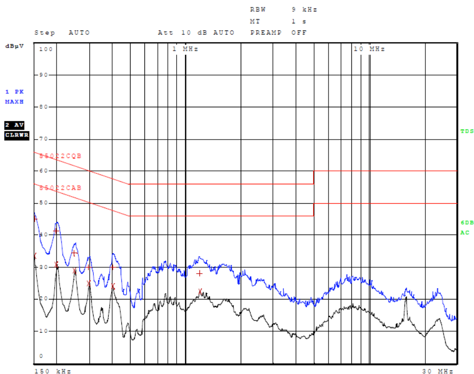
Figure 4 AC Line Conducted emissions of EUT line 2 (#2, EUT, 86 Adapter)
