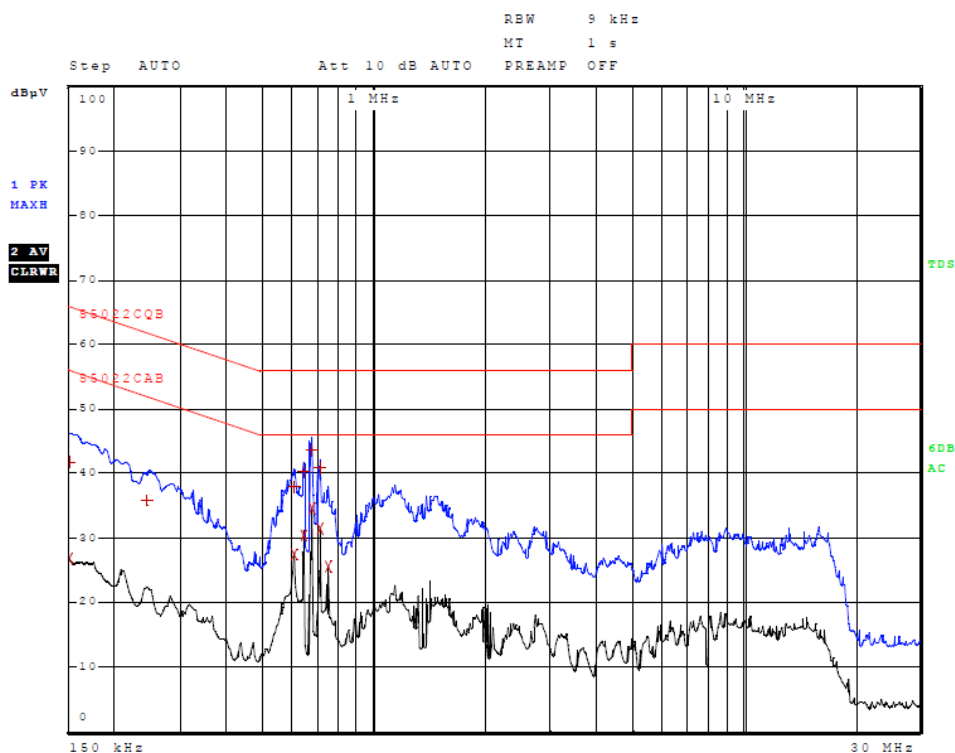
Figure 2 AC Line Conducted emissions of EUT line 2 (#2, EUT, 96 Adapter)
