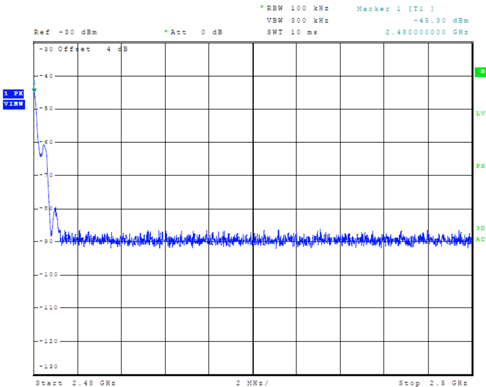
Figure 14 Plot of Transmitter Emissions (High Band Edge)
