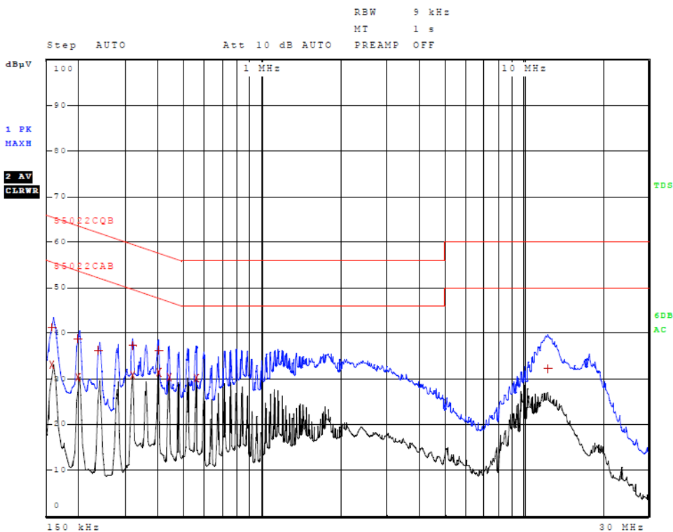
Figure 2 AC Line Conducted emissions of EUT line 2 (EUT AC Adapter, 362-00072-00)
