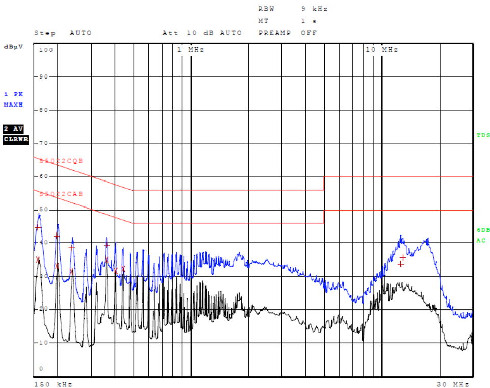
Figure 1 AC Line Conducted emissions of EUT line 1 (EUT AC Adapter, 362-00072-00)
