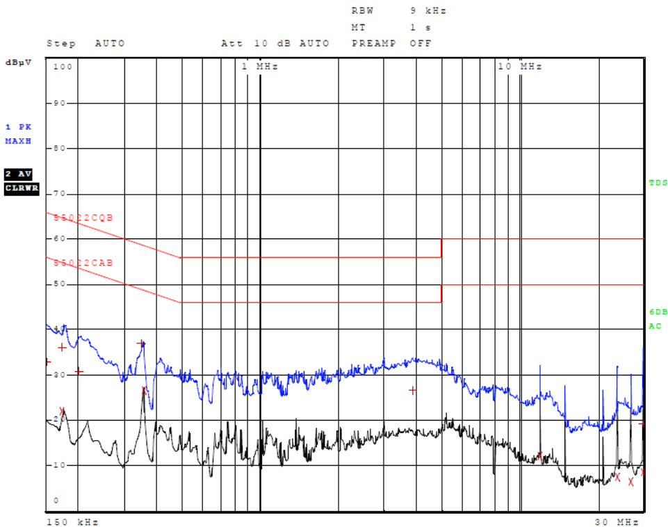
Figure 4 AC Line Conducted emissions of EUT line 2 (EUT AC Adapter, SCB0500600P)
