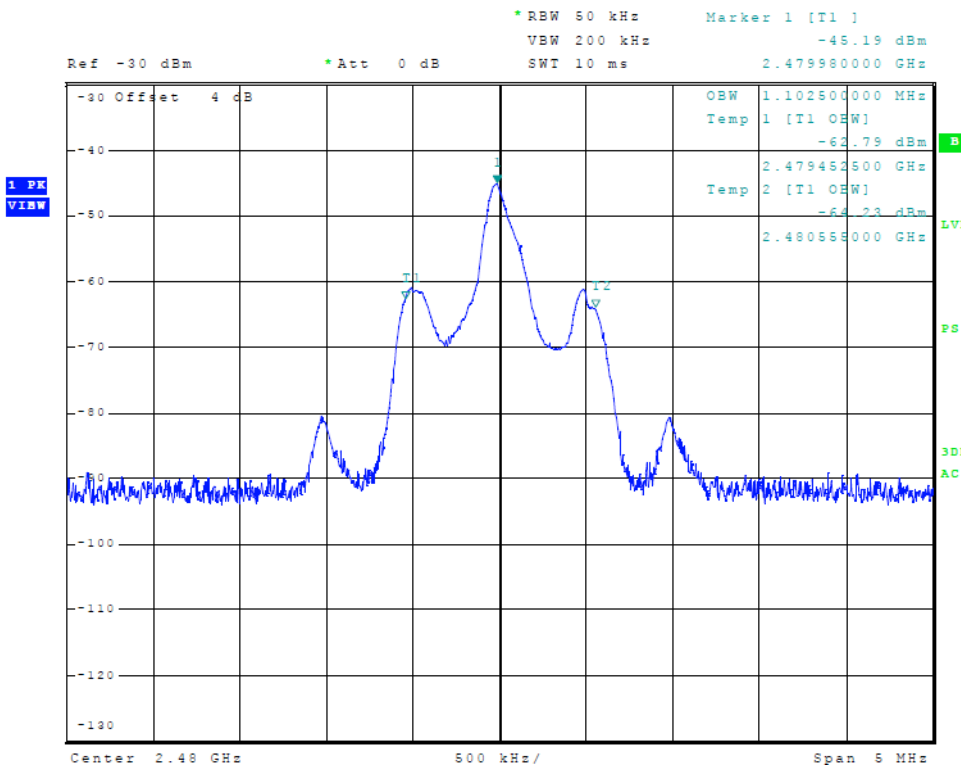
Figure 12 Plot of Transmitter Emissions (2402-2480 MHz, 99% Occupied Bandwidth)
