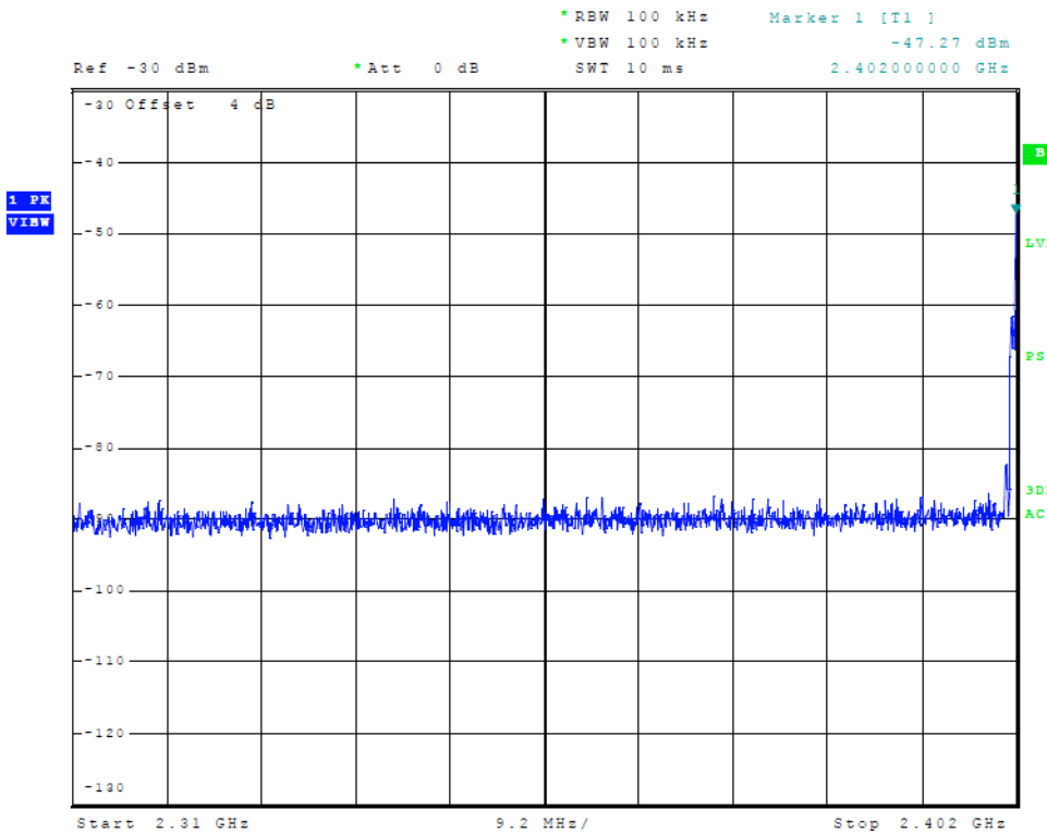
Figure 13 Plot of Transmitter Emissions (Low Band Edge)
