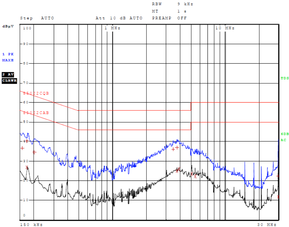
Figure 3 AC Line Conducted emissions of EUT line 1 (EUT AC Adapter, SCB0500600P)
