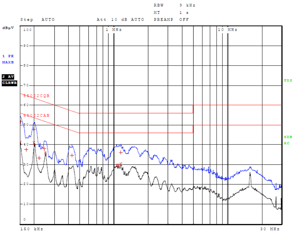
Figure 7 AC Line Conducted emissions of EUT line 1 (EUT AC Adapter, 362-00086-01)
