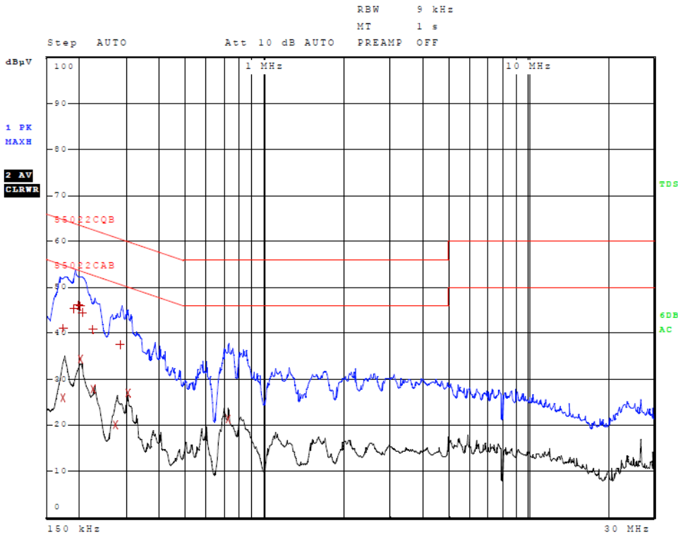
Figure 5 AC Line Conducted emissions of EUT line 1 (EUT AC Adapter, 362-00087-00)
