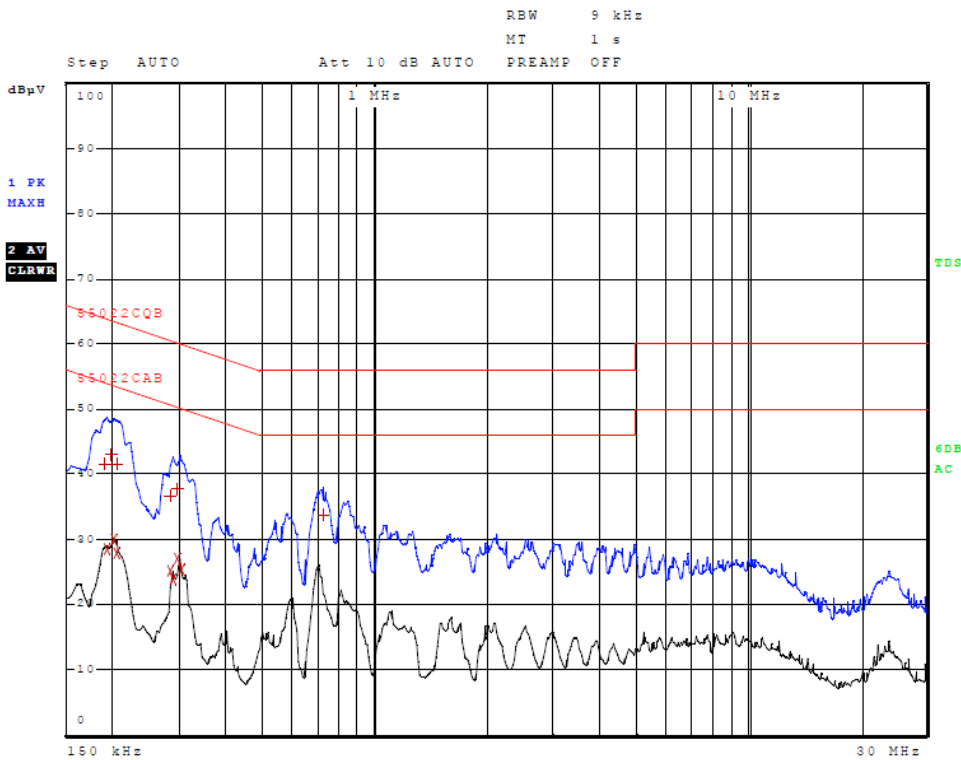
Figure 6 AC Line Conducted emissions of EUT line 2 (EUT AC Adapter, 362-00087-00)
