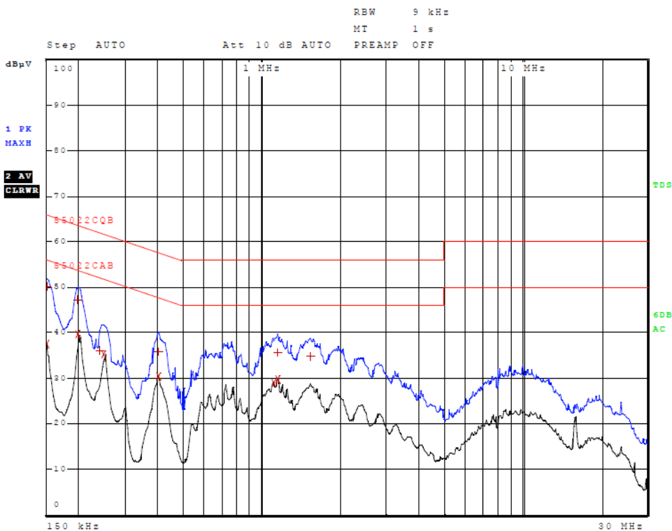
Figure 8 AC Line Conducted emissions of EUT line 2 (EUT AC Adapter, 362-00086-01)
