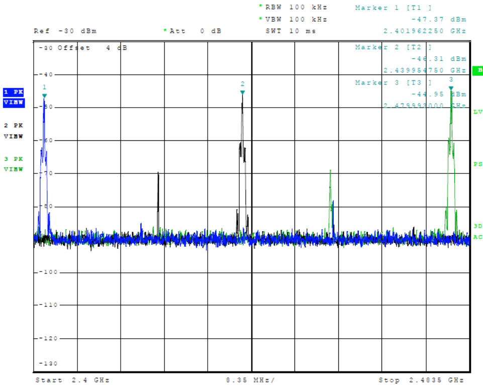
Figure 11 Plot of Transmitter Emissions (In 2402-2480 MHz Band)
