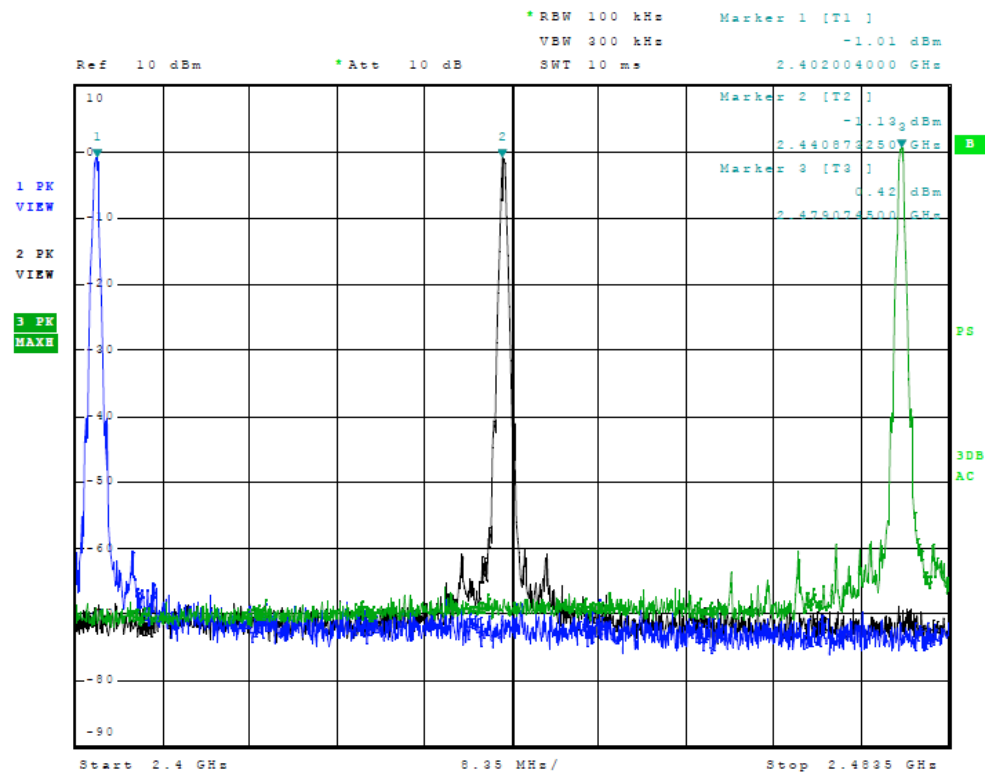
Figure 5 Plot of Transmitter Emissions (In Band 2402-2480 MHz Operation)
