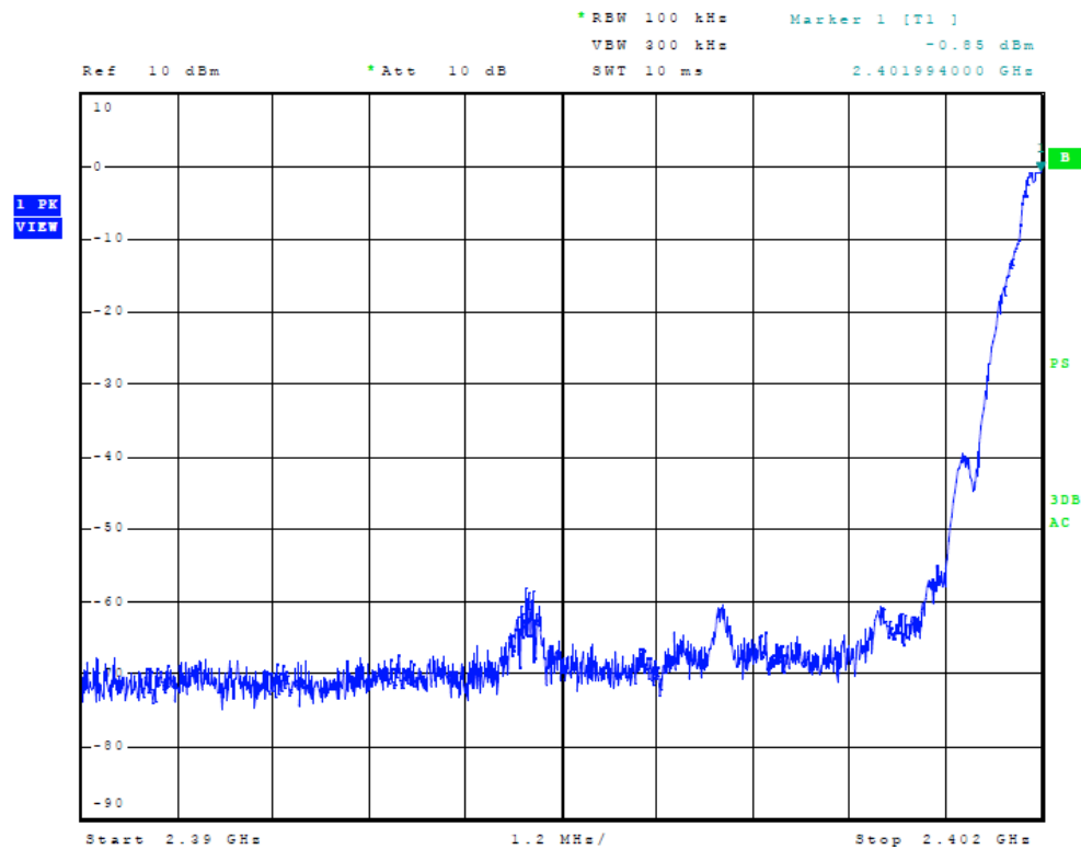
Figure 7 Plot of Transmitter Emissions (Low Band Edge 2402-2480 MHz)
