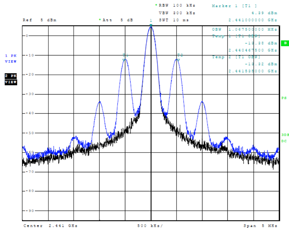
Figure 6 Plot of Transmitter Emissions (99% 2402-2480 MHz Occupied Bandwidth)
