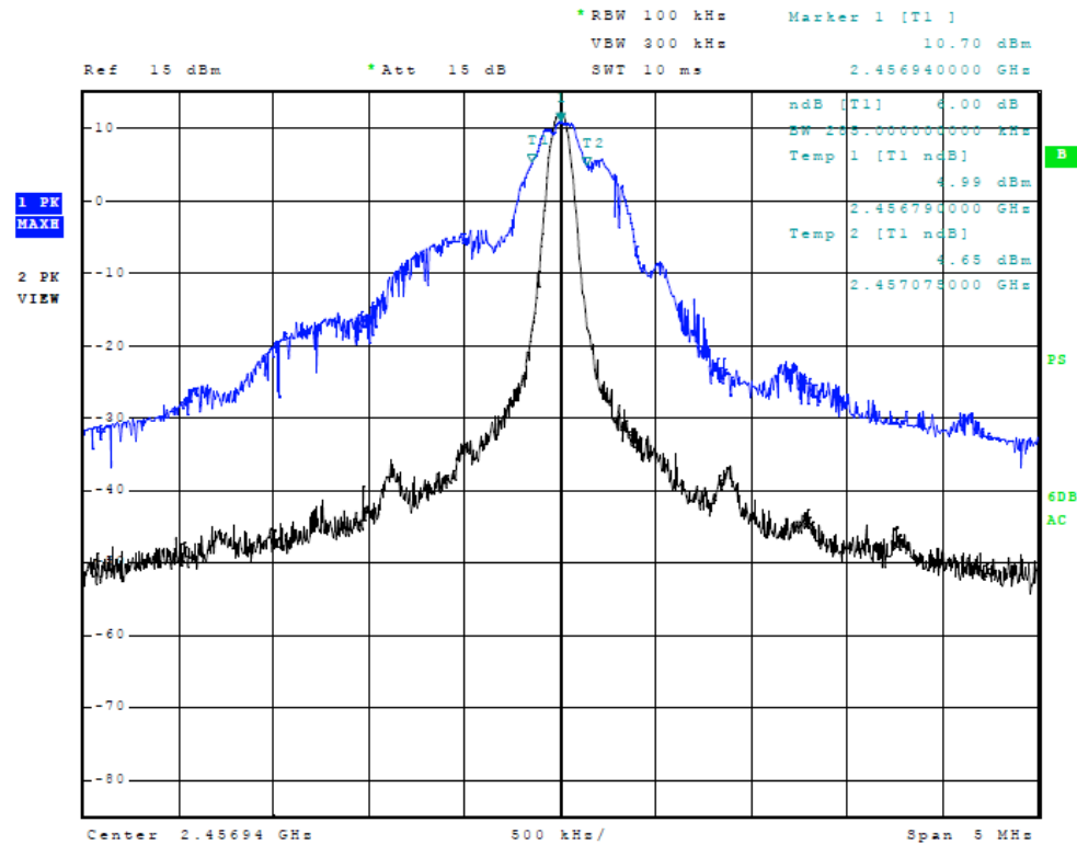
Figure 1 Plot of Occupied Bandwidth
