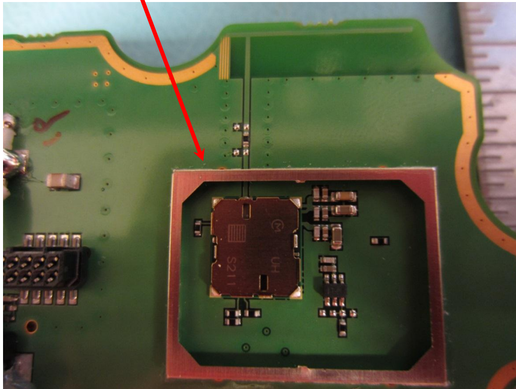
Transmitter Section
