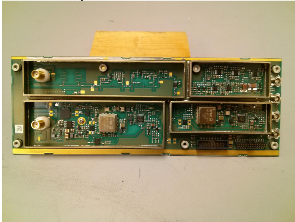
Internal Photographs RF section of PCB top
