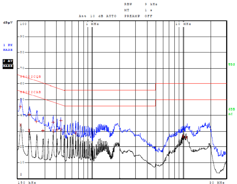
Figure Four AC Line Conducted emissions of EUT line 2 (EUT AC Adapter)
