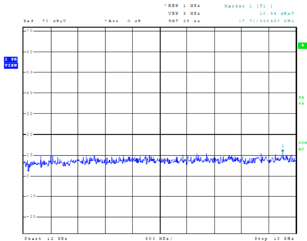
Figure Ten General Radiated Emissions in screen room
