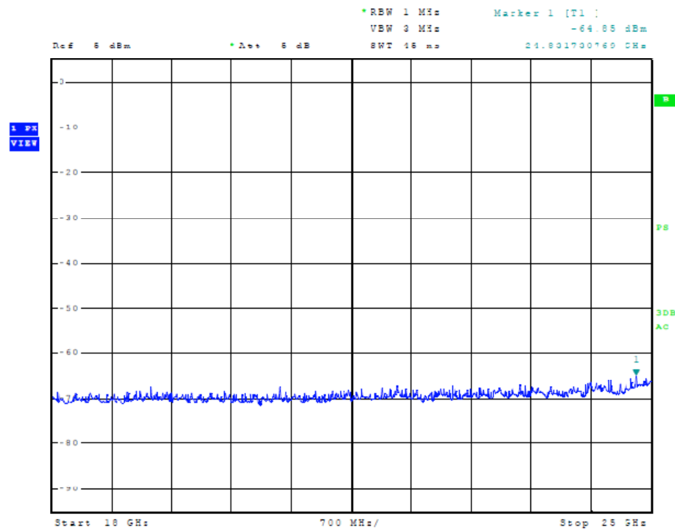
Figure Twenty-three output measured at temporary antenna terminal
