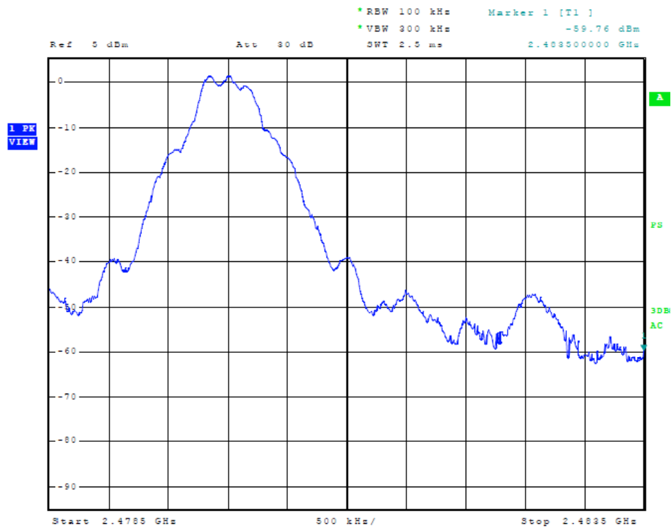
Figure Twenty-nine High Frequency Band Edge
