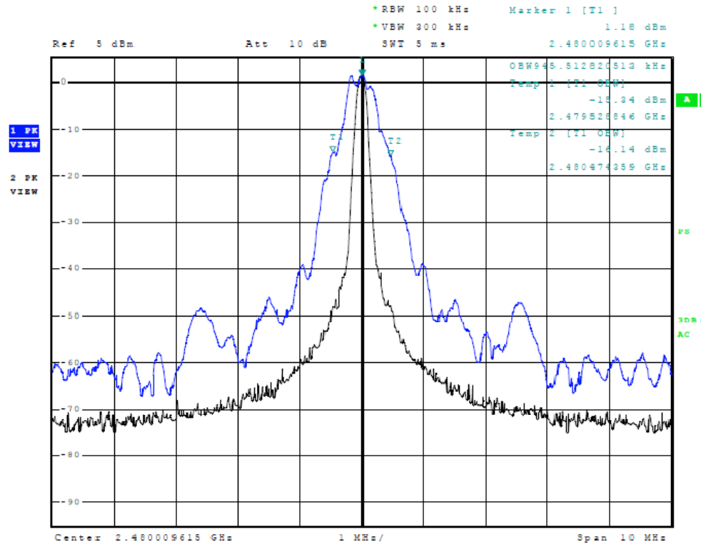
Figure Twenty-six Occupied Bandwidth (high channel)
