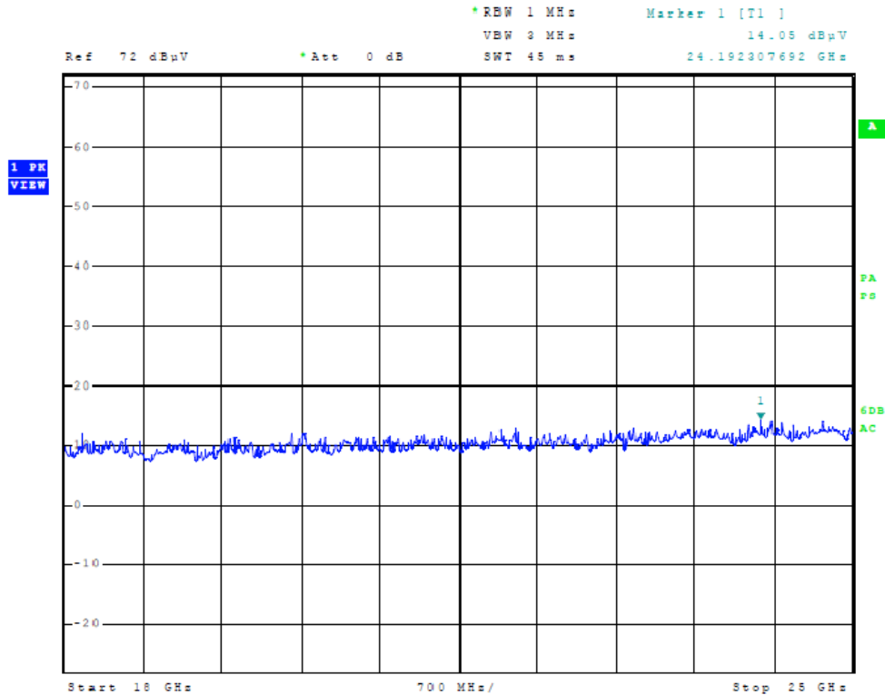
Figure Eleven General Radiated Emissions in screen room
