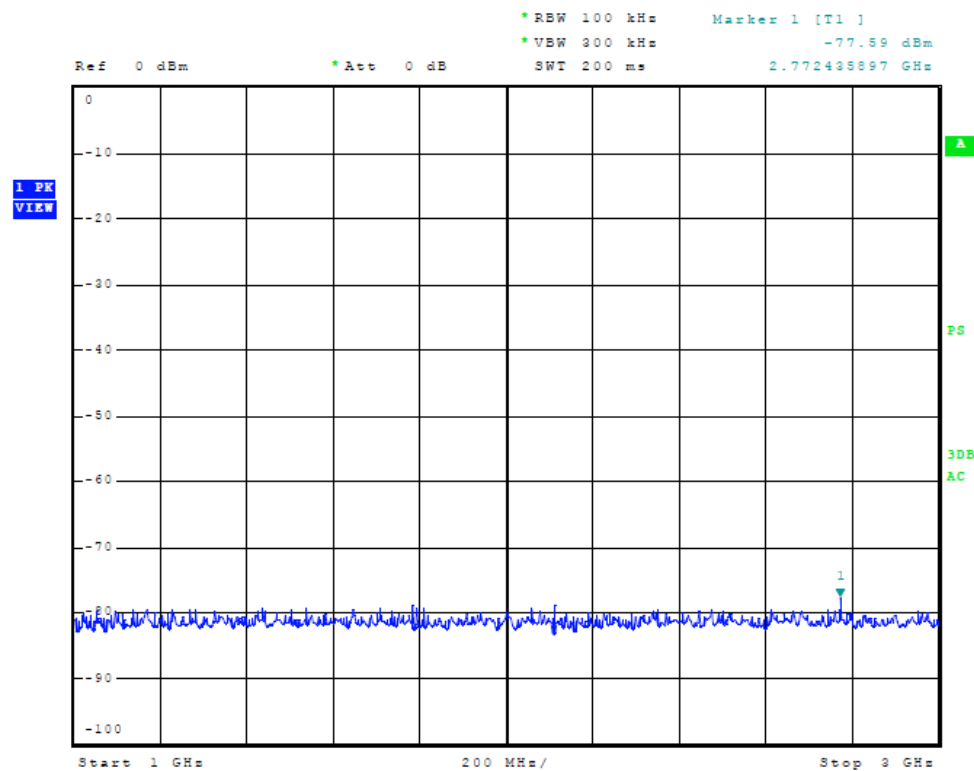
Figure Thirteen Receiver Temporary Antenna Port Conducted Emissions
