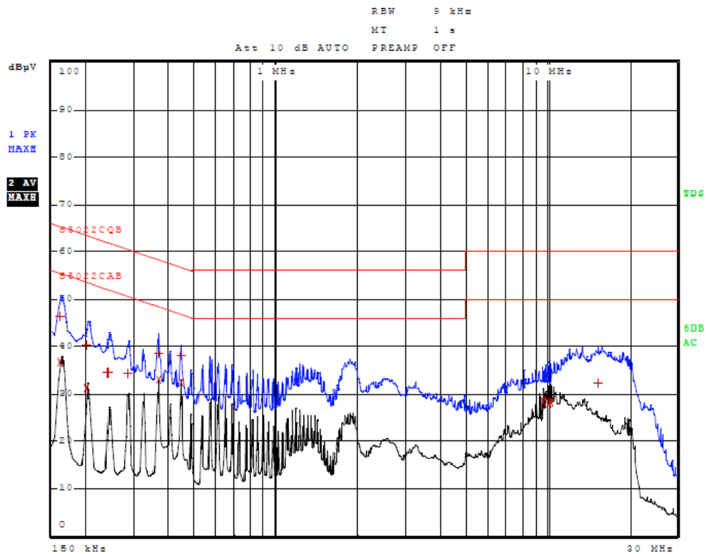
Figure Three AC Line Conducted emissions of EUT line 1 (EUT AC Adapter)
