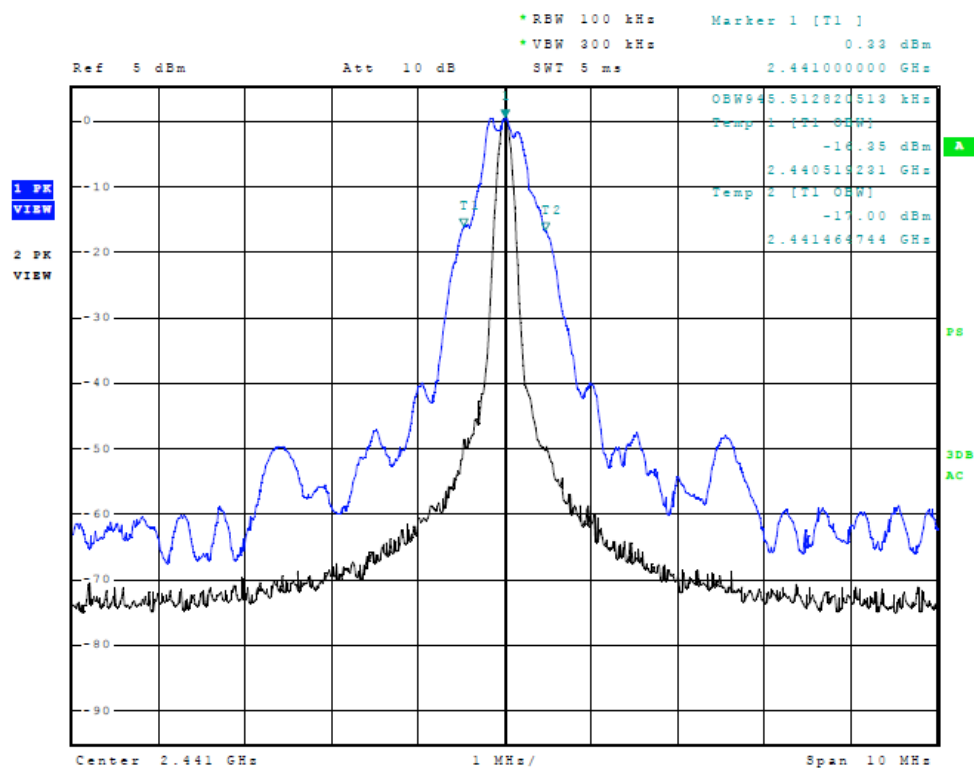
Figure Twenty-five Occupied Bandwidth (middle channel)
