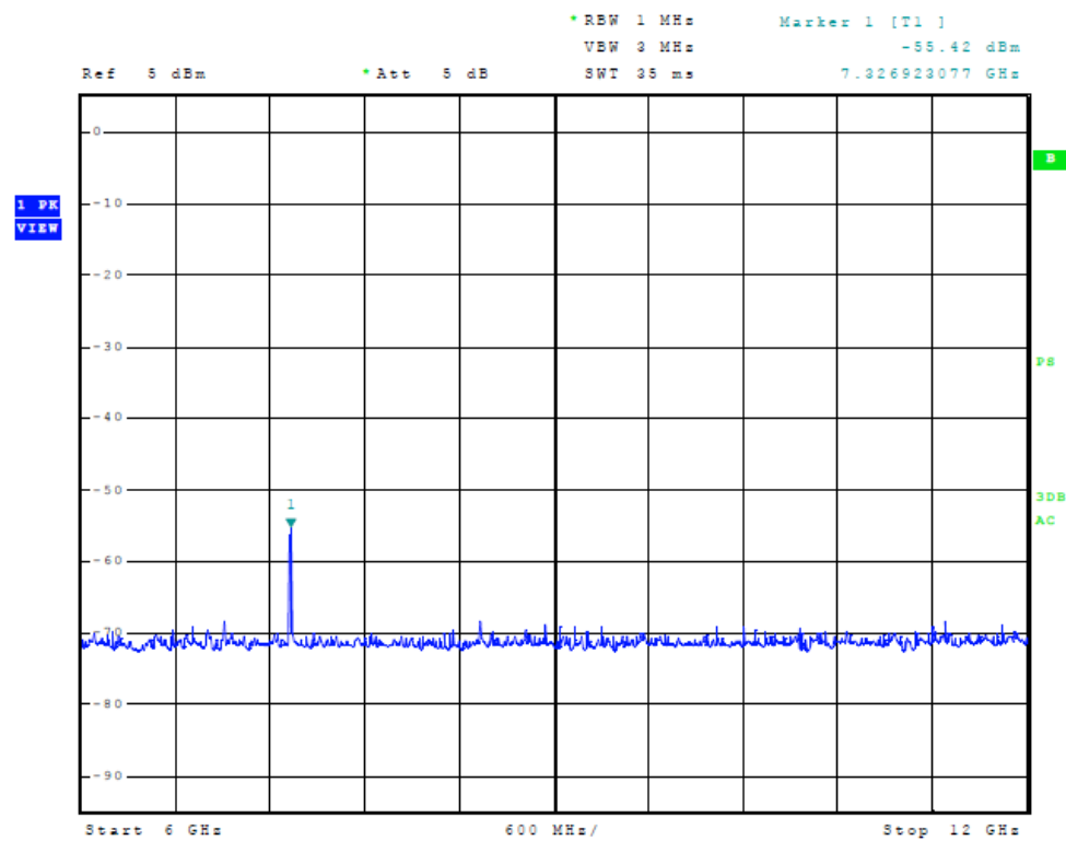
Figure Twenty-one output measured at temporary antenna terminal
