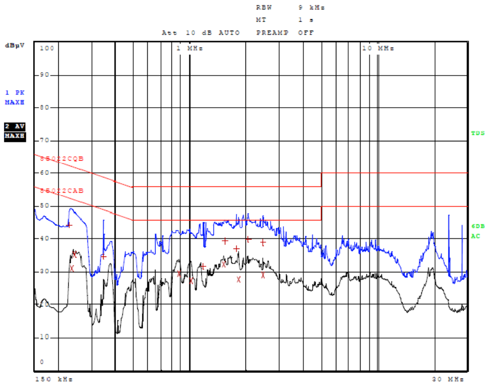
Figure Two AC Line Conducted emissions of EUT line 2 (EUT USB CPU AC Adapter)
