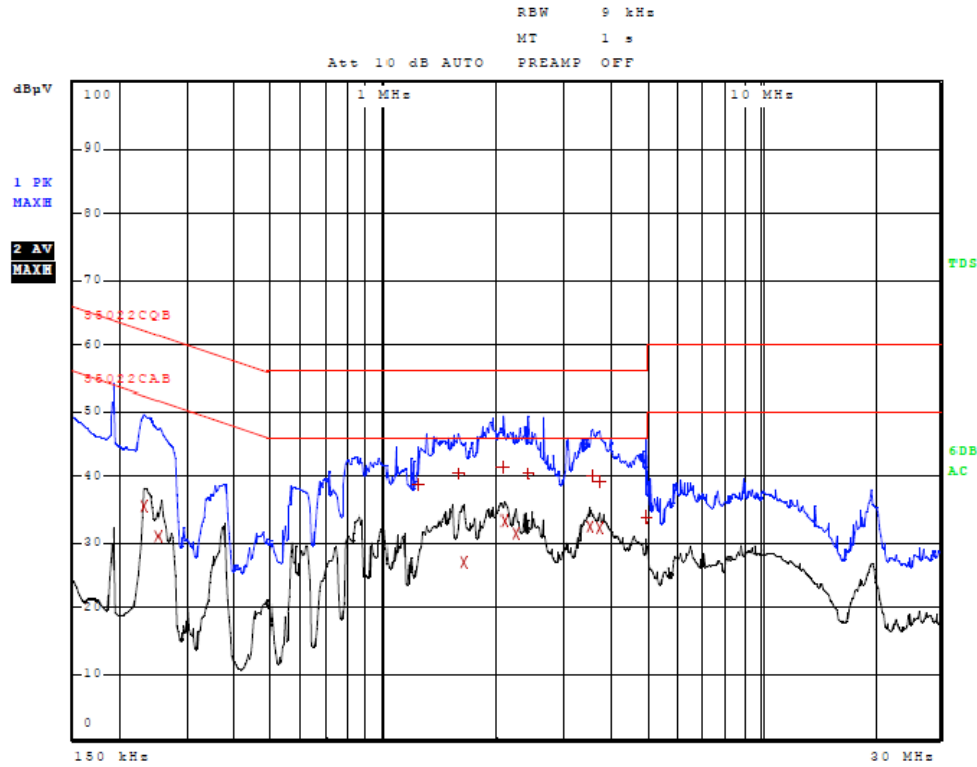
Figure One AC Line Conducted emissions of EUT line 1 (EUT USB CPU AC Adapter)
