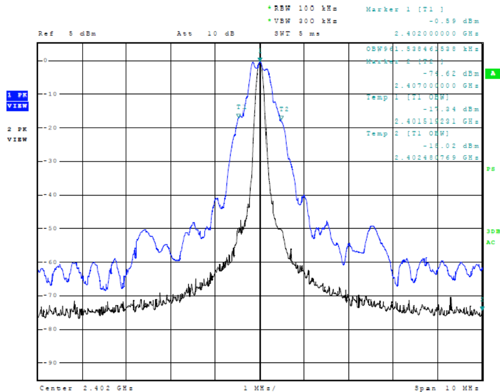
Figure Twenty-four Occupied Bandwidth (low channel)
