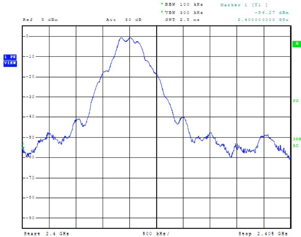
Figure Twenty-eight Low Frequency Band Edge
