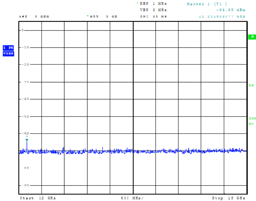
Figure Twenty-two output measured at temporary antenna terminal
