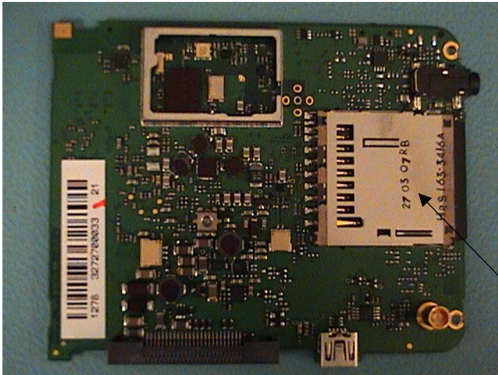
Printed Circuit Bottom with GPS Antenna and covers removed (FM/BT)
