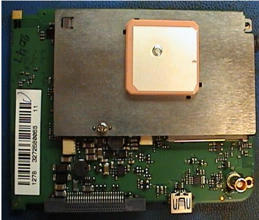
Printed Circuit Bottom with GPS Antenna in place
