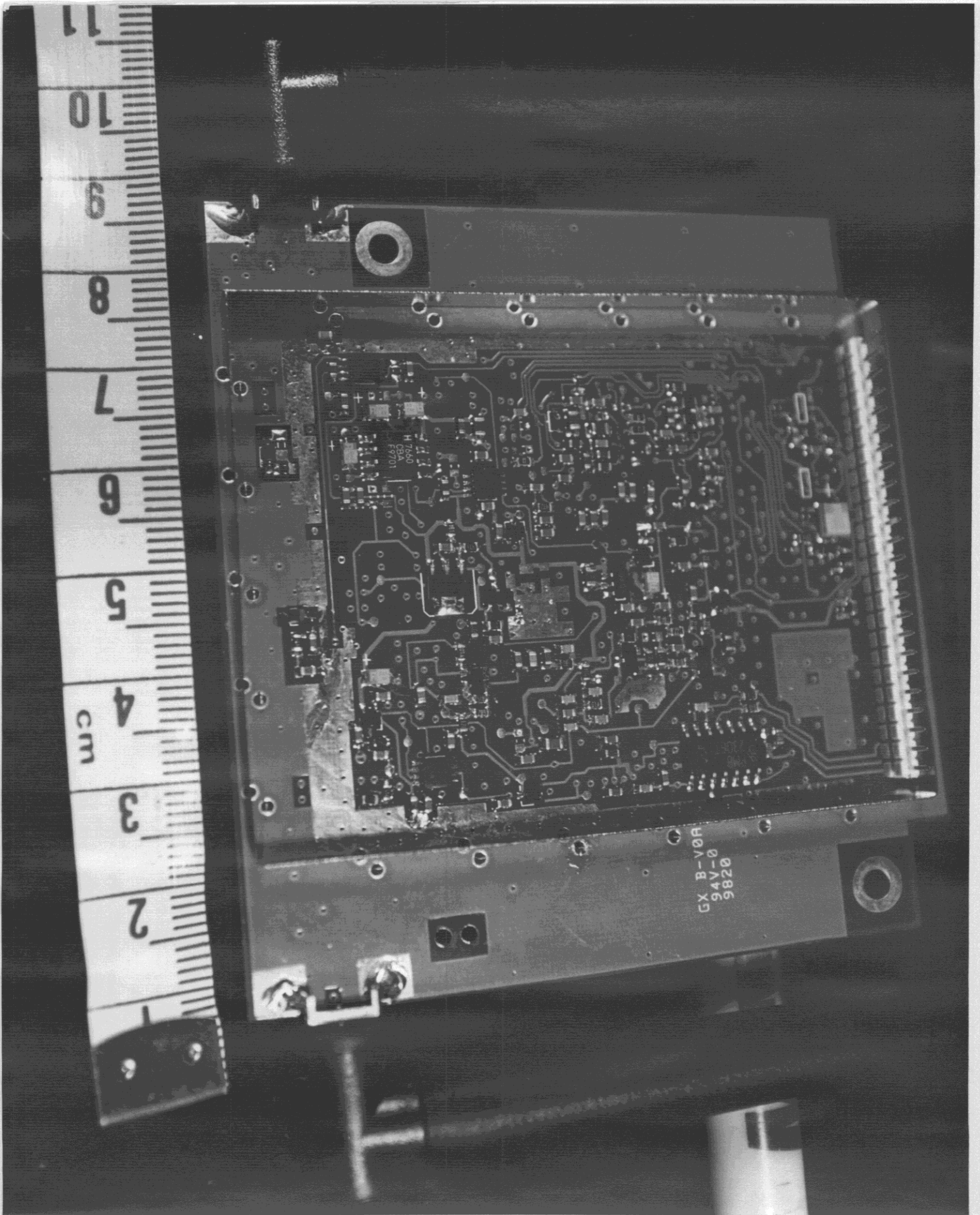
Back Side View of RF Module-2
