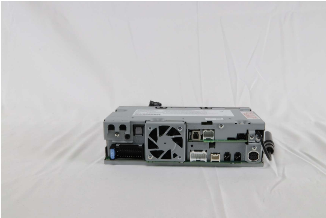
Picture10 : Rear(Body)
